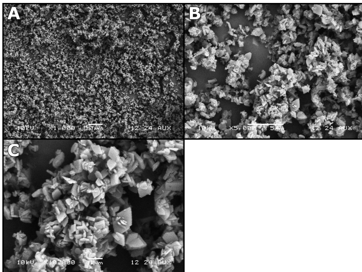
SEM micrographs of Boehmite from C31C 300°C 4hr 3-26-07 blend 2,9,10. Average particle size of 0.67 µm.
