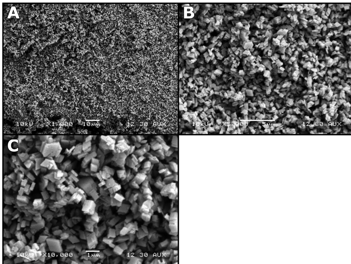
SEM micrographs of APYRAL AOH 60. Average particle size of 0.69 \mu\text{m} .
