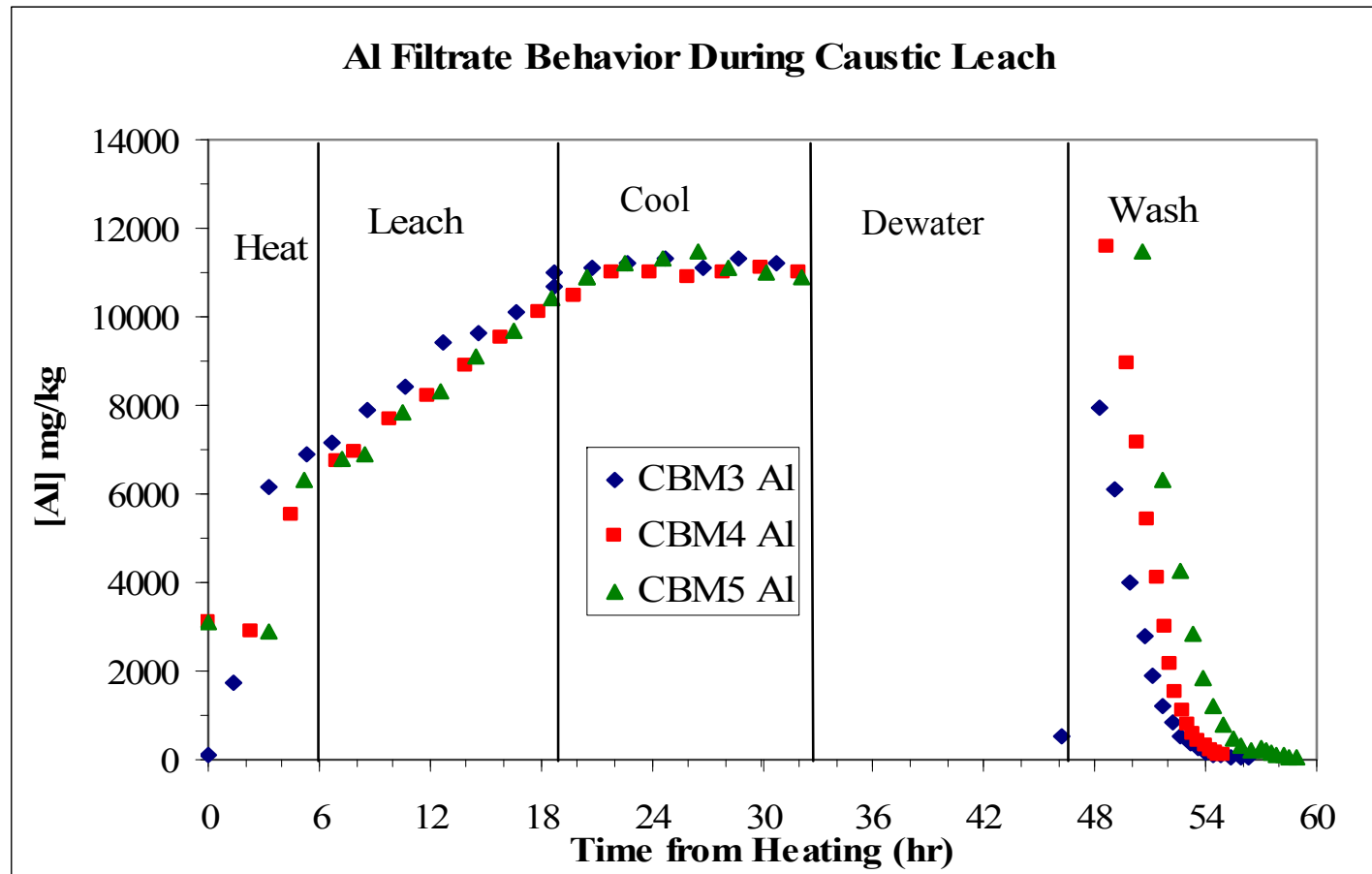
Figure 6.11. Dissolution of Aluminum in mg/kg Solution in Tests CBM-3, CBM-4, and CBM-5
