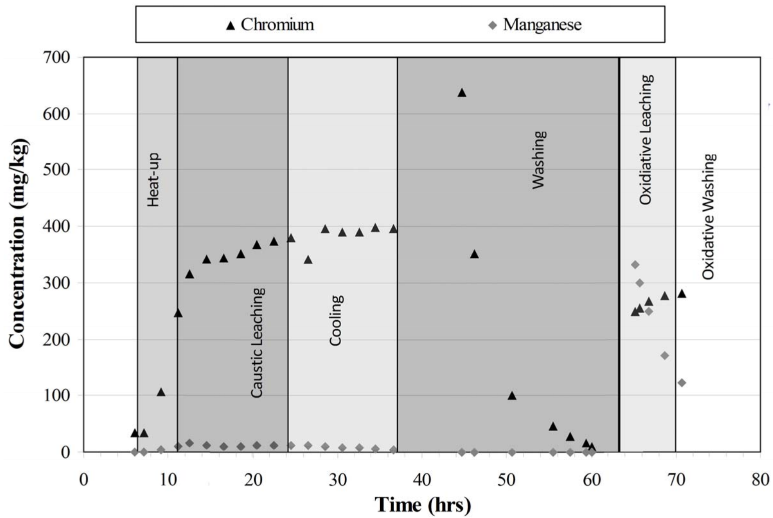
Figure 6.2. Dissolution of Chromium and Manganese in mg/kg solution in Test CBM-1
