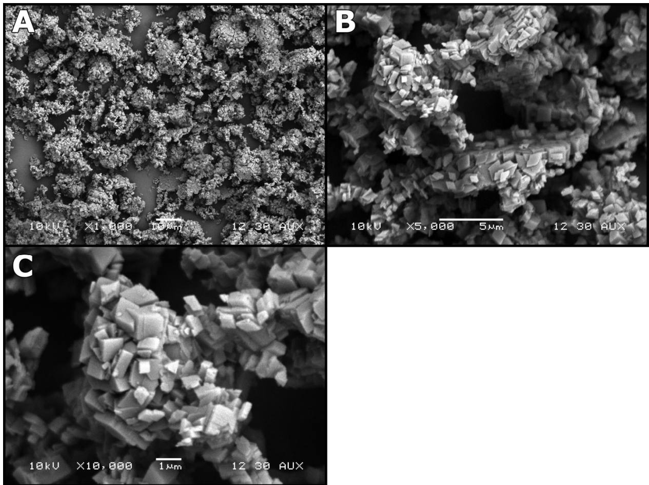
SEM micrographs of B2 APYRAL AOH 20Y. Average particle size of 0.72 \mu\text{m} .
