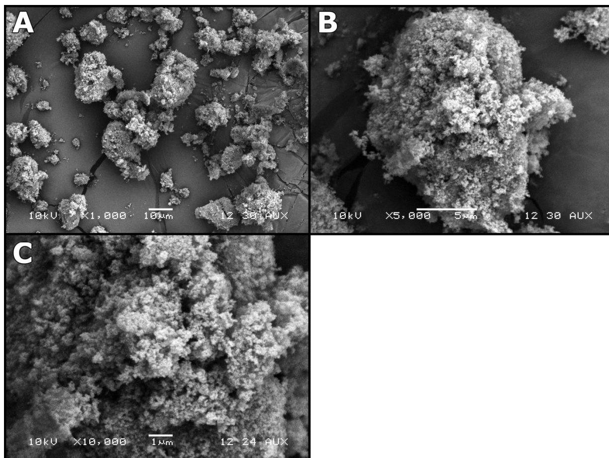
Figure 2.11. SEM Picture of Boehmite Sample B4 at 1,000×, 5,000×, and 10,000×
