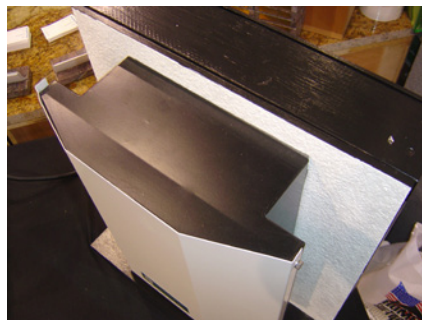
Figure 21.1. This exhaust fan and electronic controls are designed to ventilate—and could be used to create a slightly negative pressure in—the garage. Ventilation carries pollutants to the outside, negative pressure helps to stop garage air from migrating into attached houses.
