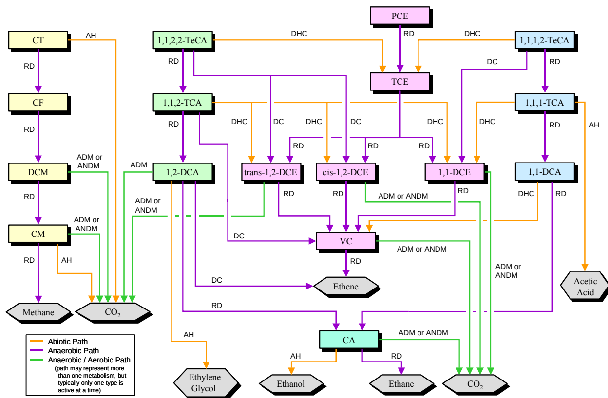
Figure 5. Conceptual Model for Dechlorination Reactions in the Mixed Chloroethene/Chloroethane/Chloromethane Dechlorination Reaction Module — Species in hexagonal shaded boxes are innocuous products and are not tracked in the reaction module. The reaction types for each pathway are described in Table 3.
