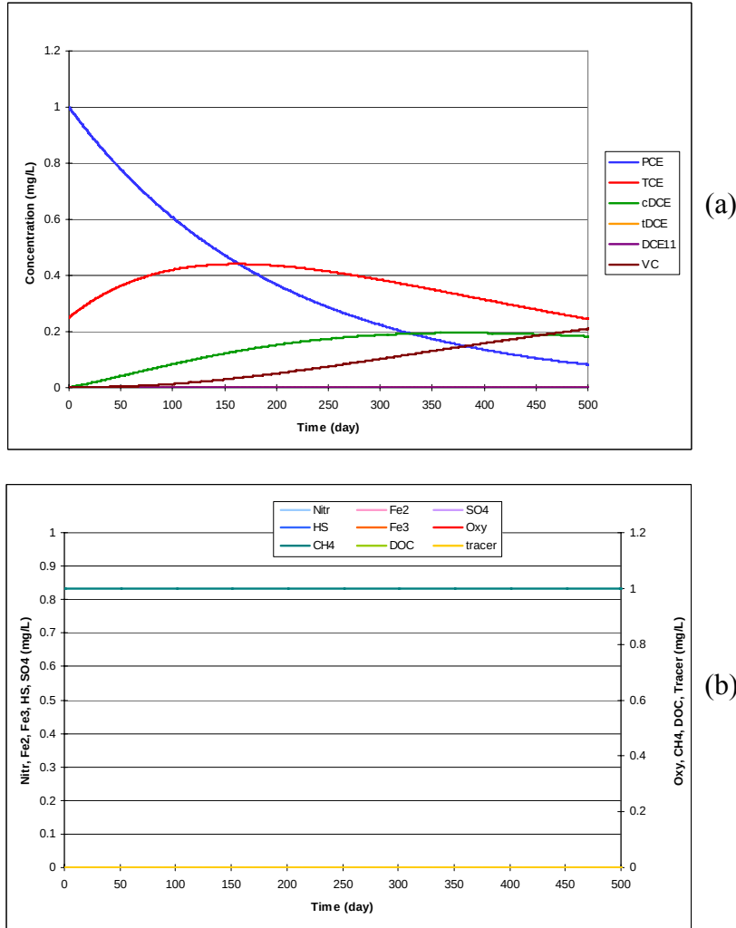
Figure 32. Example Simulation 1: Dechlorination of PCE and TCE Using the Parameter Values Shown in Table 39 — The initial concentration for PCE, TCE, and methane were 1, 0.25, and 1 mg/L, respectively. All other species concentrations started at zero. Note that the concentrations of redox species remain constant in this simulation. Figure (a) shows chlorinated solvent concentration. Figure (b) shows the concentration of other species.
