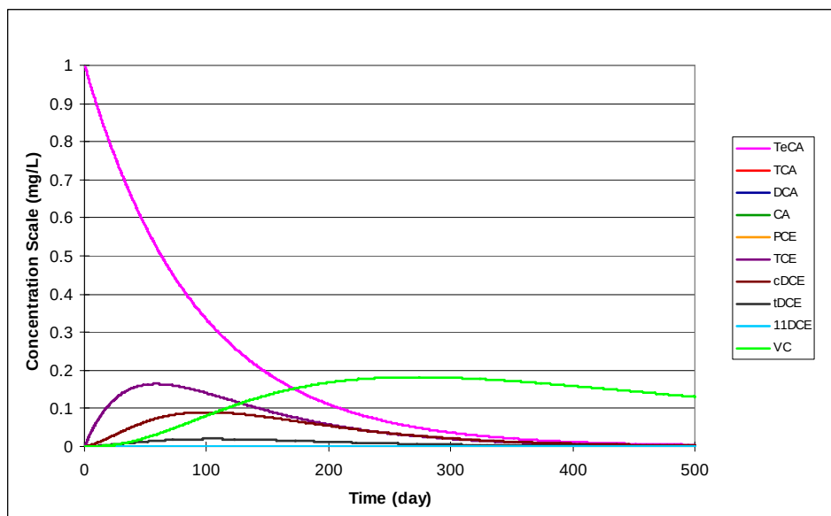
Figure 16. Dechlorination of 1,1,2,2-TeCA Using the Parameter Values Shown in Table 20 — The initial concentration for TeCA was 1 mg/L. All other species concentrations started at zero. In the results, the concentrations of TCA, DCA, CA, PCE, and 1,1DCE are zero.
