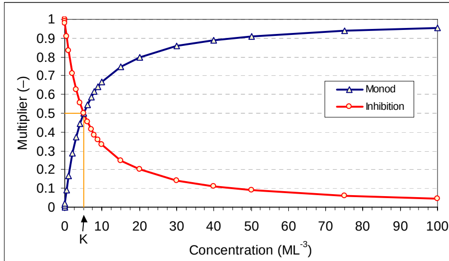
Figure 3. Arbitrary Examples of the Curves Obtained for Monod and Inhibition Terms — These terms are typically used as multipliers on the reaction rate to account for nutrient limitations and inhibition effects, respectively.
