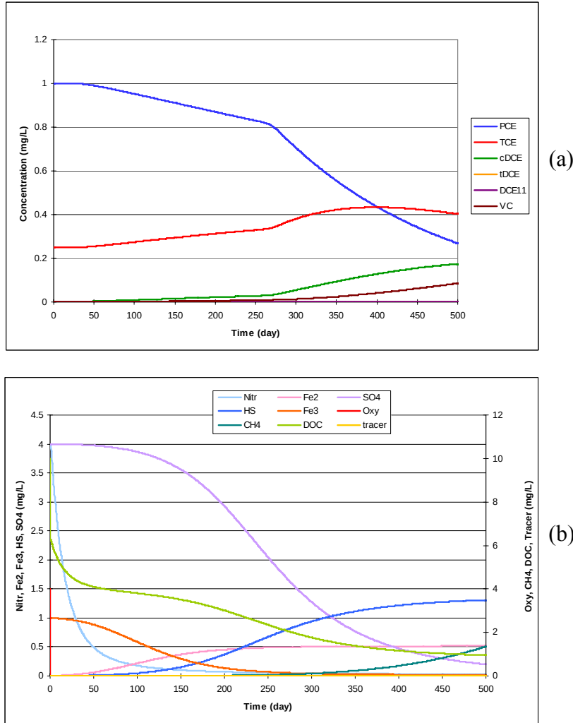
Figure 34. Example Simulation 3: Dechlorination of PCE and TCE Using the Parameter Values Shown in Table 40 — The initial concentration for PCE, TCE, oxygen, nitrate, sulfate, dissolved organic carbon, and iron(III) were 1, 0.25, 4, 4, 4, 10, and 1 mg/L, respectively. All other species concentrations started at zero. Note that the concentrations of redox species vary in this simulation according to oxidation processes and the reduction rate input parameters. Figure (a) shows chlorinated solvent concentration. Figure (b) shows the concentration of other species.
