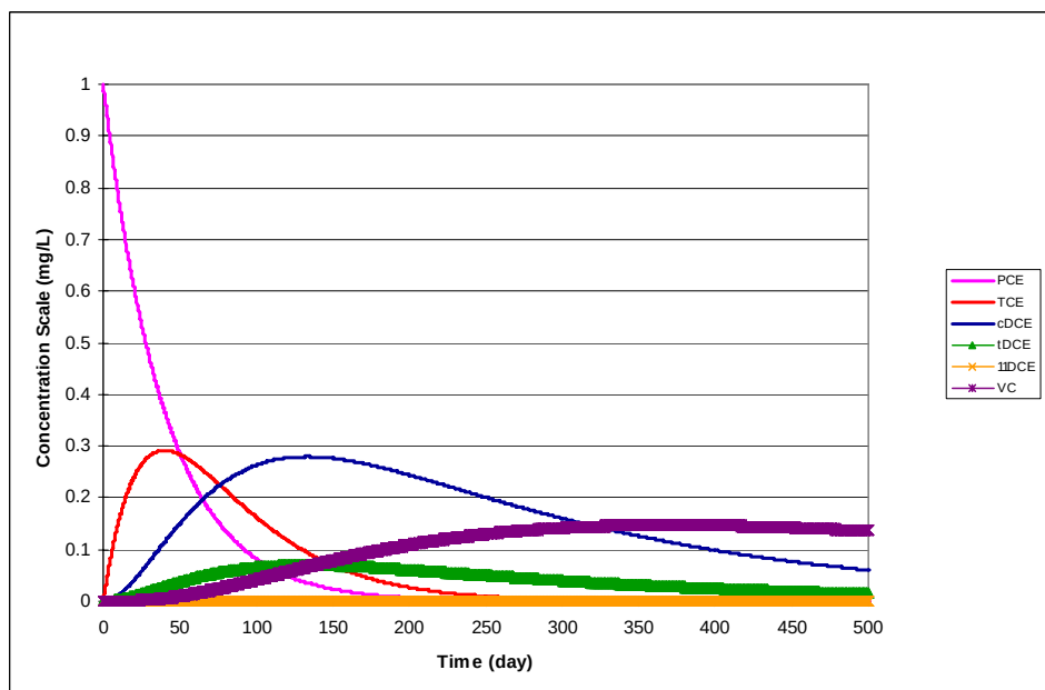
Figure 26. Dechlorination of PCE Using the Parameter Values Shown in Table 32 — The initial concentration for PCE was 1 mg/L. All other species concentrations started at zero.
