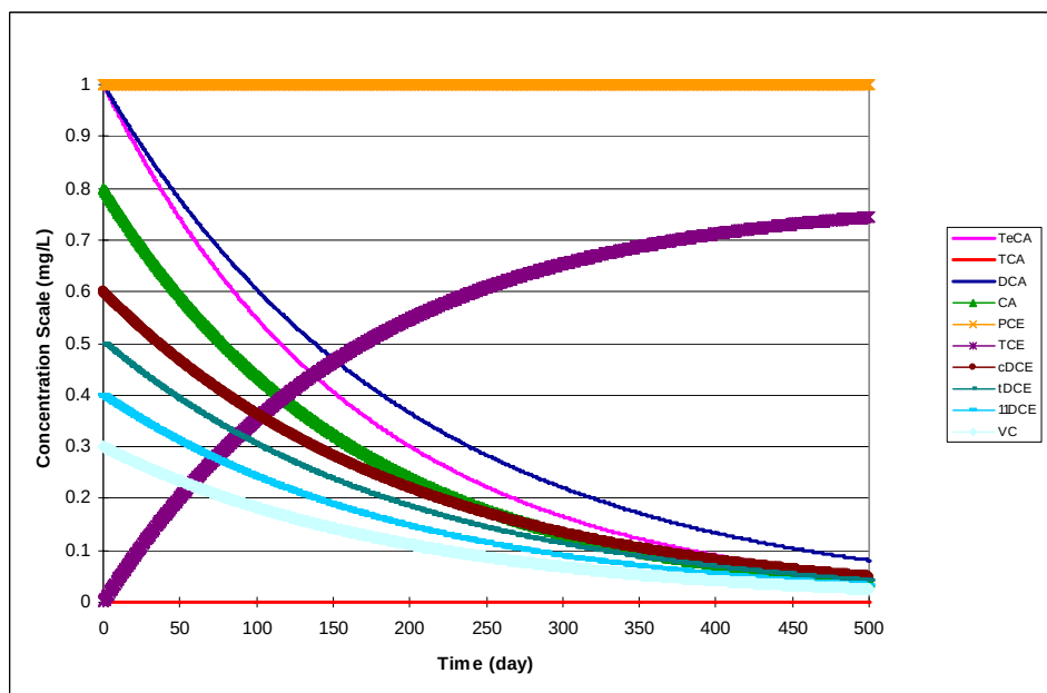
Figure 24. Aerobic and Abiotic Degradation of Contaminants in the 1,1,1,2-TeCA and PCE Families Using the Parameter Values Shown in Table 29 — The initial concentrations for TeCA, TCA, DCA, CA, PCE, TCE, cDCE, tDCE, 11DCE, and VC were 1, 0, 1, 0.8, 1, 0, 0.6, 0.5, 0.4, and 0.3 mg/L, respectively.
