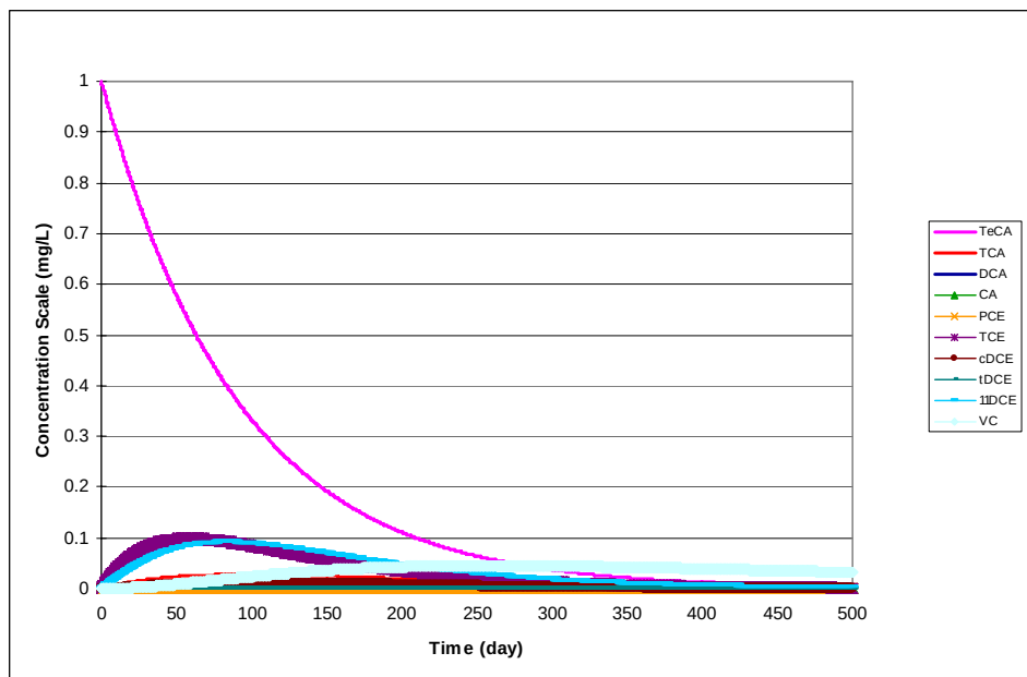
Figure 23. Dechlorination of 1,1,1,2-TeCA Using the Parameter Values Shown in Table 28 — The initial concentration for TeCA was 1 mg/L. All other species concentrations started at zero.
