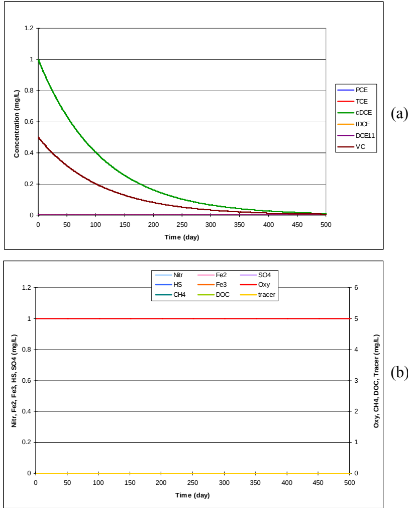
Figure 33. Example Simulation 2: Dechlorination of cDCE and VC Using the Parameter Values Shown in Table 39 — The initial concentration for cDCE, VC, oxygen, and nitrate were 1, 0.5, 5, and 1 mg/L, respectively. All other species concentrations started at zero. Note that the concentrations of redox species remain constant in this simulation. Figure (a) shows chlorinated solvent concentration. Figure (b) shows the concentration of other species.
