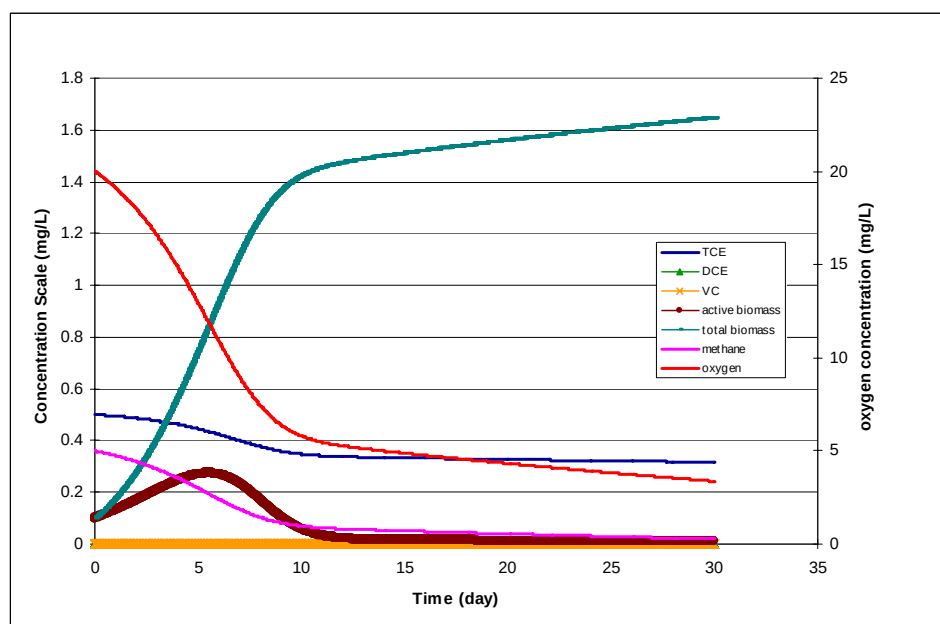
Figure 44. Dechlorination of TCE Using the Parameter Values Shown in Table 48 — The initial concentration for TCE, DCE, VC, methane, oxygen, active biomass, and total biomass were 0.5, 5, 20, 0.1, and 0.1 mg/L, respectively.
