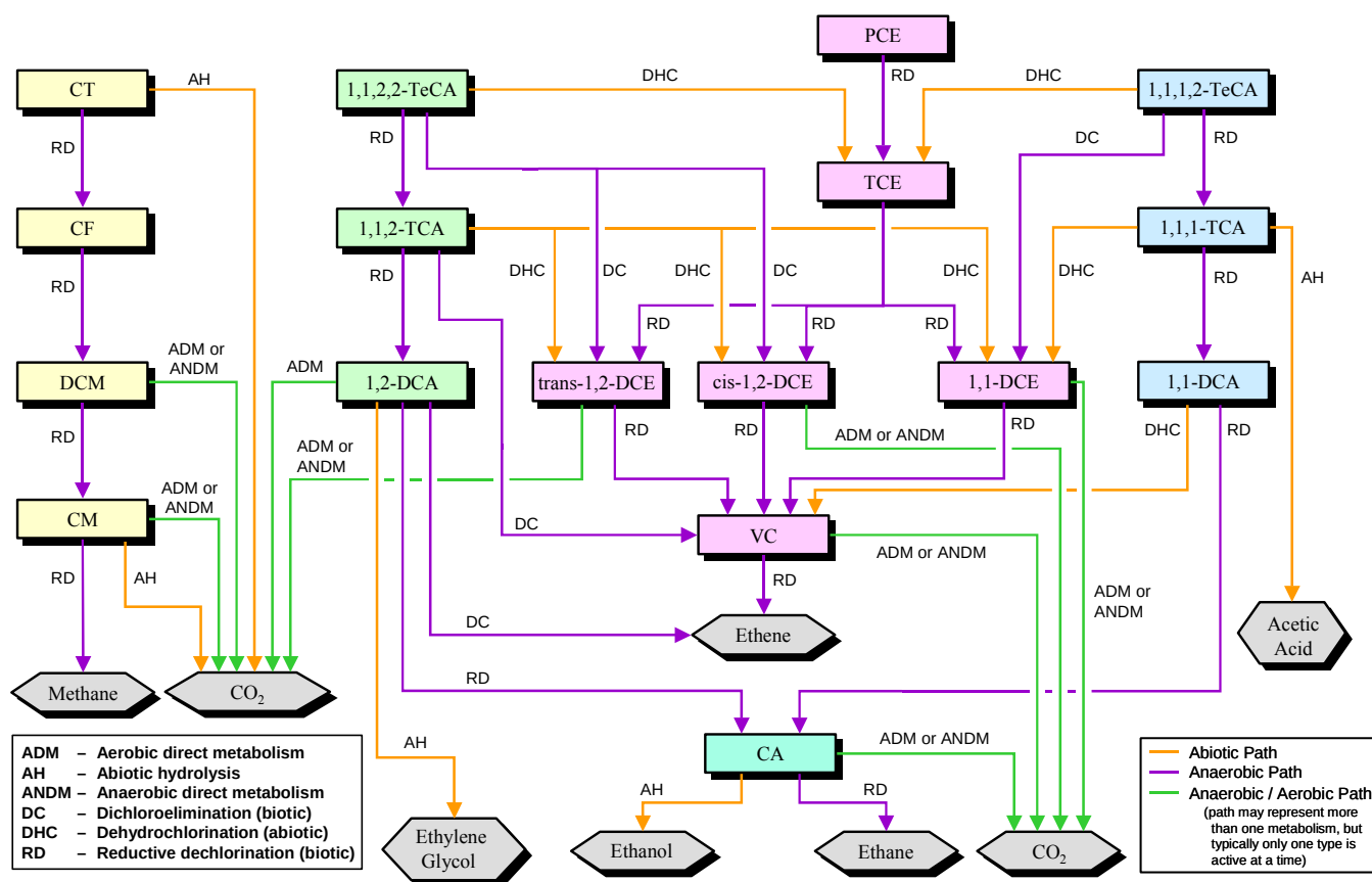
Figure 2. Reaction Pathway Network for Chlorinated Ethenes, Ethanes, and Methanes — Heterogeneous abiotic reactions, abiotic pathways with a half-life greater than 200 years, and cometabolic reaction pathways are not included.
