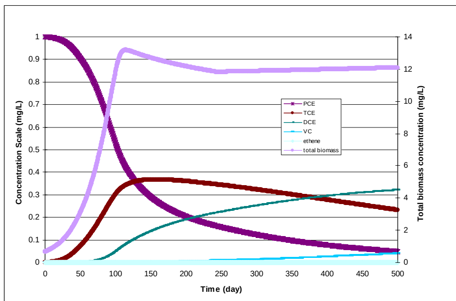
Figure 41. Dechlorination of PCE Using the Parameter Values Shown in Table 45 — The initial concentrations for PCE, lactate, oxygen, BioI, Bio2, and BioT were 1, 200, 8, 0.6, 0.06, 0.66 mg/L, respectively. All other species concentrations started at zero.
