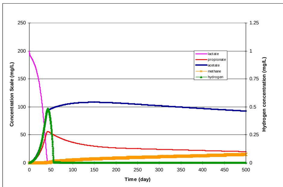
Figure 39. Concentrations of Organic Acids, Hydrogen, and Methane During Dechlorination of PCE Using the Parameter Values Shown in Table 43 — The initial concentrations for PCE, lactate, oxygen, Bio1, Bio2, and BioT were 1, 200, 8, 0.6, 0.06, 0.66 mg/L, respectively. All other species concentrations started at zero.
