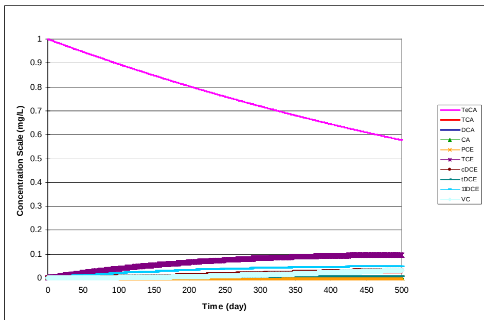
Figure 22. Dechlorination of 1,1,1,2-TeCA Using the Parameter Values Shown in Table 27 — The initial concentration for TeCA was 1 mg/L. All other species concentrations started at zero.
