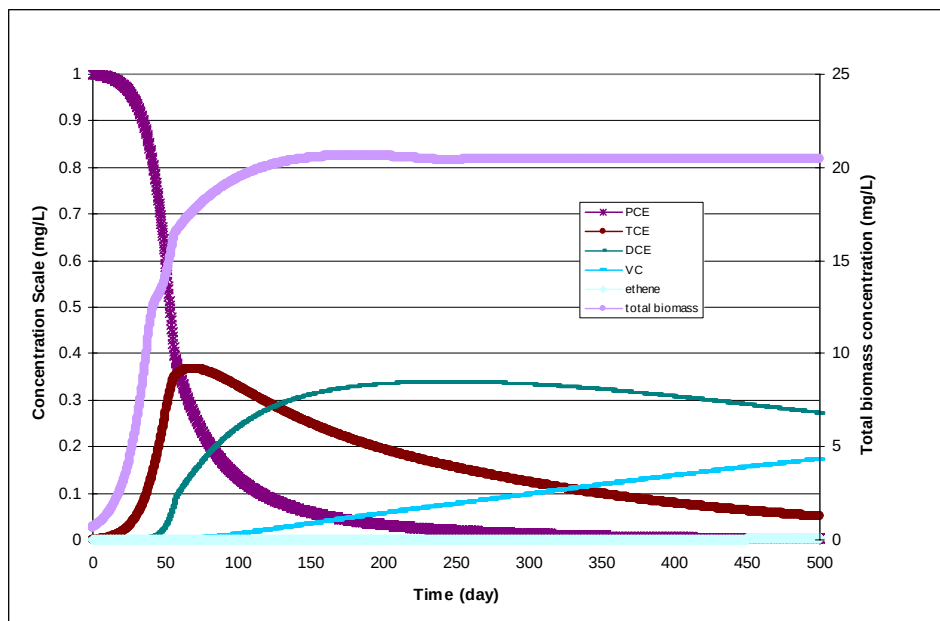
Figure 38. Dechlorination of PCE Using the Parameter Values Shown in Table 43 — The initial concentrations for PCE, lactate, oxygen, Bio1, Bio2, and BioT were 1, 200, 8, 0.6, 0.06, 0.66 mg/L, respectively. All other species concentrations started at zero.
