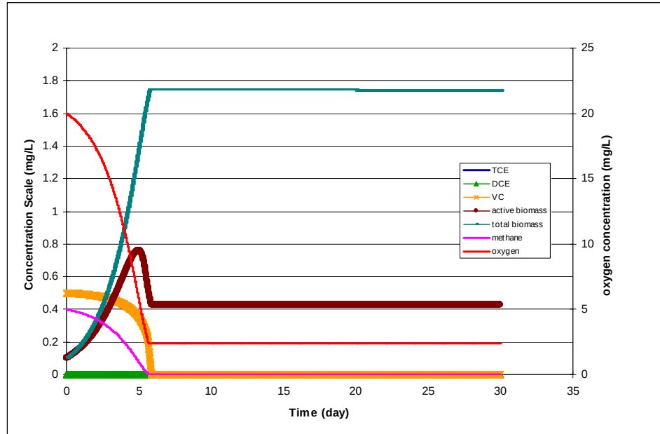
Figure 45. Dechlorination of VC Using the Parameter Values Shown in Table 48 — The initial concentration for VC, methane, oxygen, active biomass, and total biomass were 0.5, 5, 20, 0.1, and 0.1 mg/L, respectively.
