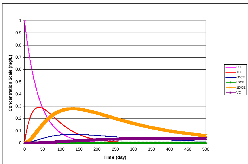
Figure 28. Dechlorination of PCE Using the Parameter Values Shown in Table 34 — The initial concentration for PCE was 1 mg/L. All other species concentrations started at zero.
