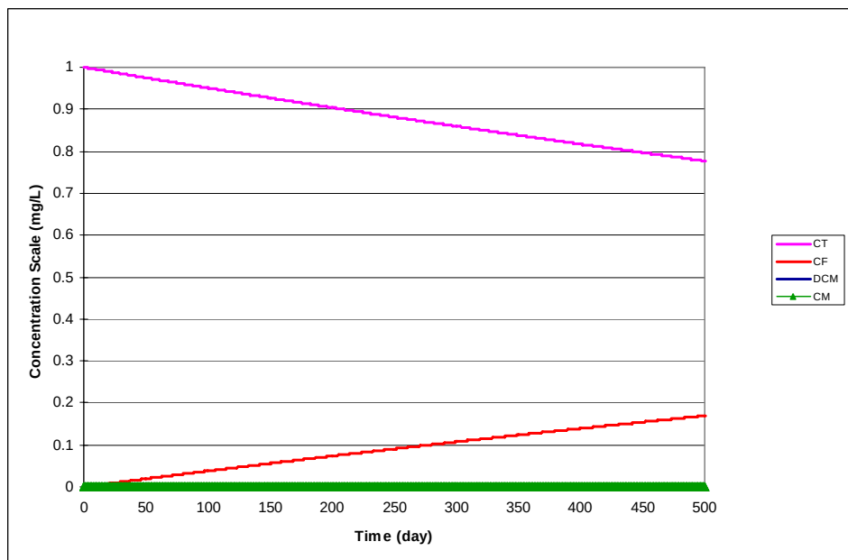
Figure 12. Dechlorination of CT Using the Parameter Values Shown in Table 15 — The initial concentration for CT was 1 mg/L. All other species concentrations started at zero.
