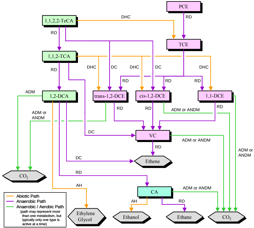
Figure 15. Conceptual Model for Dechlorination Reactions in the Dechlorination of 1,1,2,2-Tetrachloroethane and Chloroethenes Reaction Module — Species in hexagonal shaded boxes are innocuous products and are not tracked in the reaction module. The reaction types for each pathway are described in Table 3.
