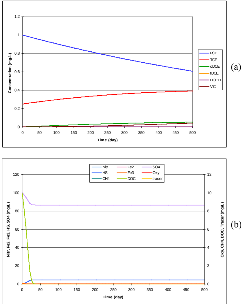
Figure 35. Example Simulation 4: Dechlorination of PCE and TCE Using the Parameter Values Shown in Table 40 — The initial concentration for PCE, TCE, sulfate, dissolved organic carbon, and iron(III) were 1, 0.25, 100, 10, and 1 mg/L, respectively. All other species concentrations started at zero. Note that the concentrations of redox species vary in this simulation according to oxidation processes and the reduction rate input parameters. Figure (a) shows chlorinated solvent concentration. Figure (b) shows the concentration of other species.
