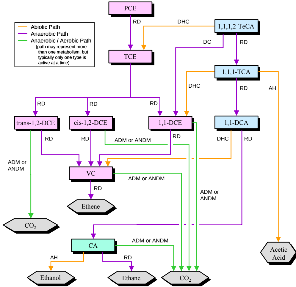
Figure 20. Conceptual Model for Dechlorination Reactions in the Dechlorination of 1,1,1,2-Tetrachloroethane and Chloroethenes Reaction Module — Species in hexagonal shaded boxes are innocuous products and are not tracked in the reaction module. The reaction types for each pathway are described in Table 3.
