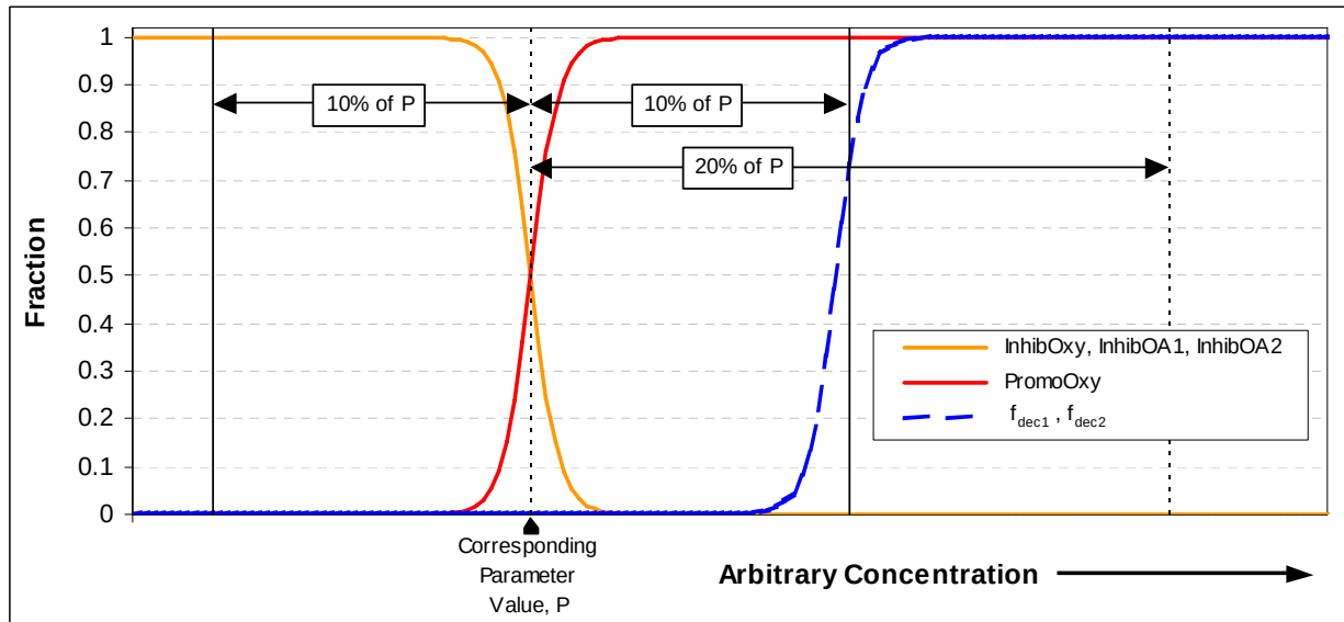
Figure 37. Conceptual Diagram of the Behavior of the Function Representing a Change in Conditions as a Smooth Transition in the Form of a Sigmoidal Curve — This diagram depicts the trend for the various groups of parameters; the actual curves will be shifted on the X-axis based on the corresponding target concentration.
