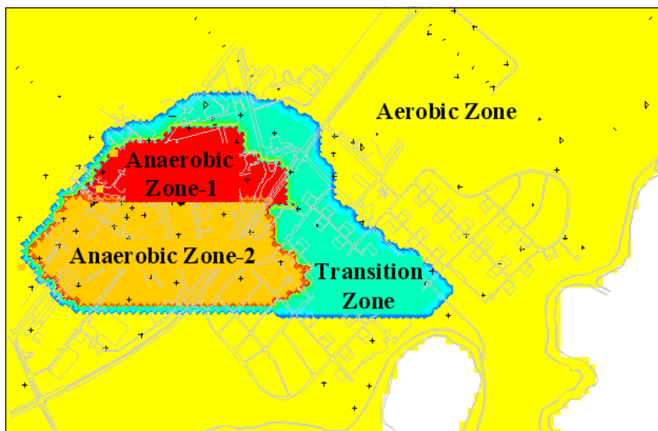
Figure 4. Example of a Reactive Transport Model Having Multiple Reaction Zones, Each with Differing Reaction Parameter Values — Figure adapted from Clement et al. [2000].
