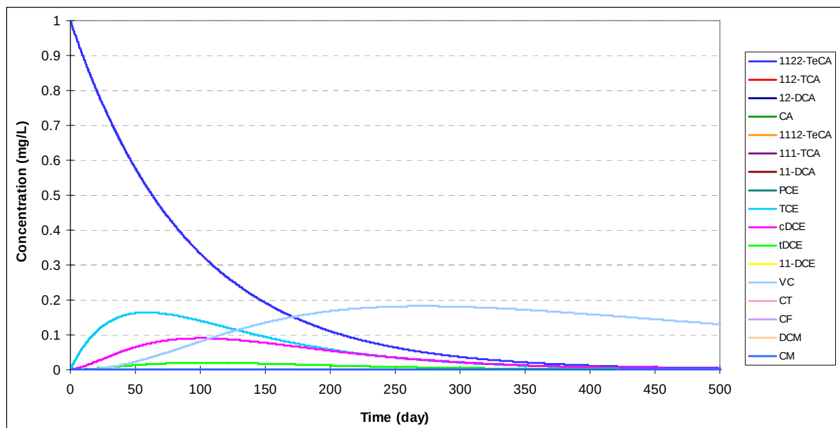
Figure 8. Dechlorination of Mixed Chlorinated Solvents Using the Parameter Values Shown in Table 10 — The initial concentration of 1122TeCA was set to 1 mg/L. All other species concentrations started at zero. These results are the same as produced by the Dechlorination of 1,1,2,2-Tetrachloroethane and Chloroethenes reaction module (Figure 16).
