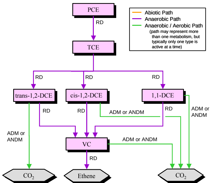
Figure 25. Conceptual Model for Dechlorination Reactions in the Chloroethene Dechlorination Reaction Module — Species in hexagonal shaded boxes are innocuous products and are not tracked in the reaction module. The reaction types for each pathway are described in Table 3.
