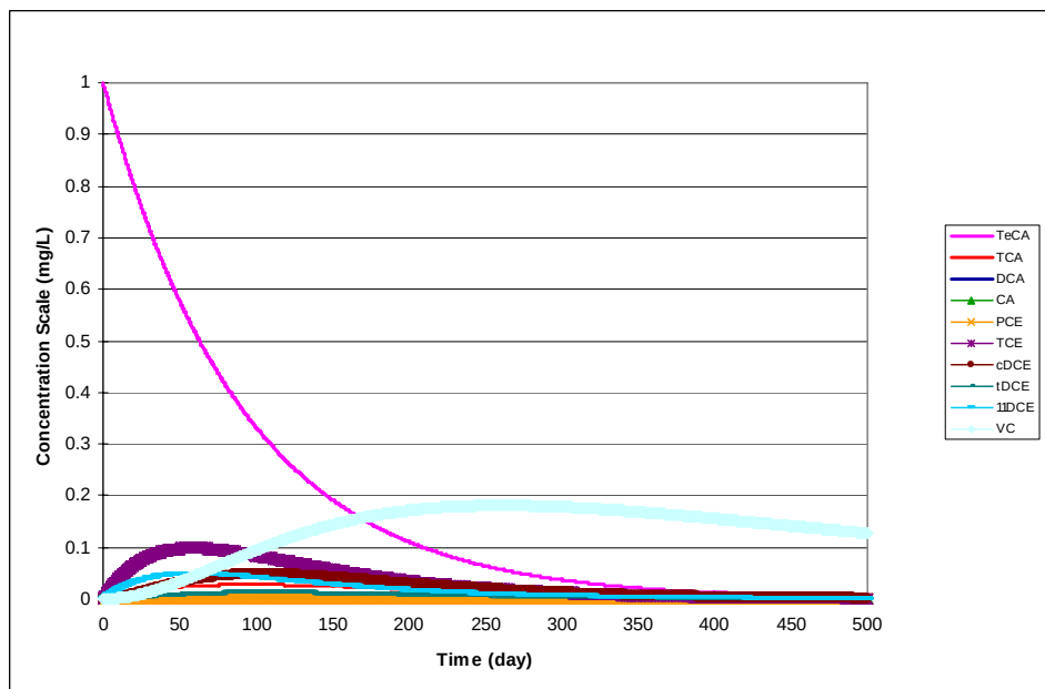
Figure 21. Dechlorination of 1,1,1,2-TeCA Using the Parameter Values Shown in Table 26 — The initial concentration for TeCA was 1 mg/L. All other species concentrations started at zero.
