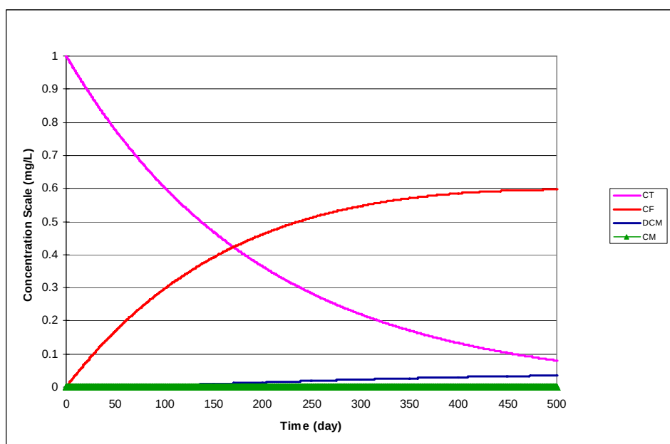
Figure 13. Dechlorination of CT Using the Parameter Values Shown in Table 16 — The initial concentration for CT was 1 mg/L. All other species concentrations started at zero.
