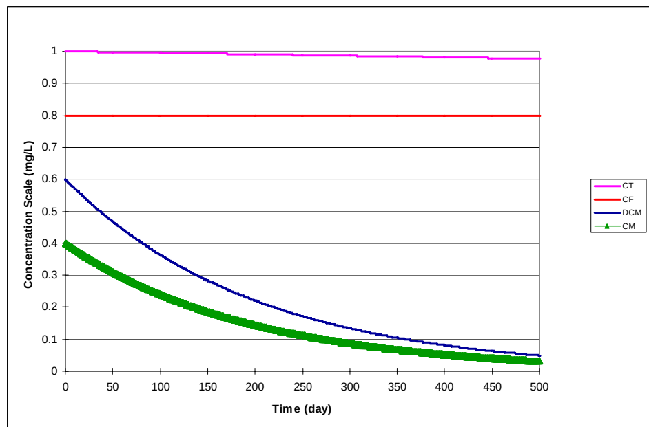
Figure 14. Aerobic and Abiotic Degradation Using the Parameter Values Shown in Table 17 — The initial concentrations for CT, CF, DCM, and CM were 1, 0.8, 0.6, and 0.4 mg/L, respectively.
