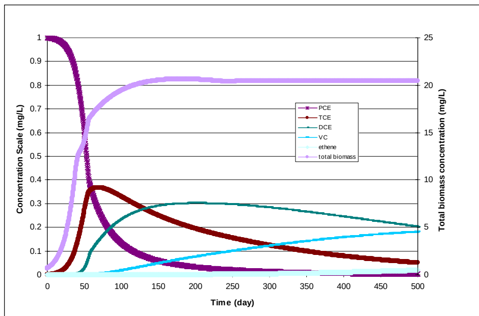
Figure 40. Dechlorination of PCE Using the Parameter Values Shown in Table 44 — The initial concentrations for PCE, lactate, oxygen, BioI, Bio2, and BioT were 1, 200, 8, 0.6, 0.06, 0.66 mg/L, respectively. All other species concentrations started at zero. The organic acids, hydrogen, and methane results are the same as shown in Figure 39.
