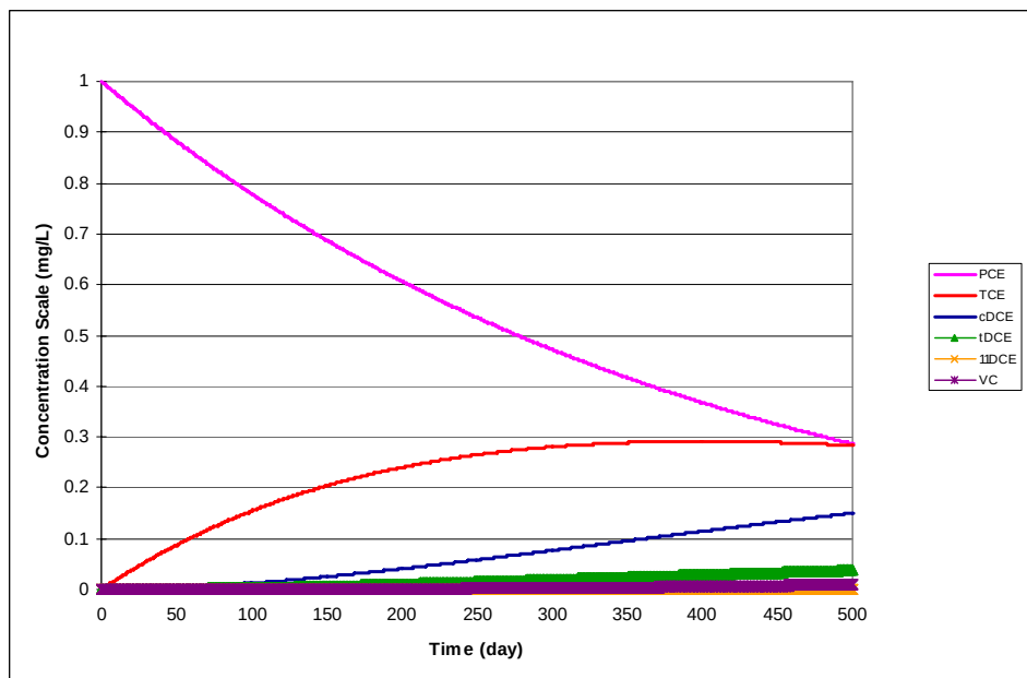
Figure 27. Dechlorination of PCE Using the Parameter Values Shown in Table 33 — The initial concentration for PCE was 1 mg/L. All other species concentrations started at zero.
