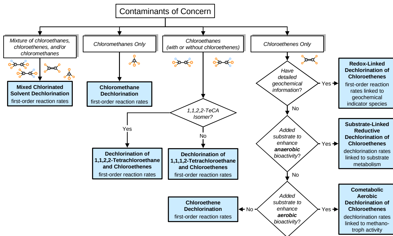
Figure 1. Flowchart Depicting the Logic for Selection of RT3D MNA/EA Reaction Modules Based on the Contaminant(s) Present, What Data is Available, and the MNA/EA Scenario under Consideration
