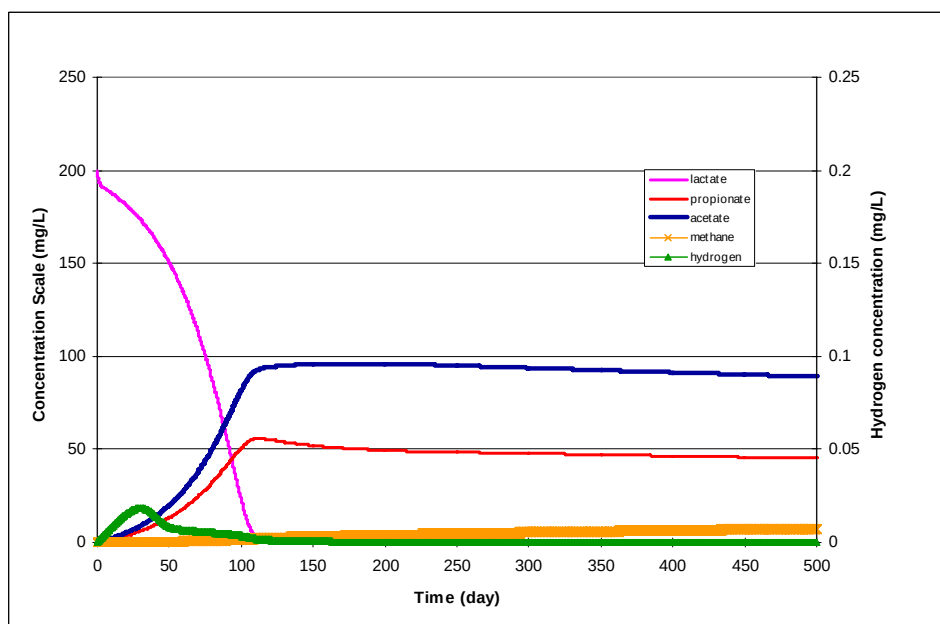
Figure 42. Concentrations of Organic Acids, Hydrogen, and Methane During Dechlorination of PCE Using the Parameter Values Shown in Table 45 — The initial concentrations for PCE, lactate, oxygen, Bio1, Bio2, and BioT were 1, 200, 8, 0.6, 0.06, 0.66 mg/L, respectively. All other species concentrations started at zero.
