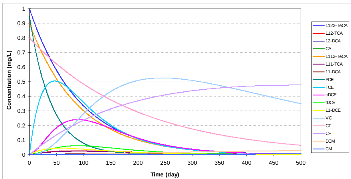
Figure 6. Dechlorination of Mixed Chlorinated Solvents under Anaerobic Conditions Using the Parameter Values Shown in Table 8 — Initial concentrations were set to 1.0, 0.9, 0.95, and 0.8 mg/L for 1122TeCA, 1112TeCA, PCE, and CT, respectively. All other species concentrations started at zero.
