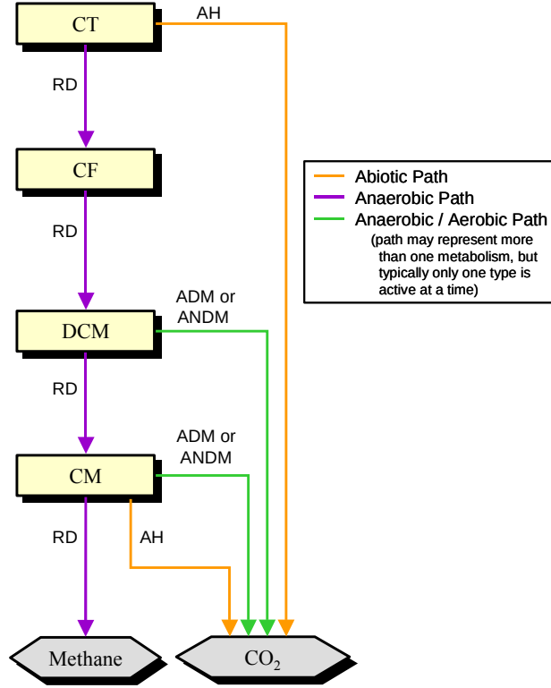
Figure 10. Conceptual Model for Dechlorination Reactions in the Chloromethane Dechlorination Reaction Module — Species in hexagonal shaded boxes are innocuous products and are not tracked in the reaction module. The reaction types for each pathway are described in Table 3.
