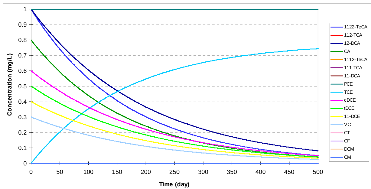
Figure 9. Aerobic and Abiotic Degradation Using the Parameter Values Shown in Table 11 — The initial concentrations for 1122TeCA, 12DCA, and PCE were 1.0 mg/L. The initial concentrations were set to 0.8, 0.6, 0.5, 0.4, and 0.3 mg/L for CA, cDCE, tDCE, 11DCE, and VC, respectively. These results are the same as produced by the Dechlorination of 1,1,2,2-Tetrachloroethane and Chloroethenes reaction module (Figure 19).
