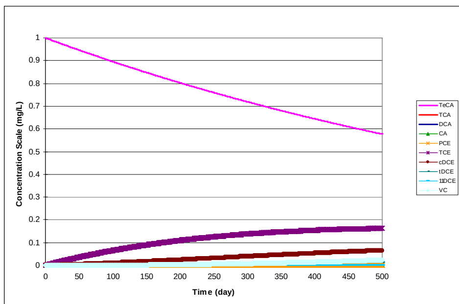
Figure 17. Dechlorination of 1,1,2,2-TeCA Using the Parameter Values Shown in Table 21 — The initial concentration for TeCA was 1 mg/L. All other species concentrations started at zero.
