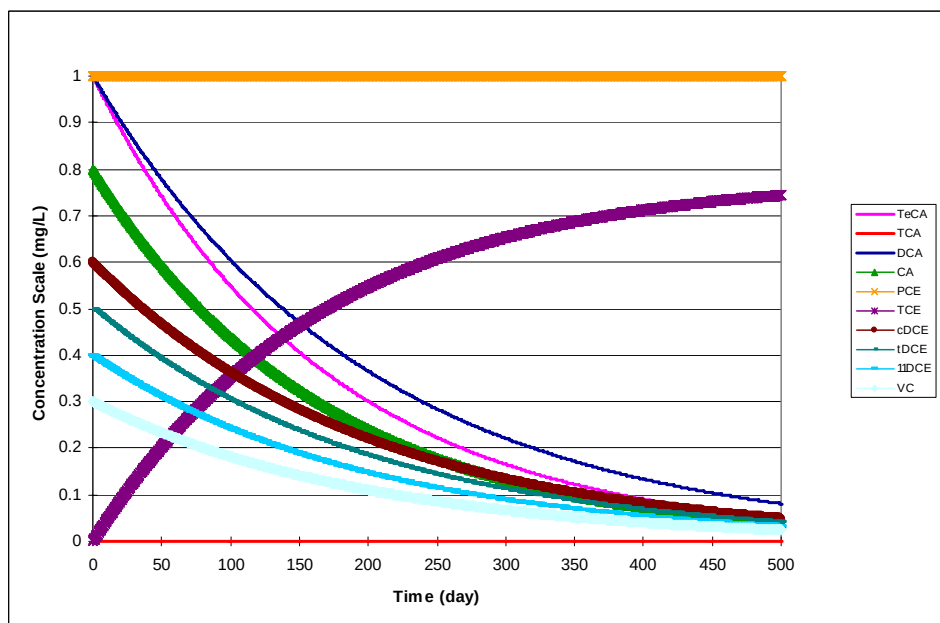
Figure 19. Aerobic and Abiotic Degradation of Contaminants in the 1,1,2,2-TeCA and PCE Families Using the Parameter Values Shown in Table 23 — The initial concentrations for TeCA, TCA, DCA, CA, PCE, TCE, cDCE, tDCE, 11DCE, and VC were 1, 0, 1, 0.8, 1, 0, 0.6, 0.5, 0.4, and 0.3 mg/L, respectively.
