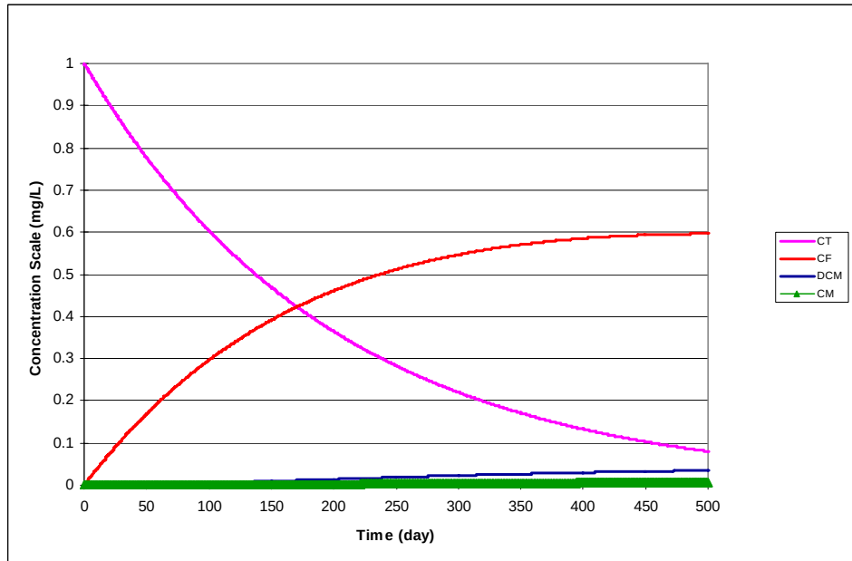
Figure 11. Dechlorination of CT Using the Parameter Values Shown in Table 14 — The initial concentration for CT was 1 mg/L. All other species concentrations started at zero.
