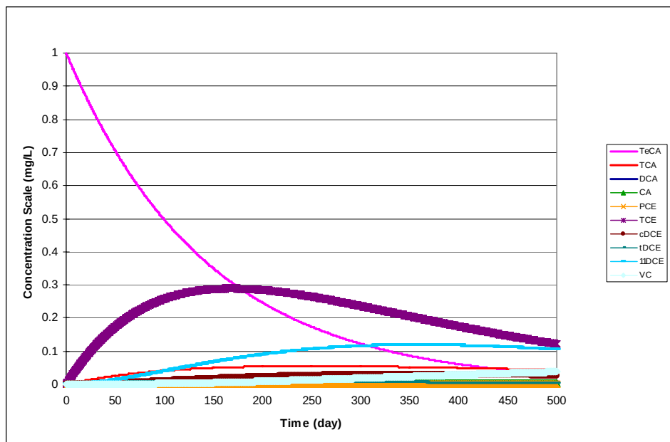
Figure 18. Dechlorination of 1,1,2,2-TeCA Using the Parameter Values Shown in Table 22 — The initial concentration for TeCA was 1 mg/L. All other species concentrations started at zero.
