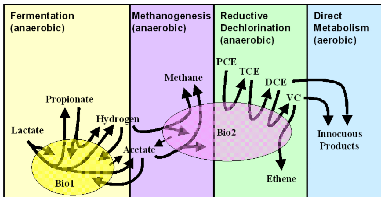
Figure 36. Conceptual Model for the Reductive Dechlorination Reactions of the Substrate-Linked Reductive Dechlorination of Chloroethenes Reaction Module
