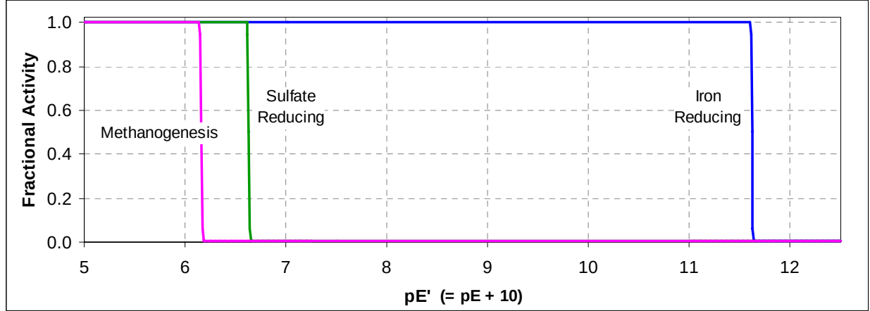
Figure 31. pE Value (On a Shifted Scale) at Which Each Anaerobic Dechlorination Mechanism Dominates
