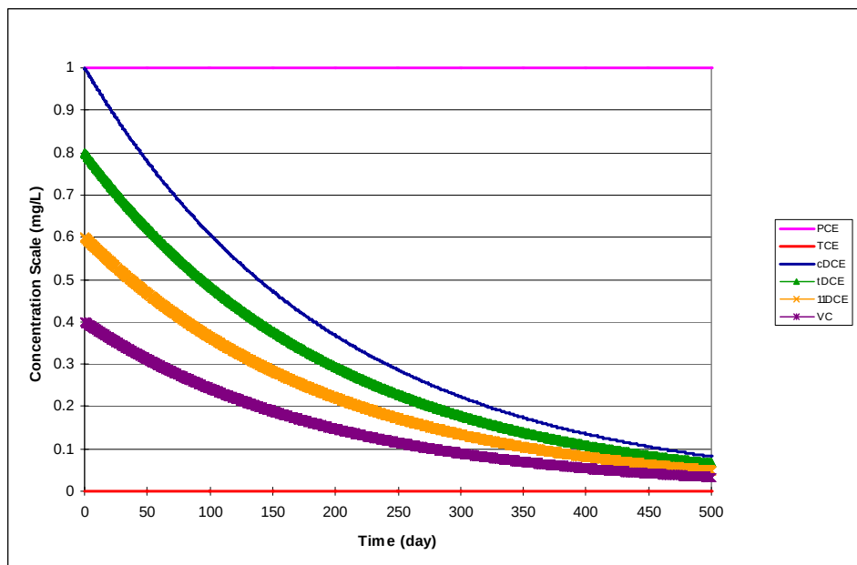
Figure 29. Aerobic and Abiotic Degradation Using the Parameter Values Shown in Table 35 — The initial concentrations for PCE, TCE, cDCE, tDCE, 11DCE, and VC were 1, 0, 1, 0.8, 0.6, and 0.4 mg/L, respectively.
