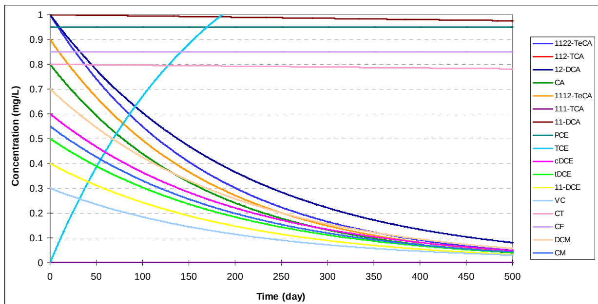
Figure 7. Dechlorination of Mixed Chlorinated Solvents under Aerobic Conditions Using the Parameter Values Shown in Table 9 — Initial concentrations were set to 1.0 mg/L for 1122TeCA, 12DCA, and 11DCA. Initial concentrations were set to 0.9, 0.95, 0.8, 0.8, 0.6, 0.5, 0.4, 0.3, 0.85, 0.7, and 0.55 mg/L for 1112TeCA, PCE, CT, CA, cDCE, tDCE, 11DCE, VC, CF, DCM, and CM, respectively. All other species concentrations started at zero.
