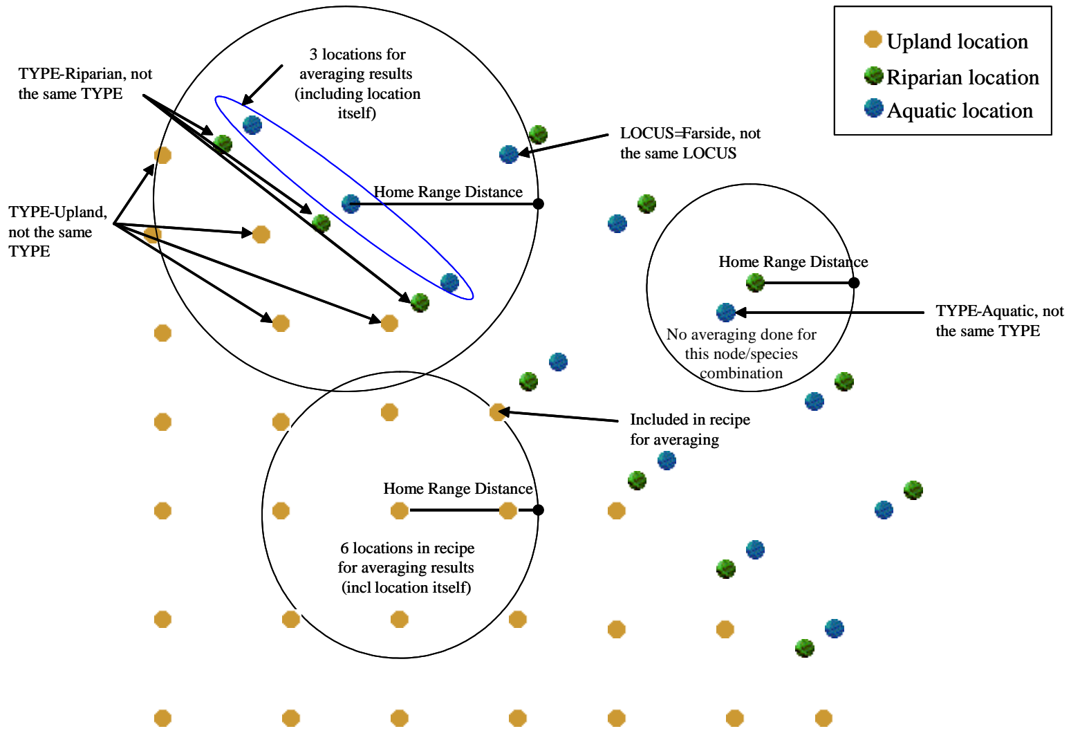
Figure 1. Example Illustrating Concepts Used in MOBILEHOME to Determine Ecological Risk to Organisms
