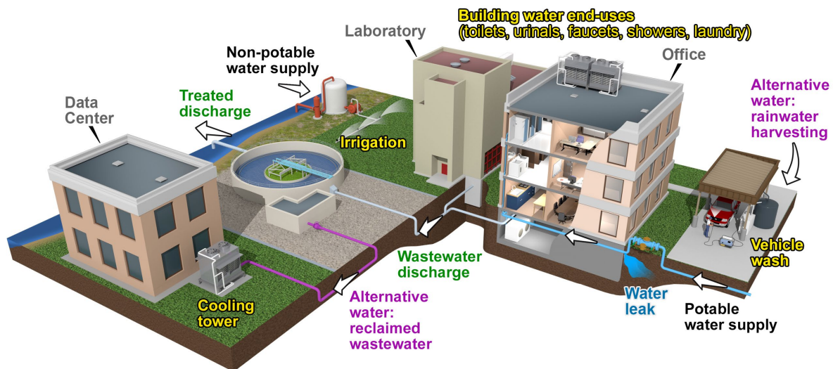
Figure 3. Example Facility Water Cycle
