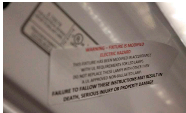
Figure 3. Some replacement options require the existing fixture wiring to be modified by an electrician. The replacement lamps (UL Type B or C) or retrofit kit should include a label like the one shown here to communicate the risks associated with the modification. The label should be visible to maintenance staff servicing the fixture. Photo courtesy of Michael Myer, PNNL.
