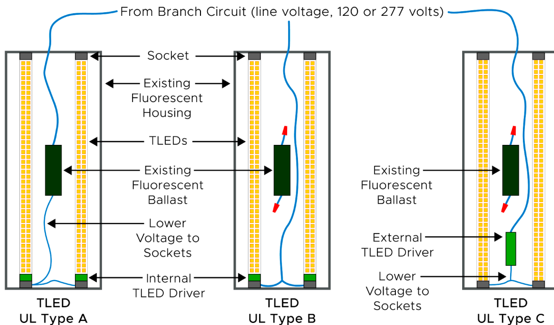
Figure 2. TLEDs can fit into existing sockets. UL Type A TLEDs use the existing fluorescent ballast. UL Type A and B TLEDs have internal drivers while UL Type C TLEDs use external drivers.
