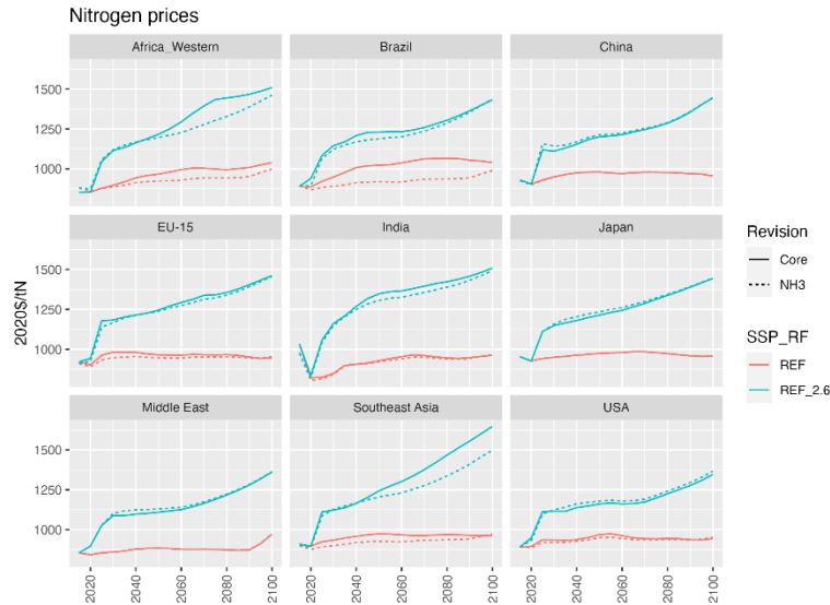
Figure 7. Prices for Nitrogen ("N fertilizer") paid by the agricultural sector in each of 9 regions, for the REF and REF_2.6 scenarios.
