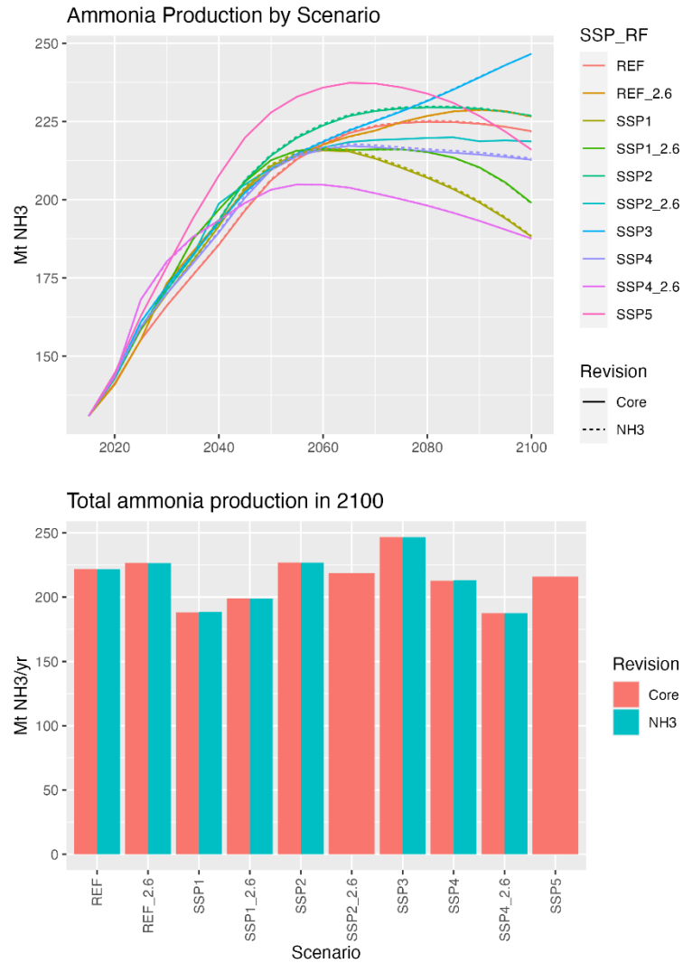
Figure 3. Ammonia production by (a) technology and year, (b) scenario and year, and (c) scenario in 2100, comparing the core model to the revision implemented here. The core model's "N fertilizer" production values are multiplied by 17/14 to translate from the modeled commodity to ammonia equivalent. The SSP2_2.6 and SSP5 scenarios did not solve in the testing runs of the NH3 revision model branch.
