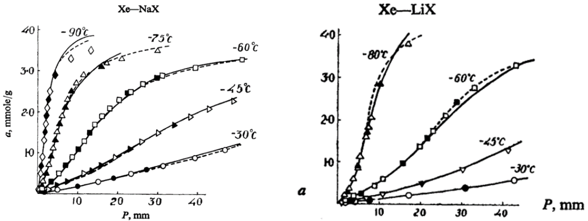
Figure 1. Isotherms of xenon in zeolite NaX (left) and LiX (right) at different temperatures. Solid and dashed lines were calculated from equations while dots are experimental data [5].
