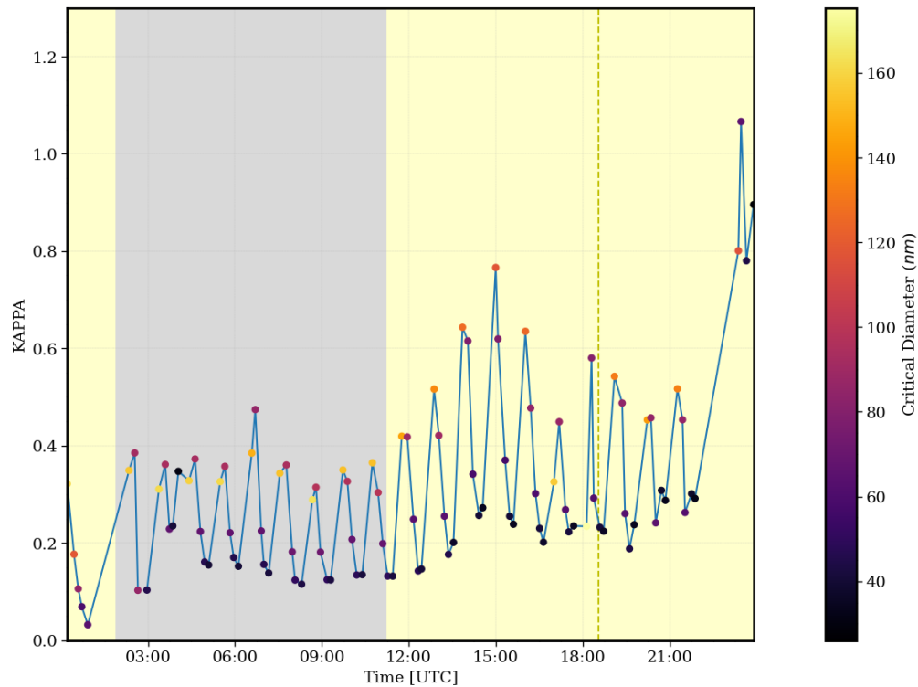
Figure 3. \kappa versus time on 2020-06-27 at the SGP E13 observatory using SMPS data.
