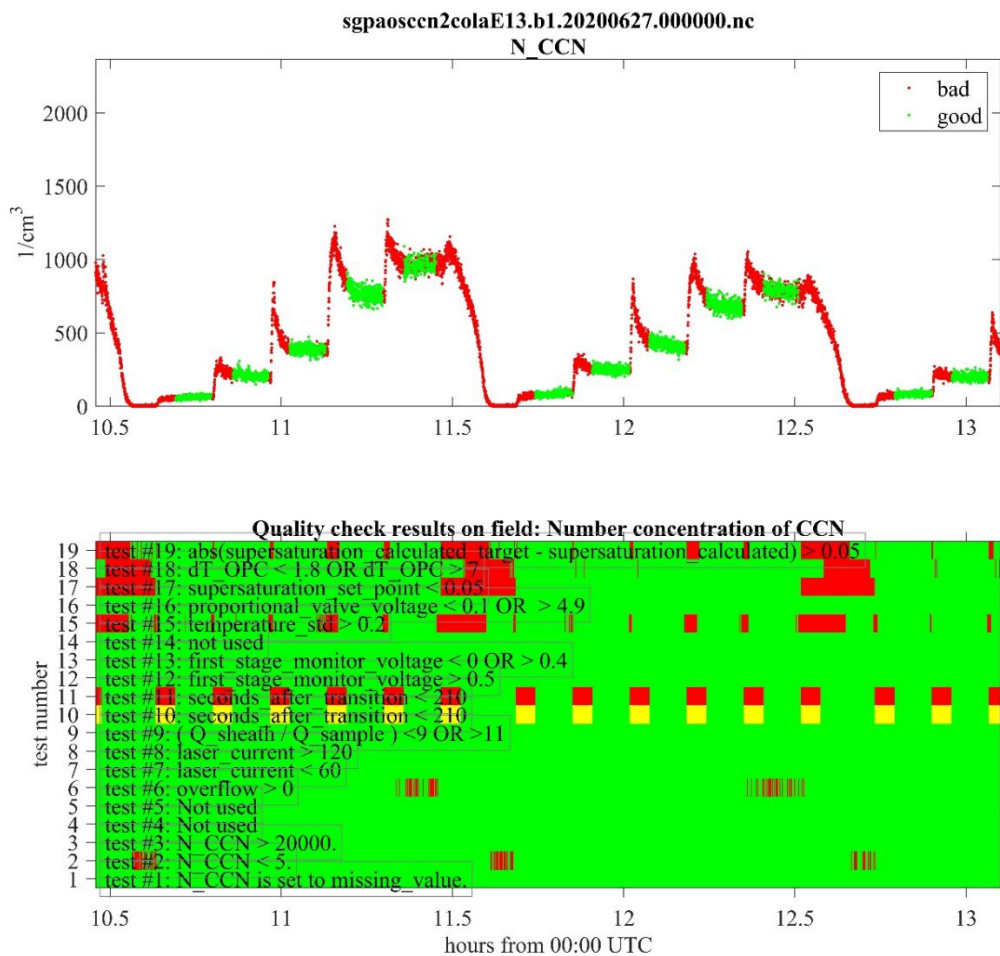
Figure 8. CCN concentrations and quality assessments from aosccn2cola.b1 at SGP E13.
