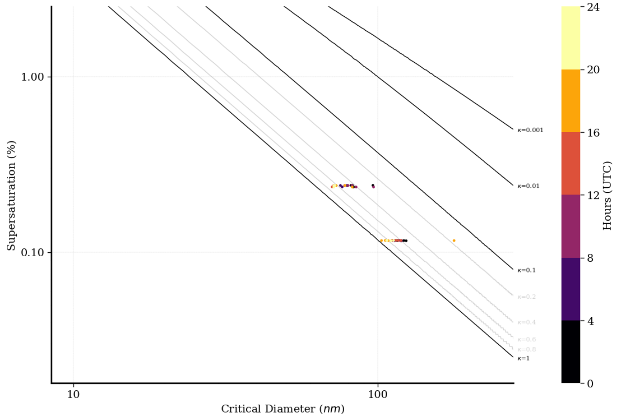
Figure 5. Supersaturation versus critical diameter with reference \kappa constant lines on 2016-08-01 at the Eastern North Atlantic (ENA) C1 observatory using UHSAS data.
