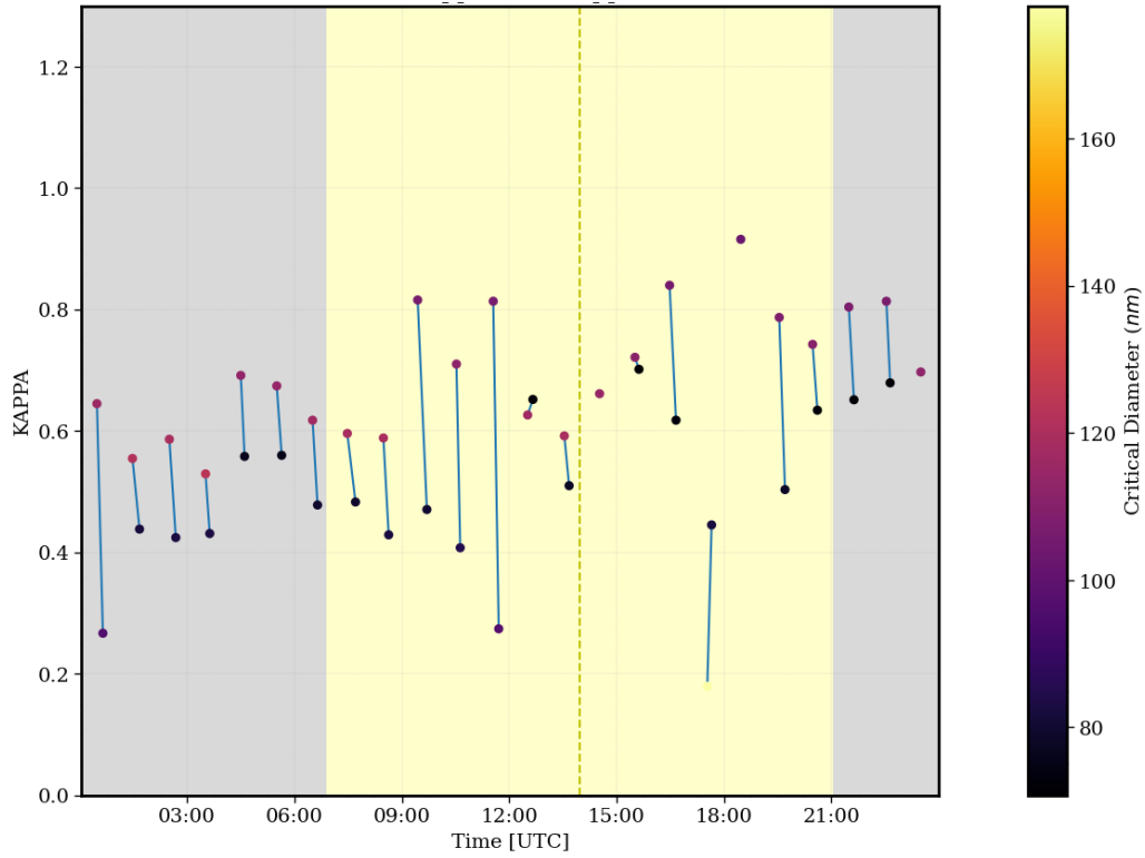
Figure 6. \kappa versus time on 2016-08-01 at the ENA C1 observatory using UHSAS data.
