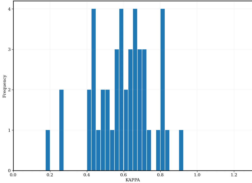
Figure 7. Frequency distribution of \kappa on 2016-08-01 using UHSAS data.
