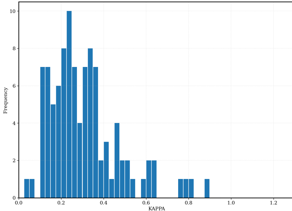
Figure 4. Frequency distribution of \kappa on 2020-06-27 at the SGP E13 observatory using SMPS data.
