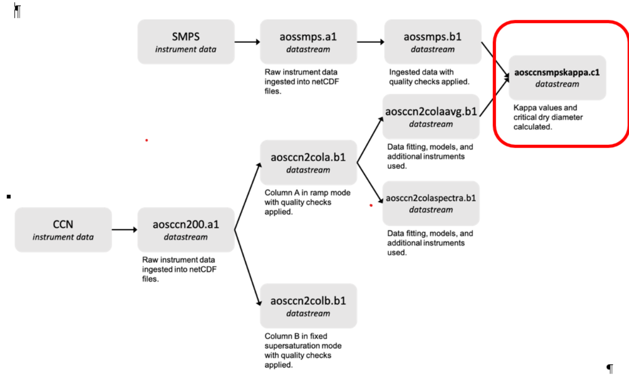
Figure 1. Diagram depicting data flows for the SMPS and CCN instruments. The highlighted box shows the VAP product datastream described in this report.
