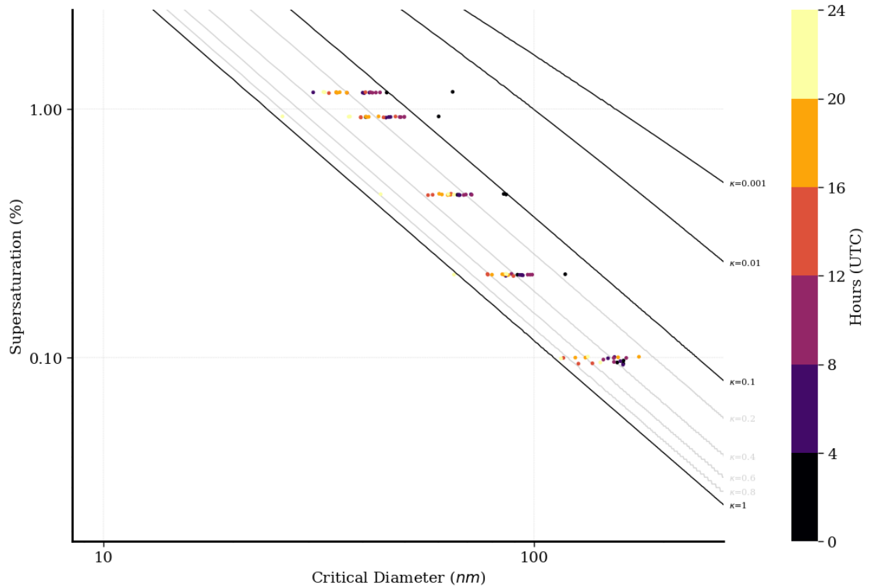
Figure 2. Supersaturation versus critical diameter with reference \kappa constant lines on 2020-06-27 at the Southern Great Plains (SGP) E13 observatory using SMPS data.
