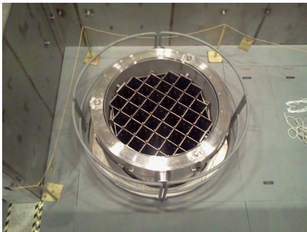
Figure 2-133. TSC-37 Canister Inside Transfer Cask
