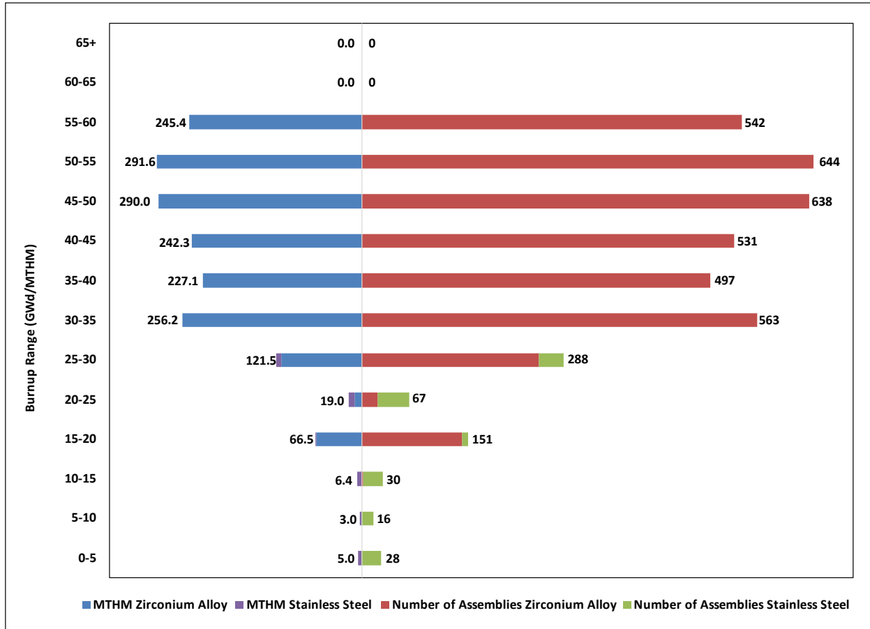
Figure 2-508. Indian Point Number of Assemblies and MTHM versus Burnup
