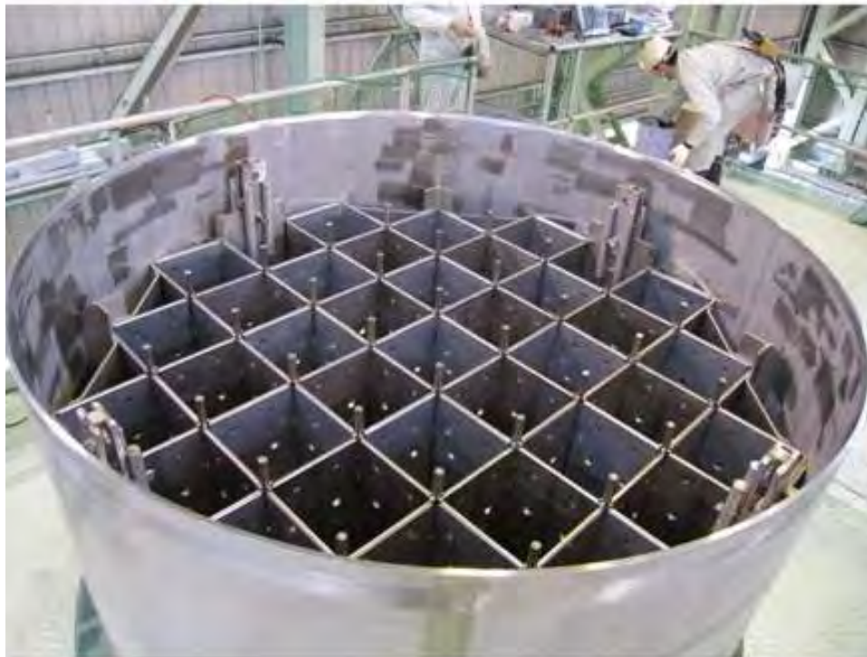
Figure 2-131. TSC-37 Canister Showing Internal Baskets Which Hold Spent Nuclear Fuel Assemblies
