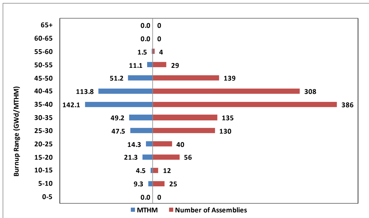
Figure 2-343. Fort Calhoun Number of Assemblies and MTHM versus Burnup (EIA 2018)
