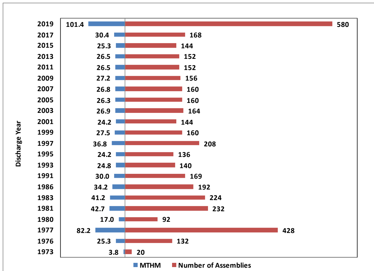
Figure 2-405. Pilgrim Number of Assemblies and MTHM versus Discharge Year
