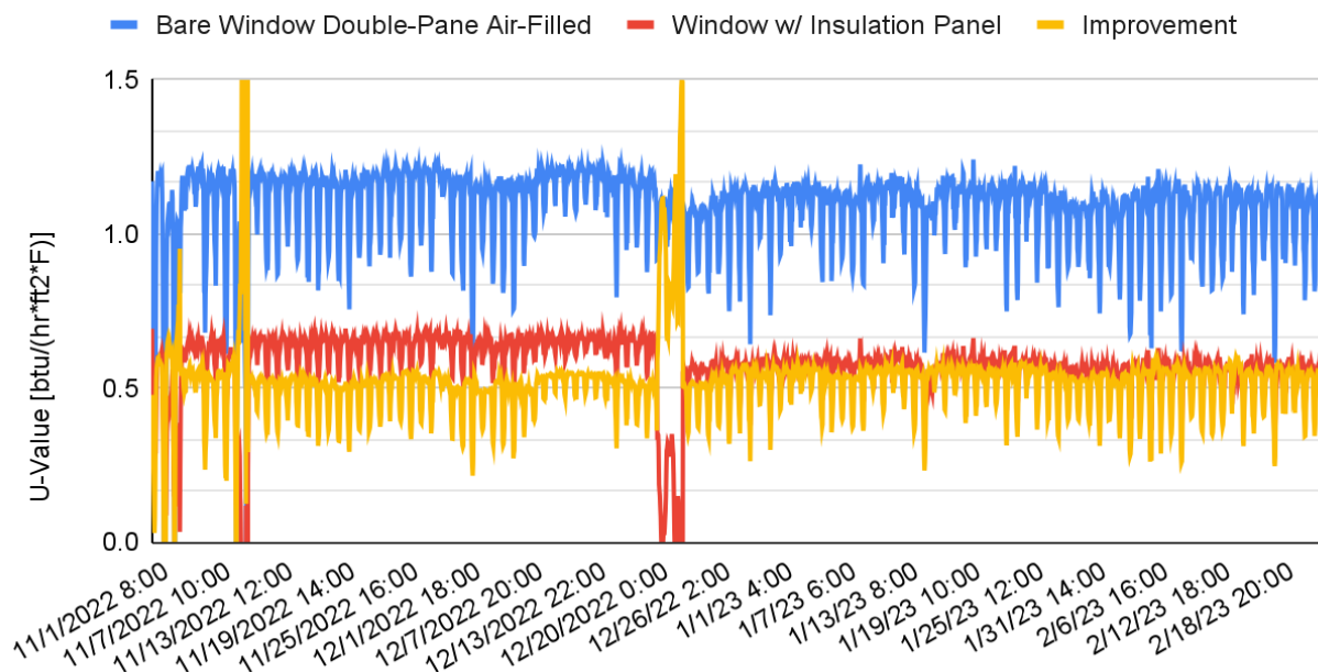
Figure 9. Comparison of the U-values of a bare window and a window with an insulation panel without a radiator below the windows.
