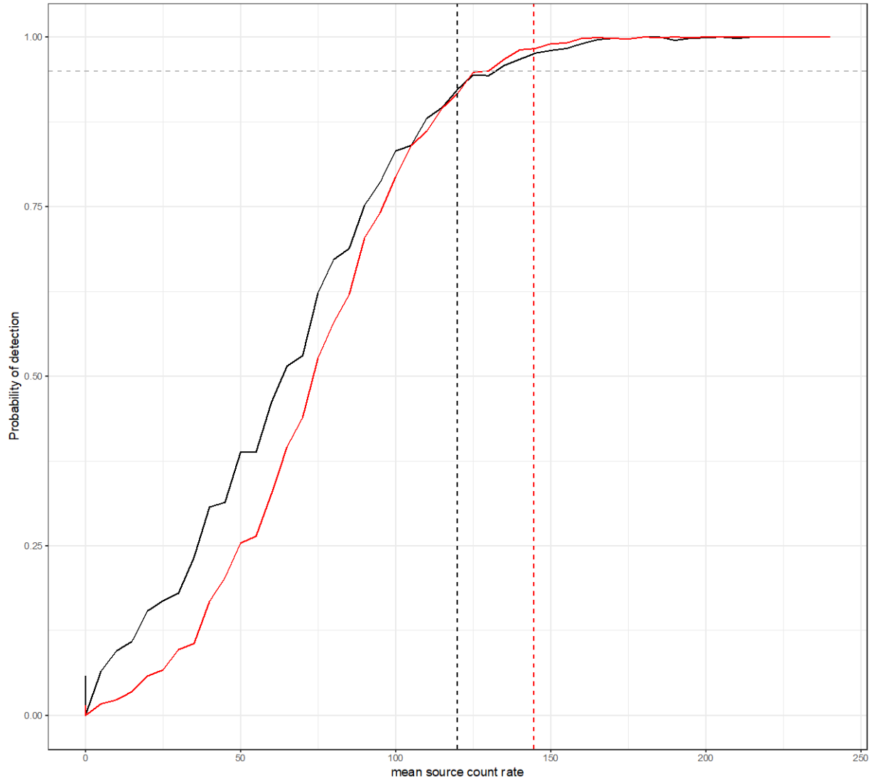
Figure 4.3. Probability of detecting a source term as a function of mean source count rate. Solid lines represent calculated probabilities of detection using the non-localized hypothesis test (red) and lag- k hypothesis method (black). Each point on the line represents the observed probability of detection (y-axis) for a given mean source count rate (x-axis). The vertical dashed lines are the calculated detection limit for each method. These results are based on 1,000 simulations from a process with non-constant background ( A = 0 ).
