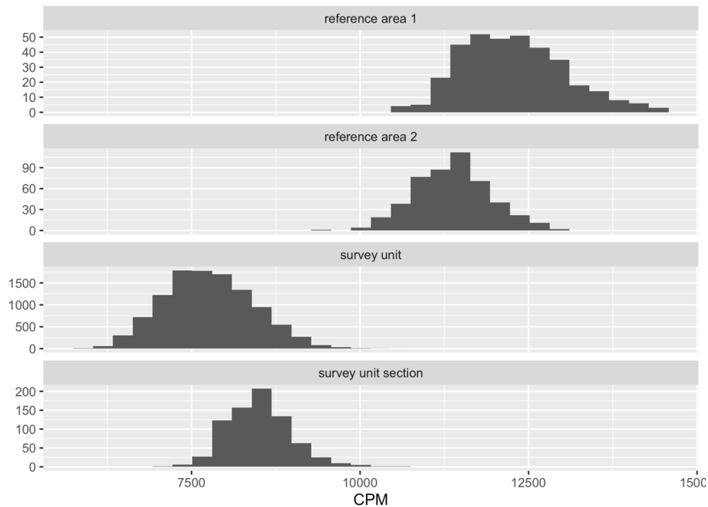
Figure 5.4. Histograms of survey unit and reference area data (with counts on the y-axis and cpm on the x-axis). Reference Areas 1 and 2 correspond to Figures 5.1 and 5.2, respectively. The survey unit and survey unit sections correspond to Figures 5.3 and 5.6, respectively. Note that the reference areas are shifted right of the survey data. Reference area 1 has a higher standard deviation than any other area.
