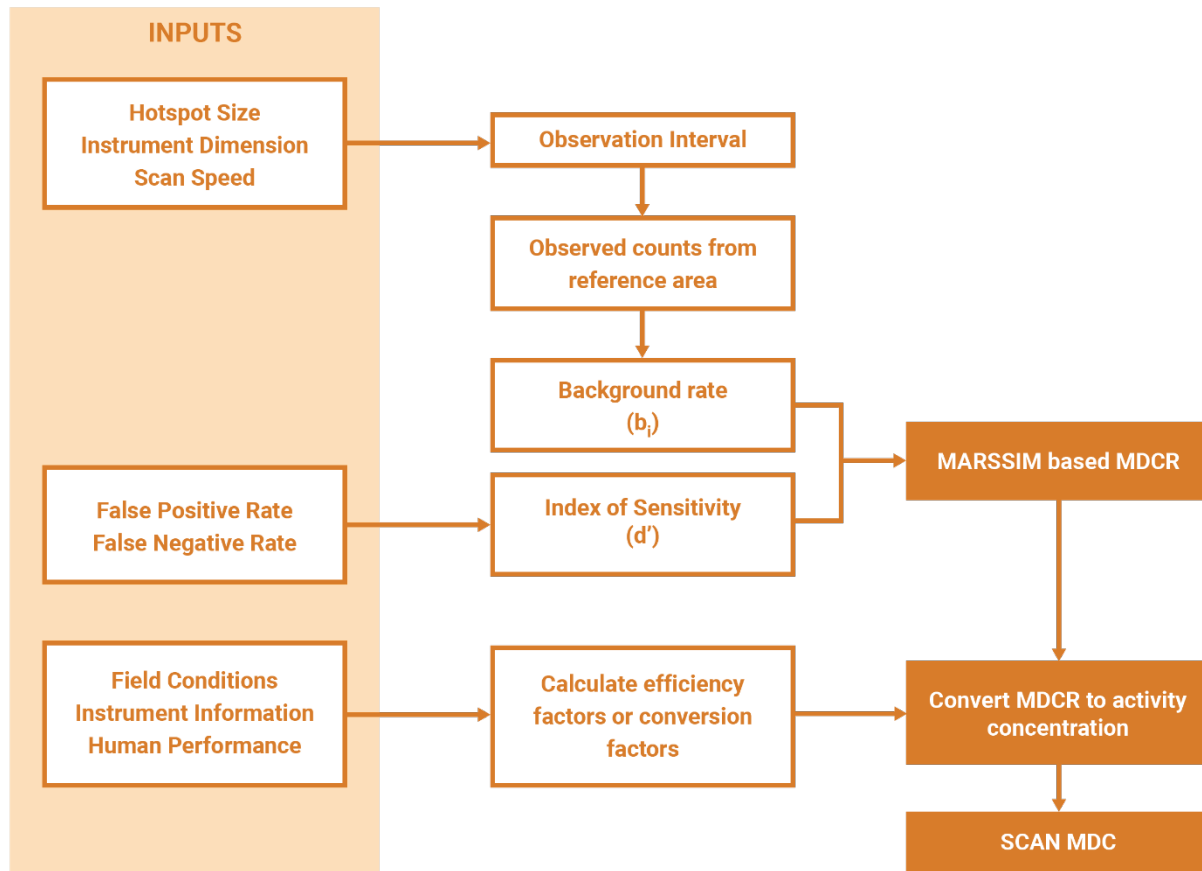
Figure 3.1. Flowchart showing the requirements for calculating a scan MDC.
