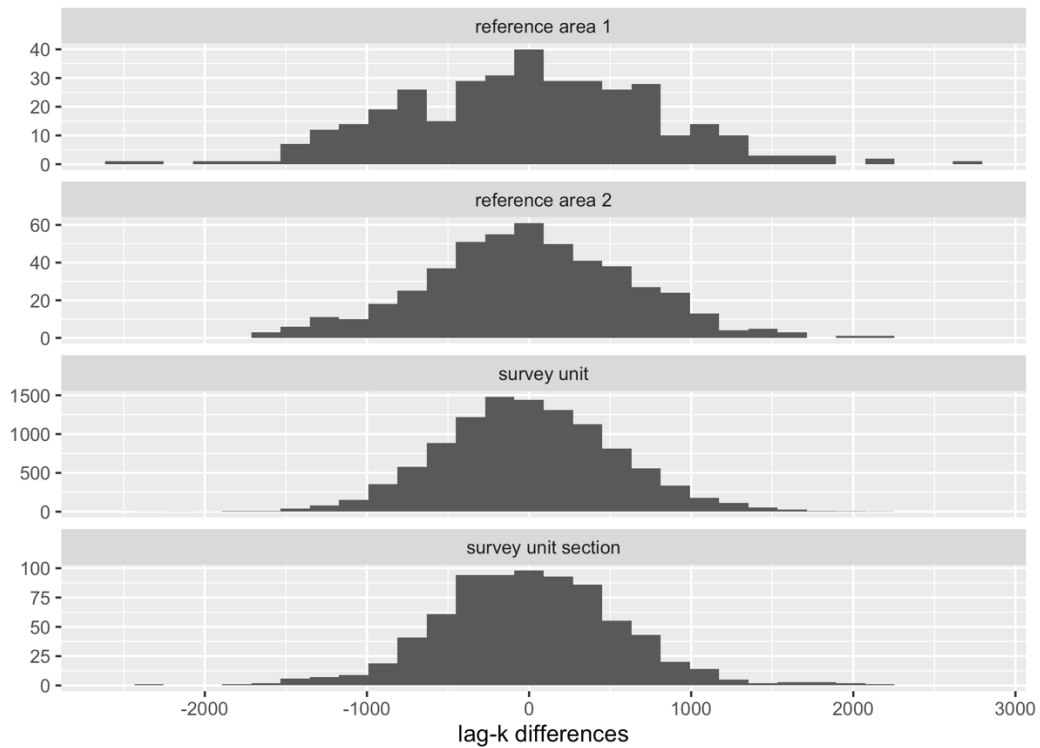
Figure 5.7. Histograms of the lag- k ( k = 20 ) differences from background reference area and survey unit. Reference Areas 1 and 2 correspond to Figures 5.1 and 5.2, respectively. The survey unit and survey unit sections correspond to Figures 5.3 and 5.6, respectively. Note that the histograms are centered at zero, regardless of the distribution location (e.g., mean) in Figures 5.1 through 5.6.
