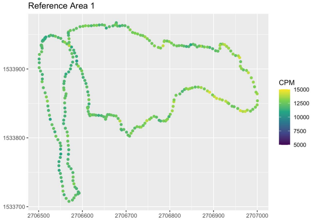
Figure 5.1. Scan survey data from Reference Area 1 with easting on the x-axis and northing on the y-axis.
