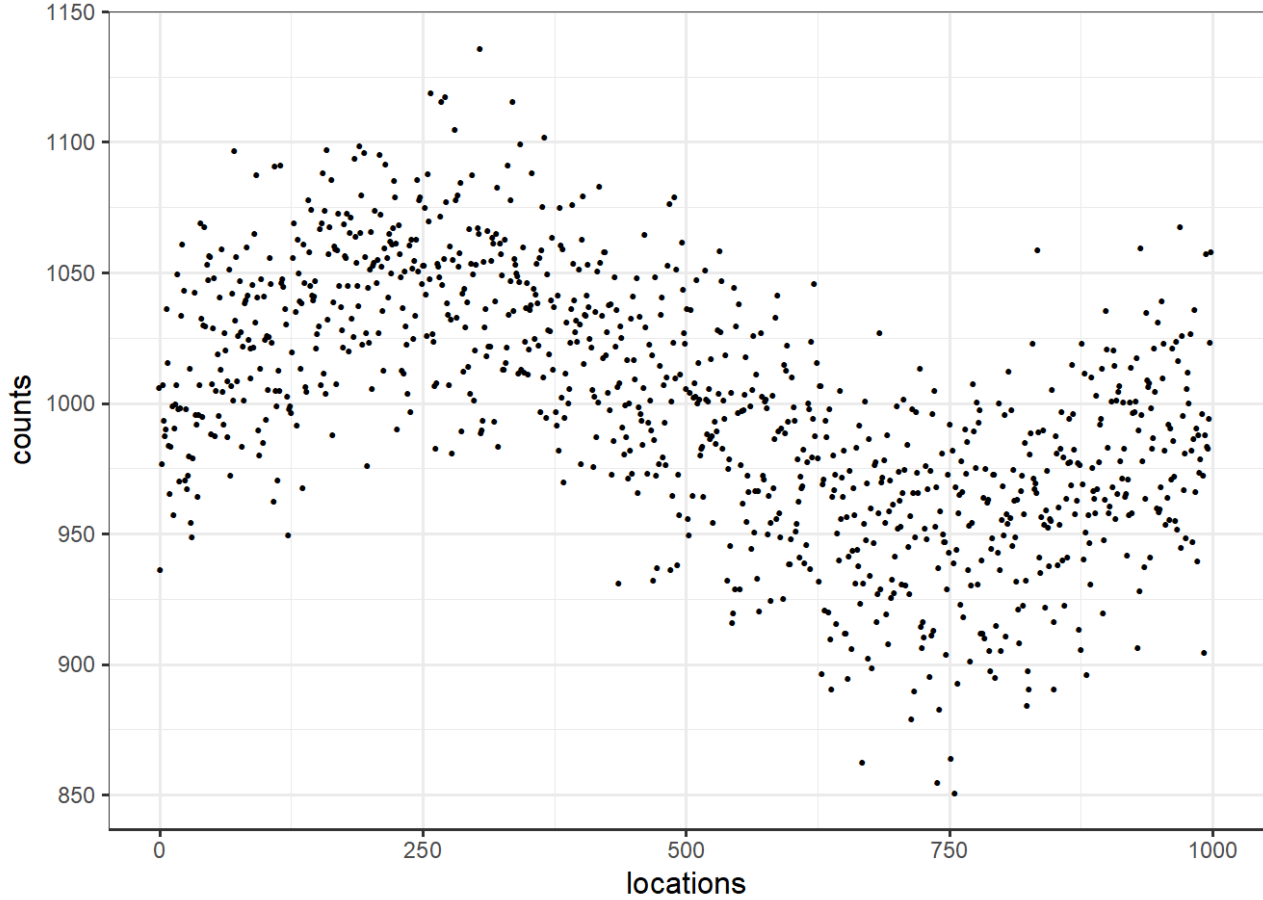
Figure 4.1. Simulated background counts along a transect using a background mean function f(x) = 1000 + 50\sin(2 * \pi * x/1000) , where units of distance between locations are notional.
