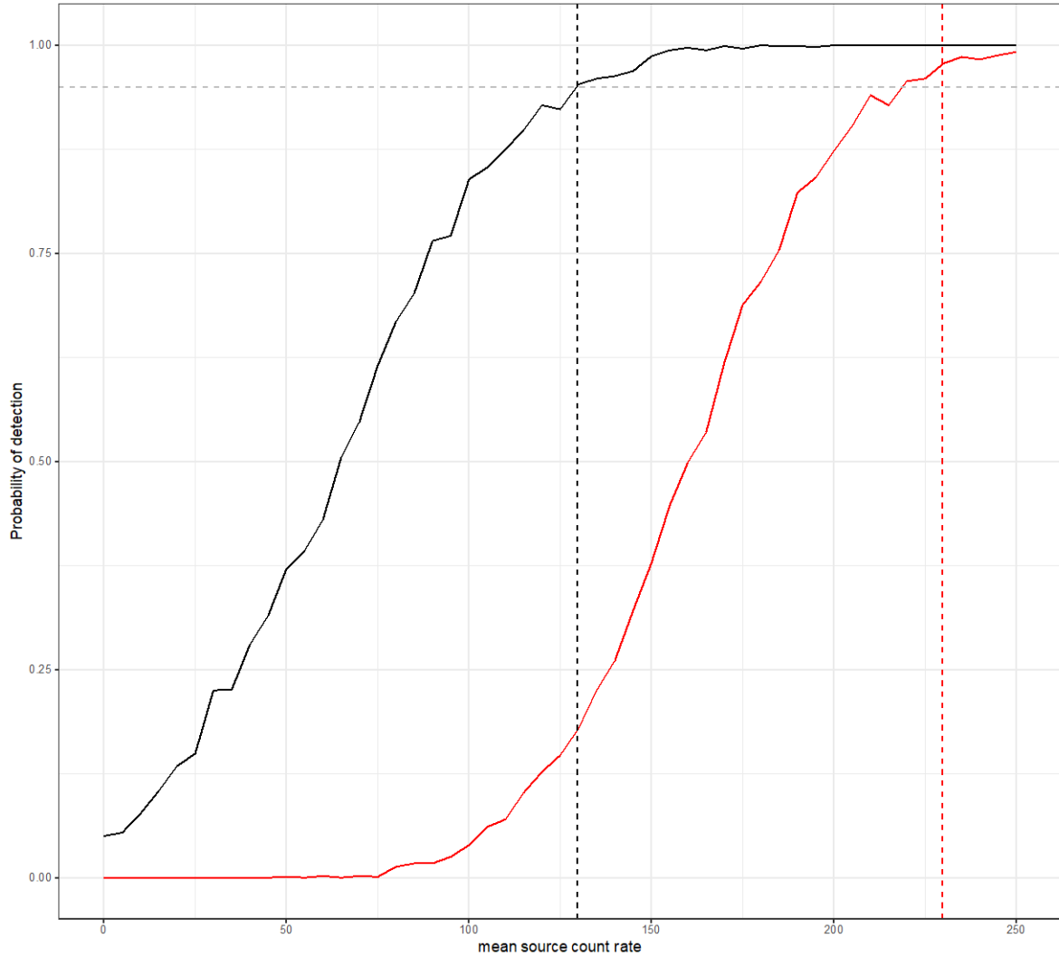
Figure 4.4. Probability of detecting a point source located at the lowest mean background level (location 750 on Figure 4.1) as a function of mean source count rate with variable background. Solid lines represent calculated probabilities of detection using the non-localized hypothesis test (red) and lag- k hypothesis method (black). Each point on the line represents the observed probability of detection (y-axis) for a given mean source count rate (x-axis). The vertical dashed lines are the calculated detection limit for each method. These results are based on 1,000 simulations from a process with non-constant background ( A = 50 ).
