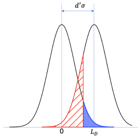
Figure 3.5. Distributions of the null (centered at zero) and alternative (centered at L_D ) hypotheses and the relationship between the detection limit, L_D , and sensitivity index, d' .
