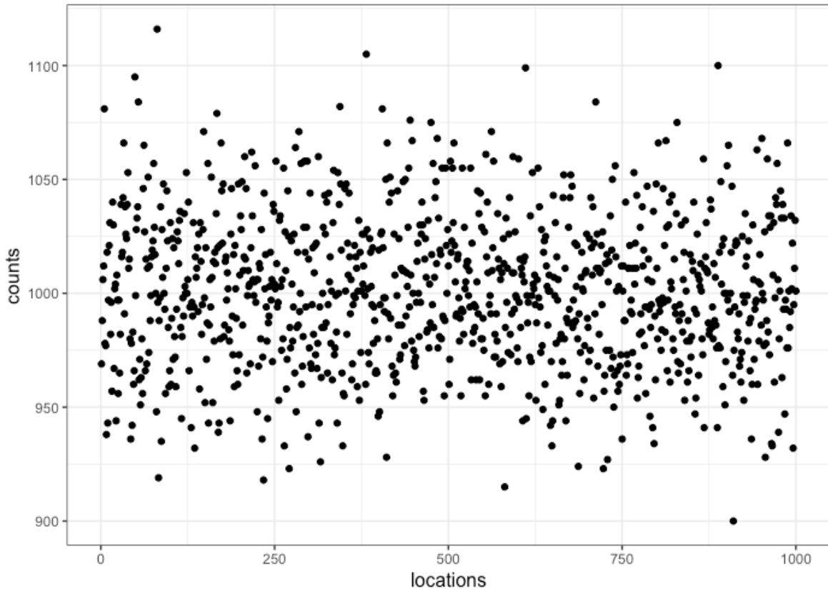
Figure 4.2. Example of simulated data using constant background.
