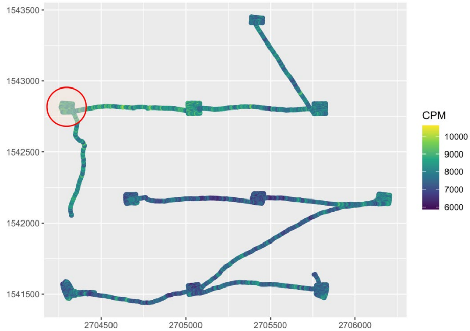
Figure 5.3. Survey unit scan data (in cpm) with easting on the x-axis and northing on the y-axis. The area within the red circle is the sub-area shown in Figure 5.6.
