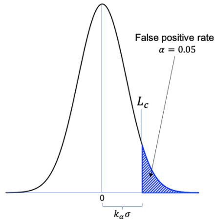
Figure 3.3. False-positive rate, \alpha , and associated critical level, L_c , for a distribution of net counts under the null hypothesis of no net activity.
