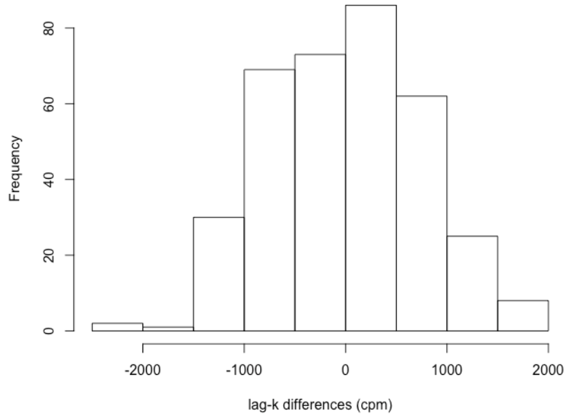
Figure 5.5. Histogram of the lag- k differences using k = 20 for the background reference area data.
