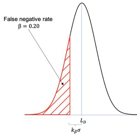
Figure 3.4. False-negative error rate, \beta , and its relationship to the detection limit, L_D .
