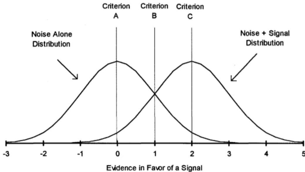
Figure 3.2. The signal detection theory view of signals in noise and decision criteria (from NUREG-CR-6364 [NRC 1998]).
