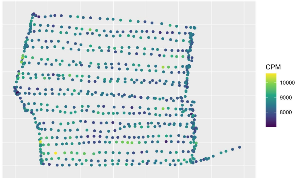
Figure 5.6. One continuously scanned section of the survey unit data (in cpm) with easting on the x-axis and northing on the y-axis. This portion of the survey unit is located in the upper-left region of the survey unit within the red circle in Figure 5.3.
