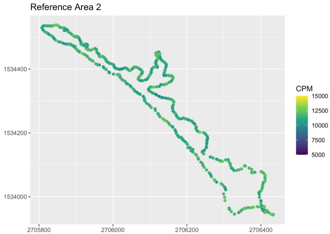
Figure 5.2. Scan survey data from Reference Area 2 with easting on the x-axis and northing on the y-axis.
