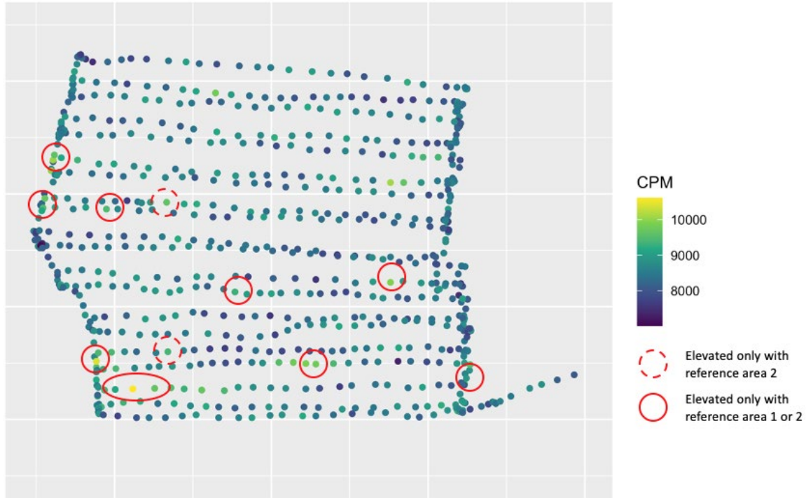
Figure 5.11. Sub-area of survey unit with easting on the x-axis and northing on the y-axis and points identified as greater than local background using lag- k ( k = 20 ) identified in the red circles (also shown in Figure 5.10). Solid red circles indicate points flagged using Reference Area 1 or 2. Dashed red circles indicate points flagged using Reference Area 2 but not Reference Area 1.
