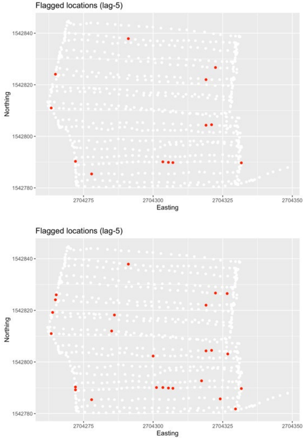
Figure 5.8. Flagged locations (red) indicate observations exceeding the critical level for the reference area 1 (top) and 2 (bottom) and lag- k ( k = 5 ) value, with easting on the x-axis and northing on the y-axis. The critical values used for each plot are listed in Table 2.
