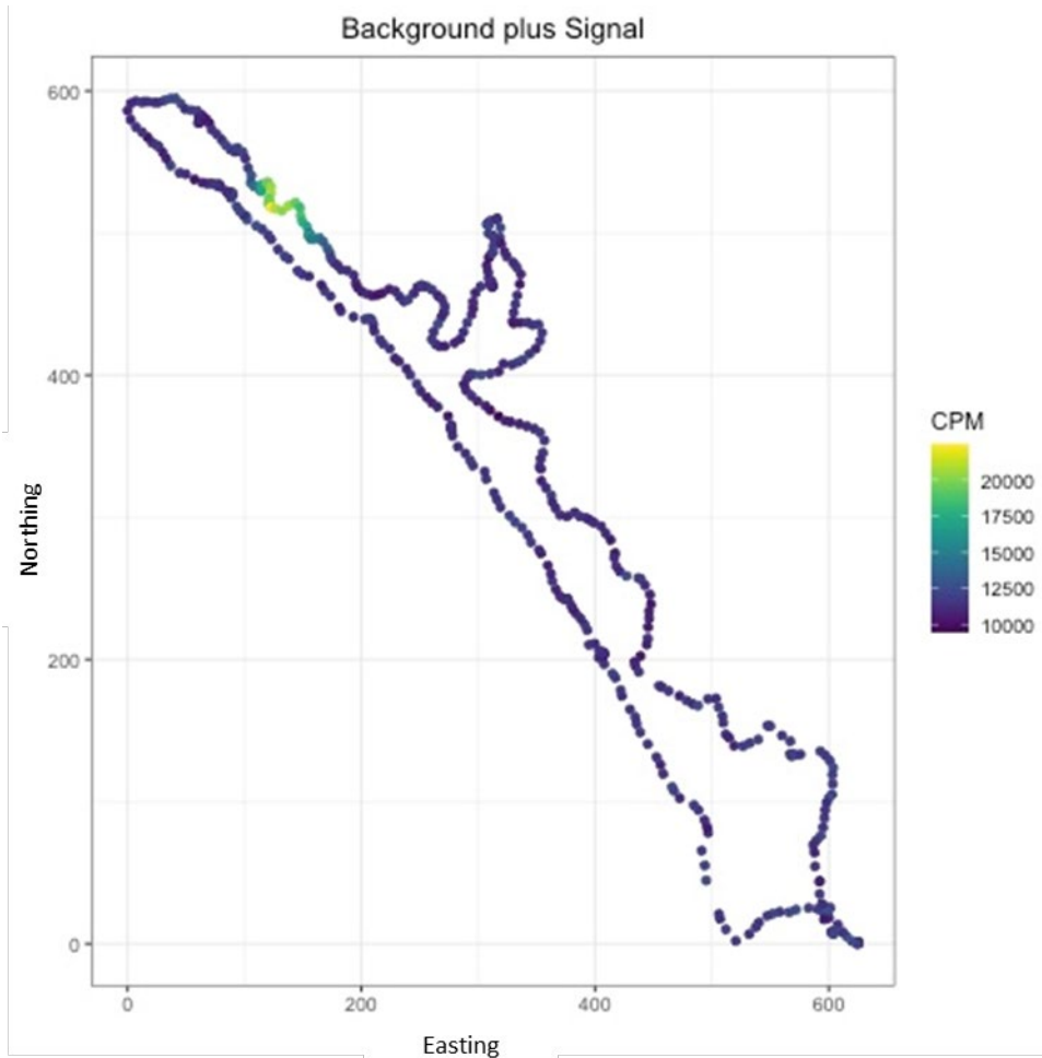
Figure 5.12. Heatmap of observed counts per minute with known inserted signal for Reference Area 2, with easting on the x-axis and northing on the y-axis.
