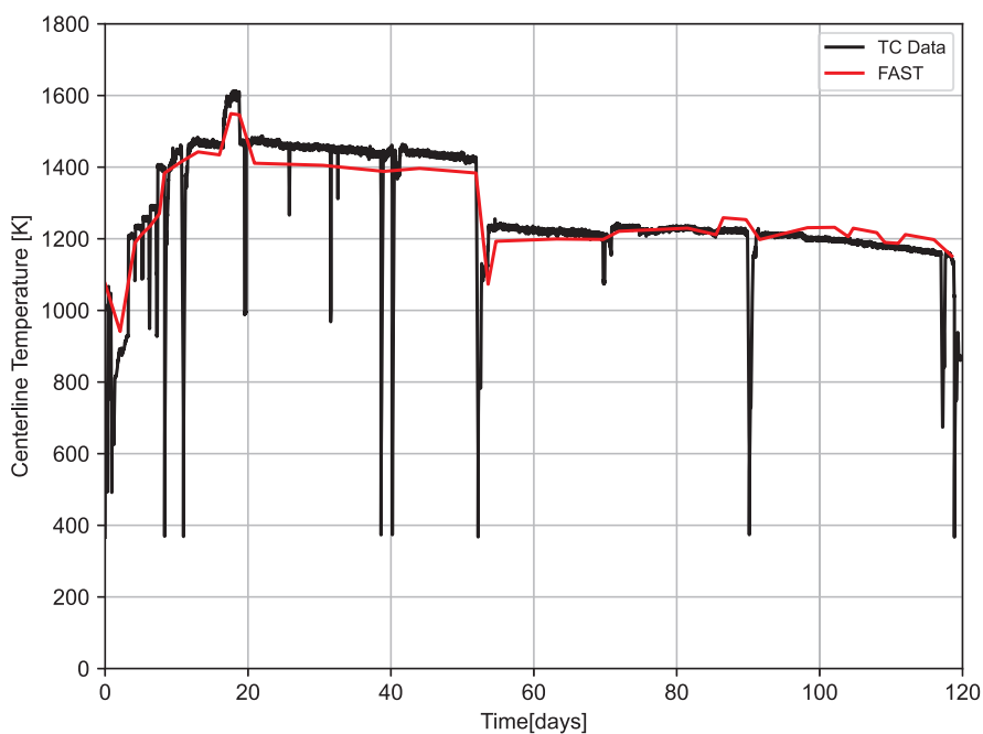
Figure 3-20. Measured and predicted centerline temperature for IFA-629.1 rod 1 (MOX) (starting burnup = 27 GWd/MTU, ending burnup=33 GWd/MTU, as-fabricated radial gap = 84 \mu m)
