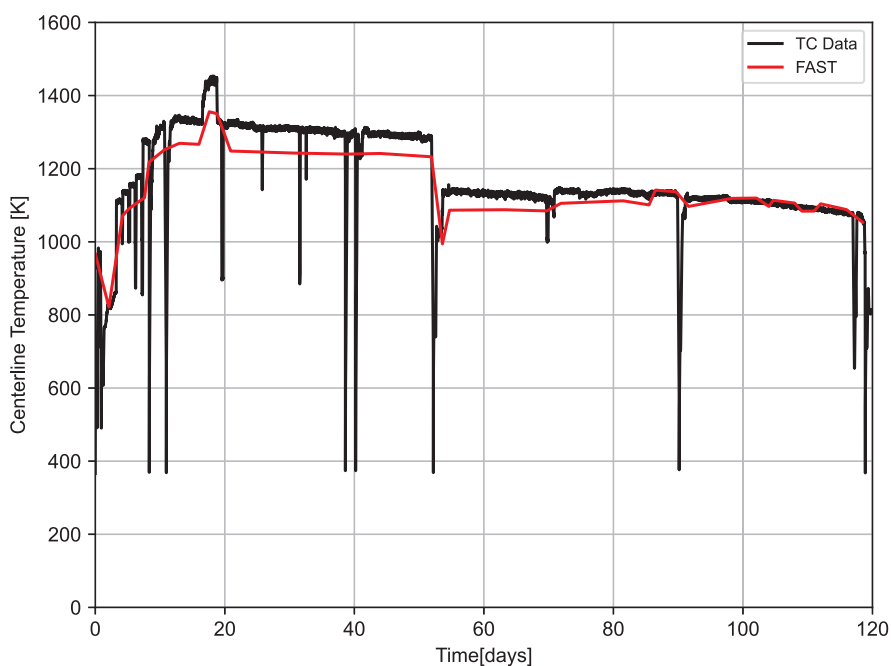
Figure 3-21. Measured and predicted centerline temperature for IFA-629.1 rod 2 (starting burnup = 29 GWd/MTU, ending burnup = 40 GWd/MTU, as-fabricated radial gap = 84 \mu m)
