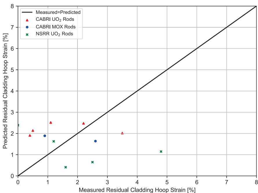
Figure 8-1. FAST-1.2 predictions of residual cladding hoop strain for CABRI and NSRR \text{UO}_2 and MOX rods
