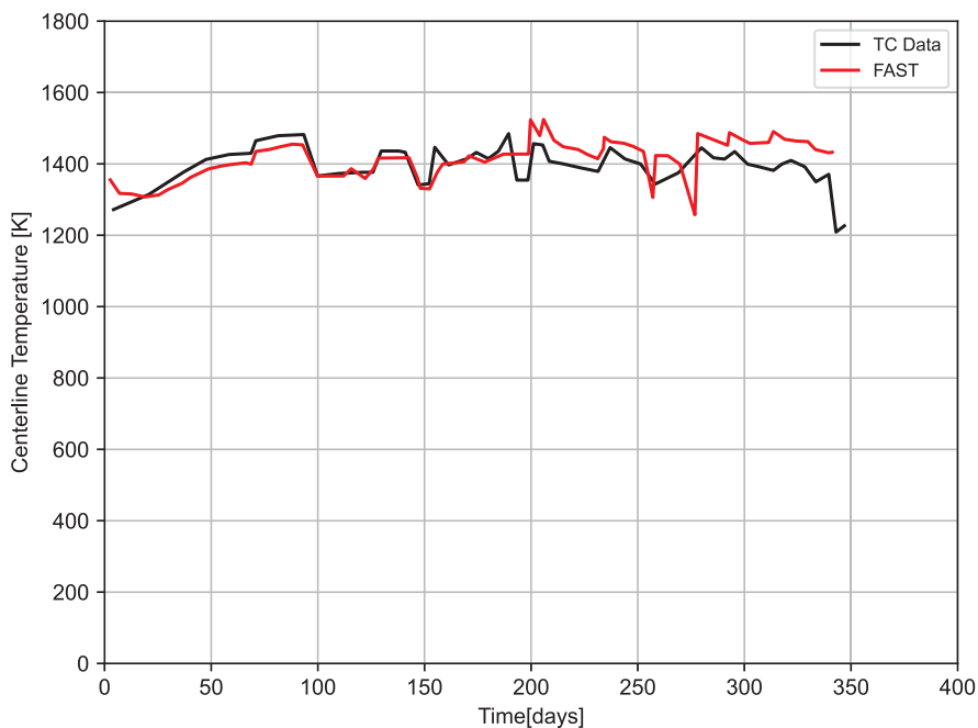
Figure 3-14. Measured and predicted centerline temperature for IFA-681 rod 1 \text{UO}_2 (burnup = 33 GWd/MTU, as-fabricated radial gap = 85 \mu\text{m} )
