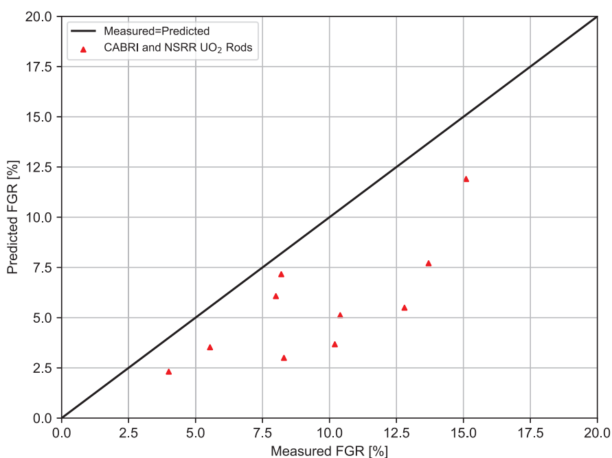
Figure 8-2. FAST-1.2 Predictions of RIA FGR for CABRI and NSRR \text{UO}_2 Rods
