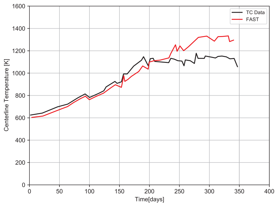
Figure 3-43. Measured and predicted centerline temperature for IFA-681 rod 3 ( \text{UO}_2\text{-8\% Gd}_2\text{O}_3 ) (burnup = 12 GWd/MTU, as-fabricated radial gap=85 \mu\text{m} )
