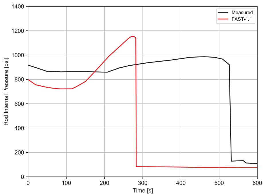
Figure 9-4. FAST-1.1 predicted and measured rod internal pressure for IFA-650.6
