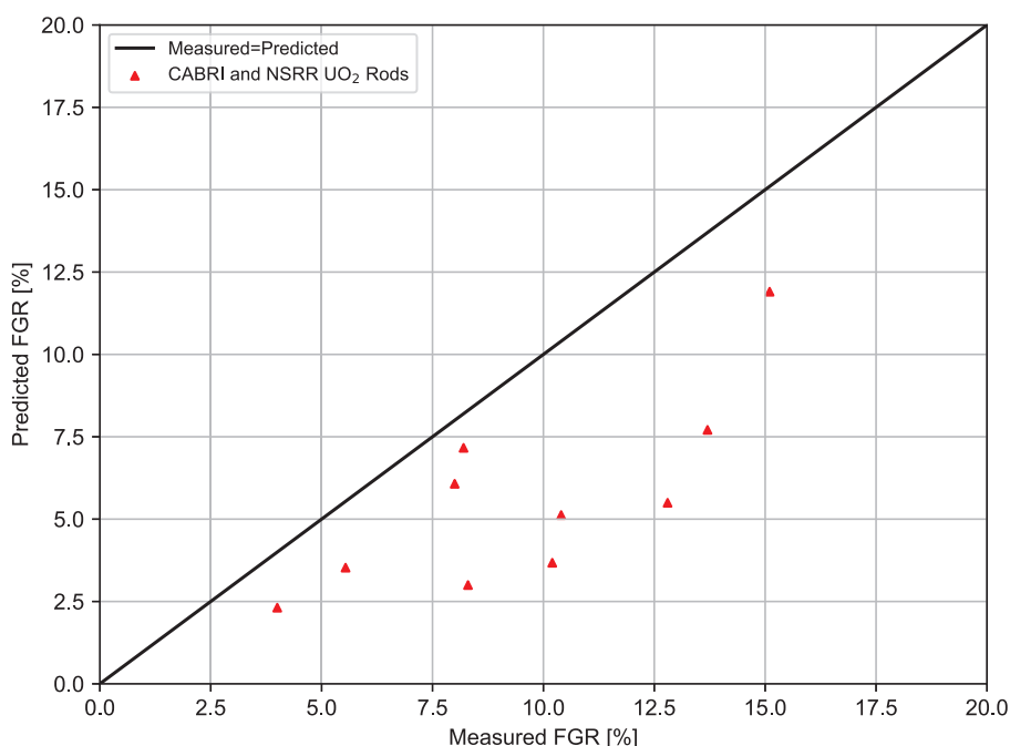
Figure 8-2. FAST-1.1 Predictions of RIA FGR for CABRI and NSRR UO 2 Rods
