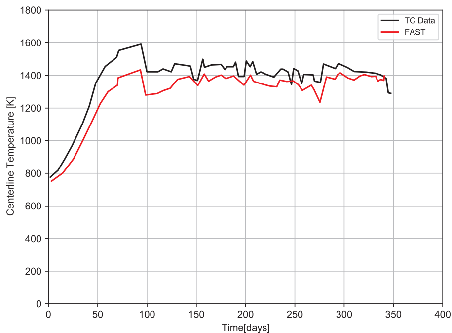
Figure 3-44. Measured and predicted centerline temperature for IFA-681 rod 4 ( \text{UO}_2\text{-2\% Gd}_2\text{O}_3 ) (burnup = 22 GWd/MTU, as-fabricated radial gap = 85 \mu\text{m} )
