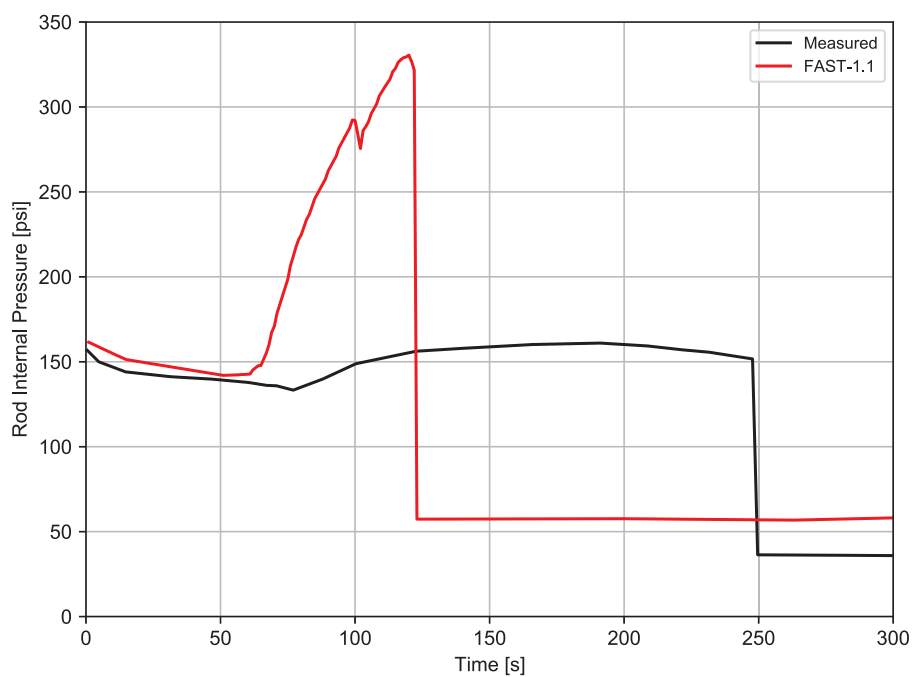
Figure 9-5. FAST-1.1 predicted and measured rod internal pressure for IFA-650.7
