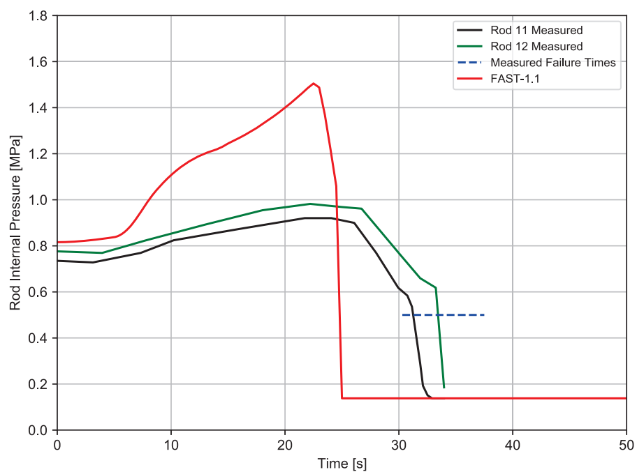
Figure 9-2. FAST-1.1 predicted and measured rod internal pressure for TREAT FRF-2 rods. Solid lines show pressure for two rods. Dashed line shows failure time range for all 7 rods.
