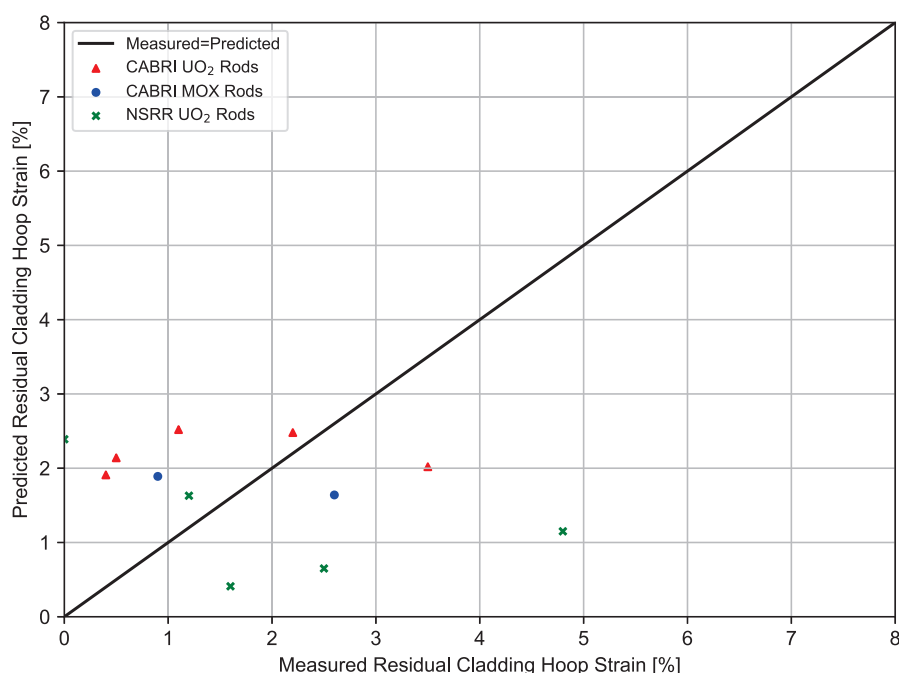
Figure 8-1. FAST-1.1 predictions of residual cladding hoop strain for CABRI and NSRR \text{UO}_2 and MOX rods
