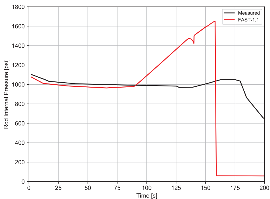
Figure 9-3. FAST-1.1 predicted and measured rod internal pressure for IFA-650.5
