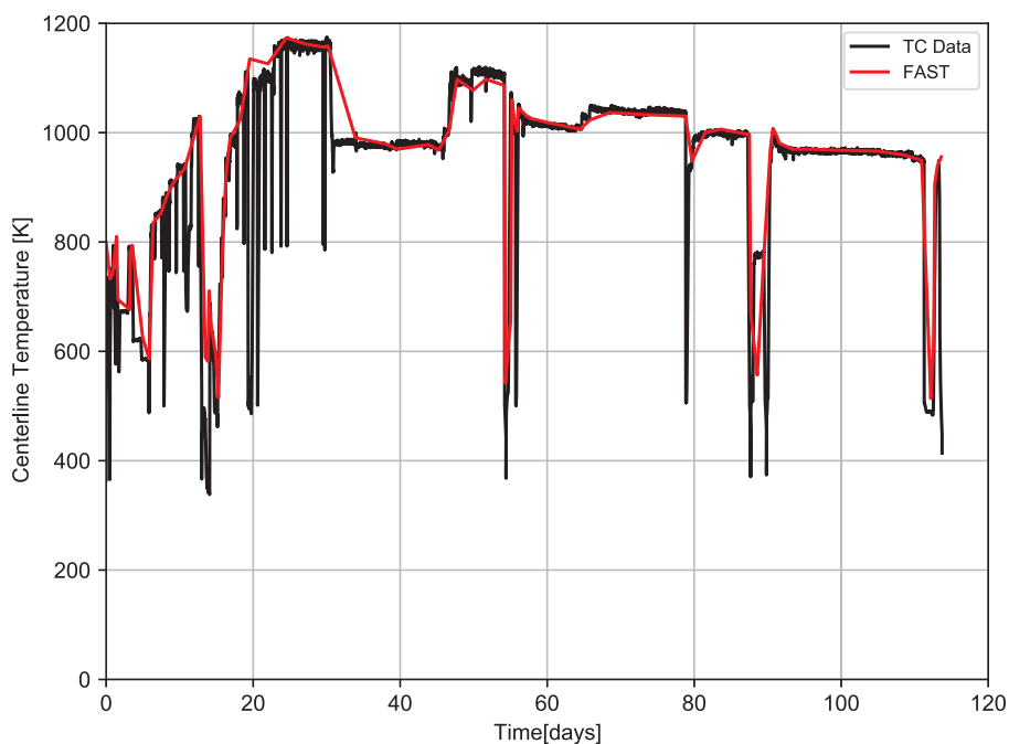
Figure 3-26. Measured and predicted centerline temperature for IFA-629.3 rod 5 (MOX) (starting burnup = 62 GWd/MTU, ending burnup = 72 GWd/MTU, as-fabricated radial gap = 84 \mu m)
