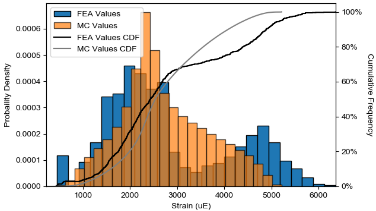
Figure 5.3. Distributions of MC and FEA simulation outputs.
