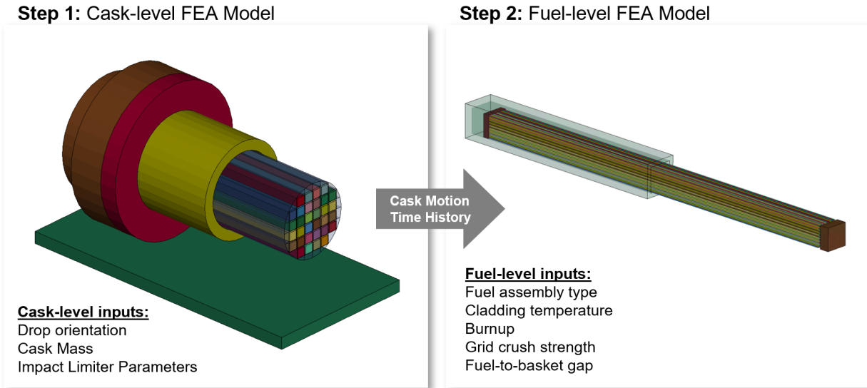
Figure A.1. Overview of FEA models used in this work. Models have been sectioned for illustrative purposes.
