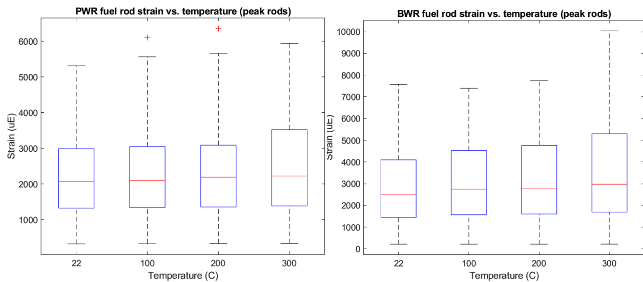
Figure D.4. Box plots of peak cladding strain versus temperature.
