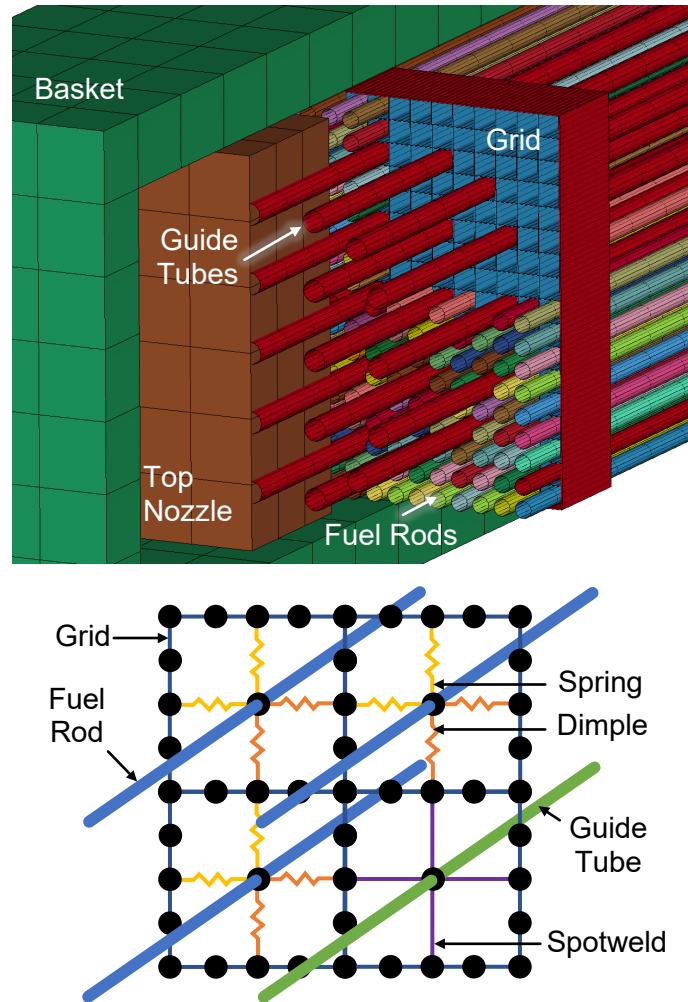
Figure B.1. Detail of the PWR model (top) and illustration of grid model (bottom). Some components have been hidden or sectioned for illustrative purposes.
