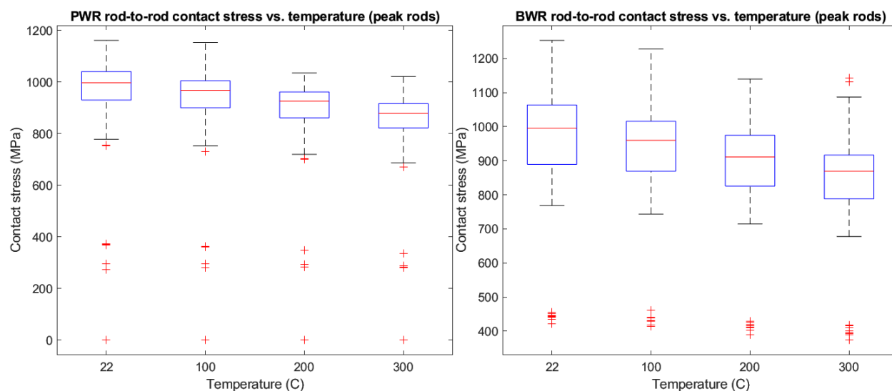
Figure D.12. Box plots of rod-to-rod contact stress versus temperature.
