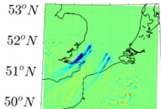
WRF shows wind farm wakes
