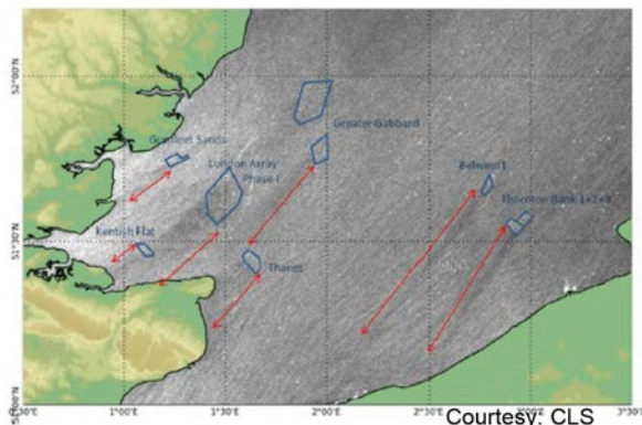
Satellite SAR shows wind farm wakes
