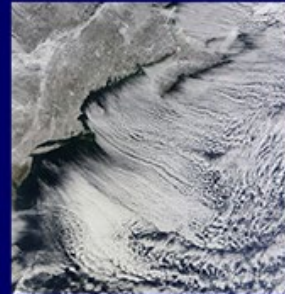
Horizontal roll vortices or “Cloud streets” with Convection
