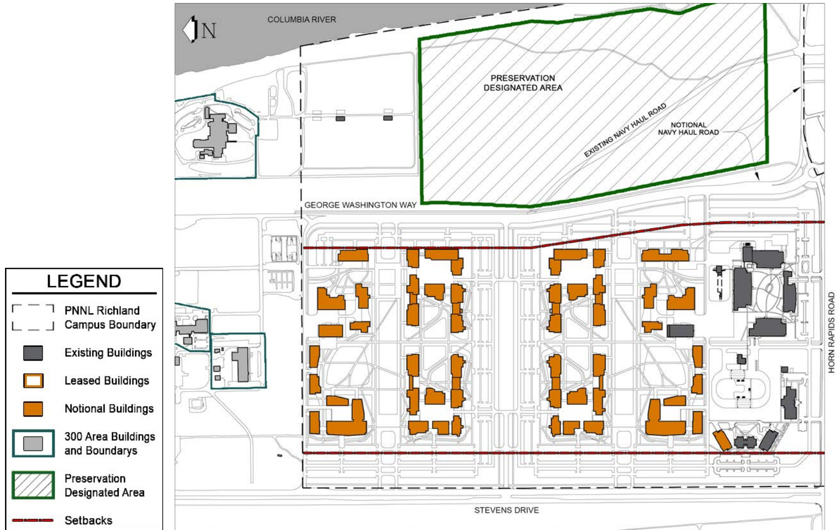
Figure 4.10. Building setbacks
