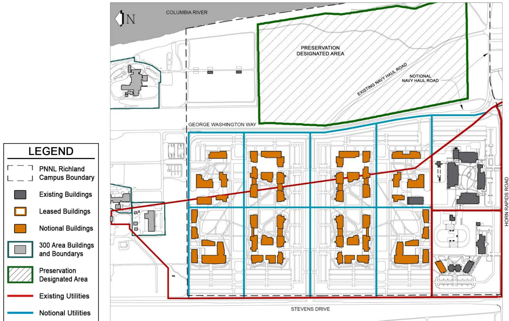
Figure 3.4. Utilities infrastructure and distribution systems corridors
