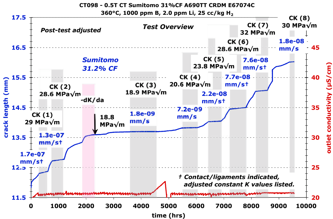
Figure 142. Overview of the entire SCC test on the 31%CF Sumitomo E67074C specimen CT098 showing crack growth rate at the different stress intensity levels.
