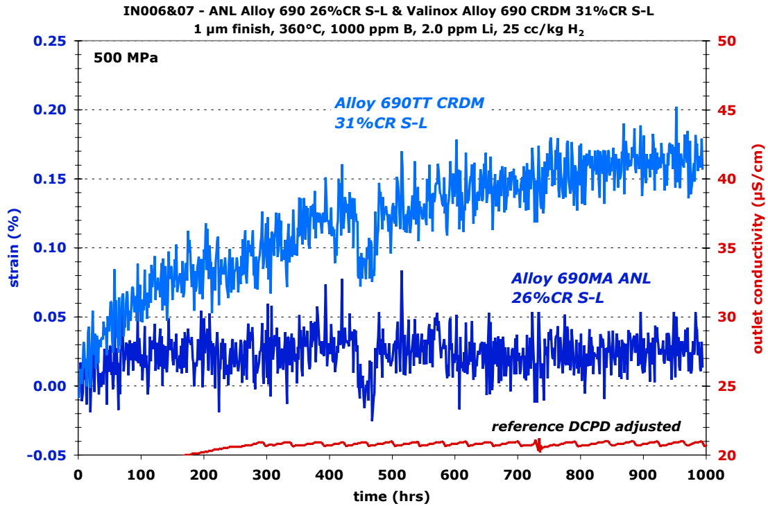
Figure 75. DCPD-based strain response for specimens IN006 and IN007 during the first 1000 hours of testing.
