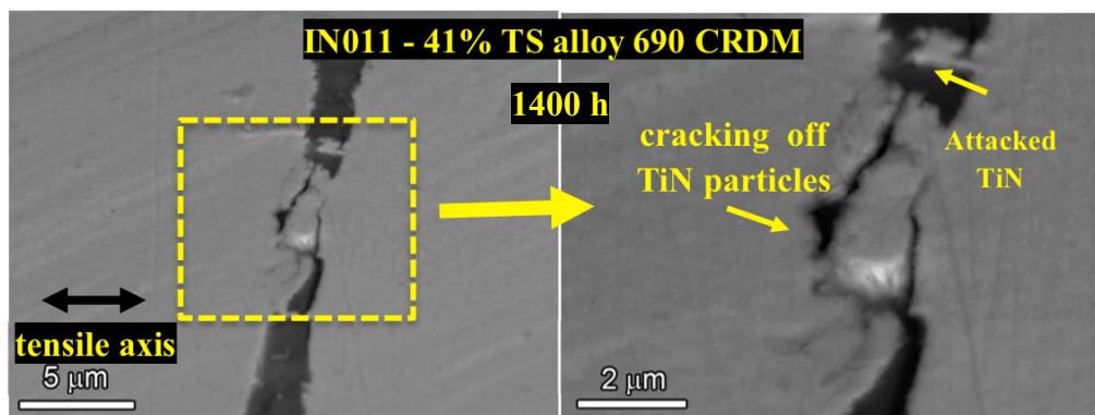
Figure 118. SEM-BSE images of the surface of 41% tensile strained alloy 690 CRDM specimen IN011. Corrosion and cracking of TG TiN particles was observed.
