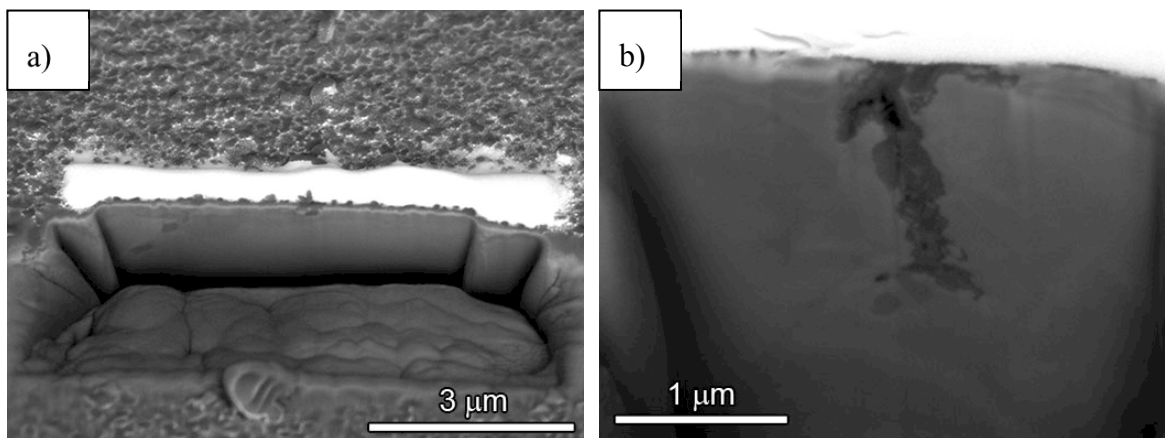
Figure 11. SEM (BSE) micrographs of FIB trenches cut across a) a grain boundary and b) a crack in an alloy 690 sample. The size of the trench is significantly wider than any observed cracking.
