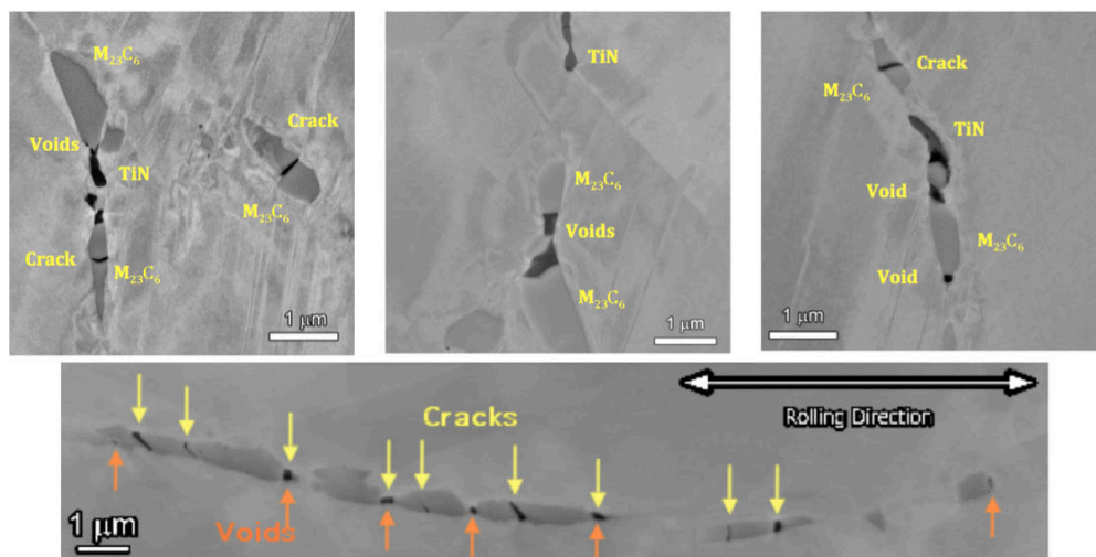
Figure 72. SEM-BSE images of the ANL 26%CR alloy 690MA plate material showing voids and cracked carbides on grain boundaries in this material.
