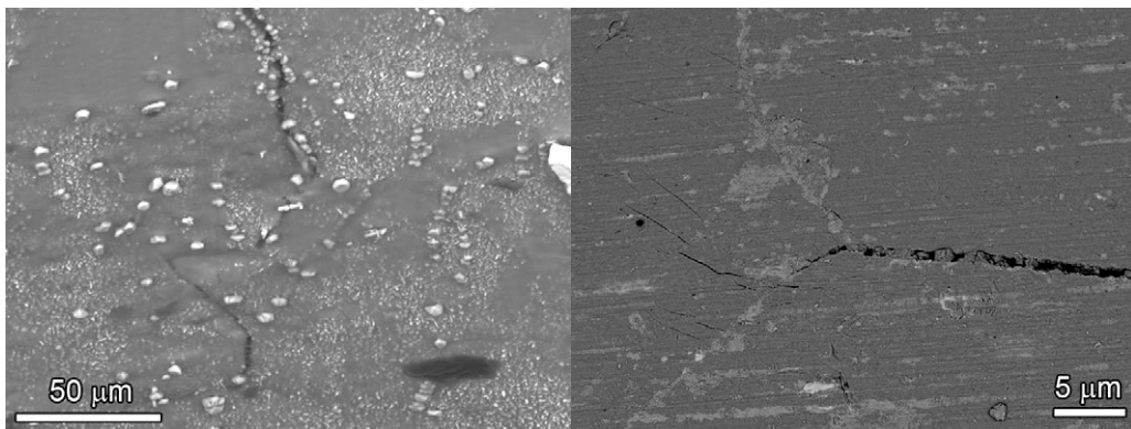
Figure 130. Higher magnification SEM-SE images showing cracks on the notch surface of the 31%CF Valinox CRDM specimen c672.
