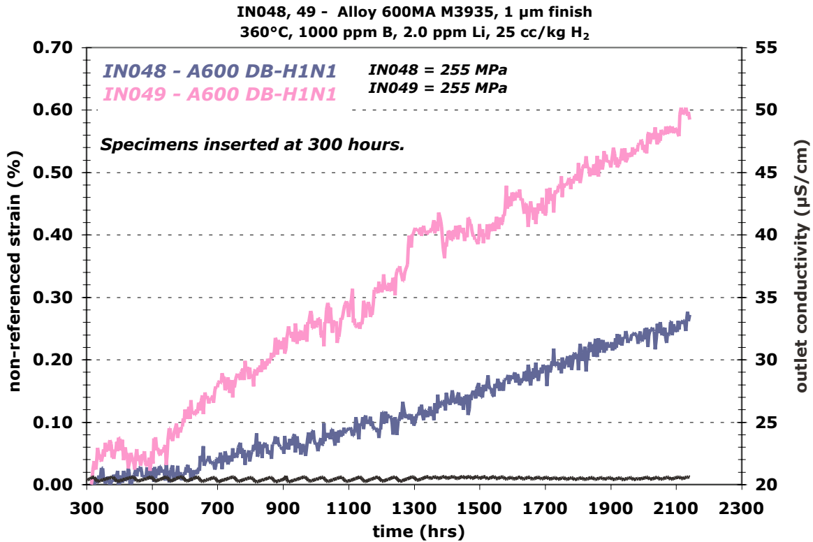
Figure 63. DCPD response for the two instrumented alloy 600 CRDM specimens from PWR service (IN048 and IN049) during their first exposure in 360°C PWR primary water for 1840 hours.
