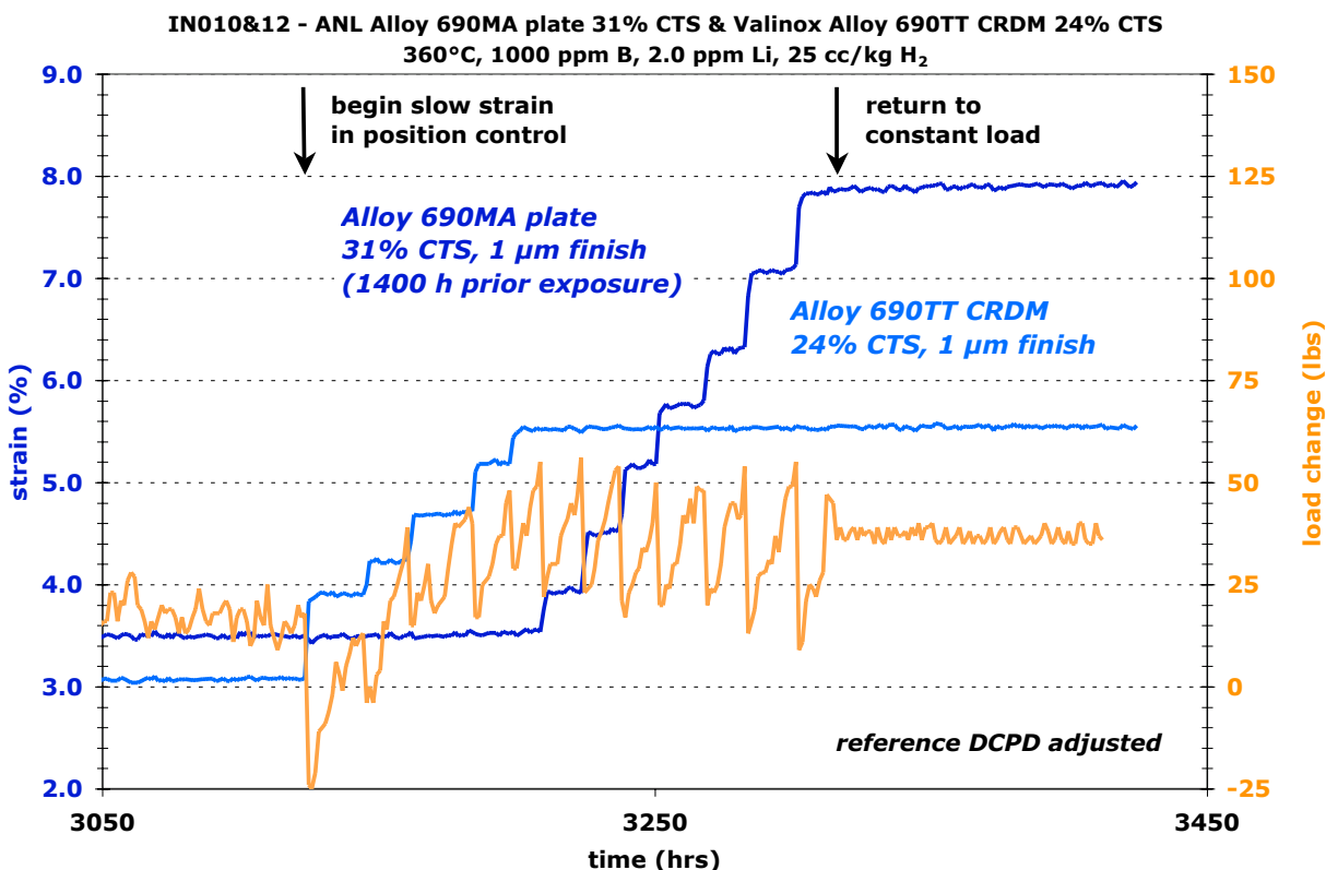
Figure 122. Slow straining response of the 31%TS alloy 690 plate (IN010) combined with a 24%TS alloy 690 CRDM specimen (IN012). Note that IN010 has 1400 hours of prior exposure.
