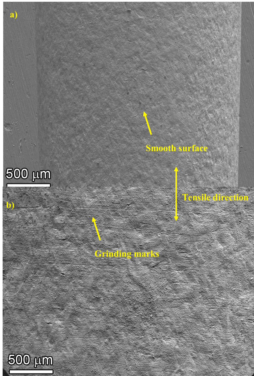
Figure 35. SEM-SE images of exposed surfaces for the alloy 600 initiation specimens that had a) highly polished gage section surface (IN003) or b) surfaces polished to 1 \mu\text{m} and then ground with 1200 grit SiC ground gage section surface (IN002).
