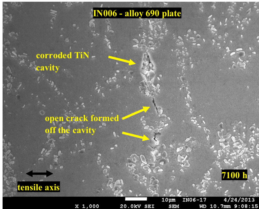
Figure 85. Example of surface crack morphology in the 26%CR plate specimen (IN006) after ~7100 hours of exposure.
