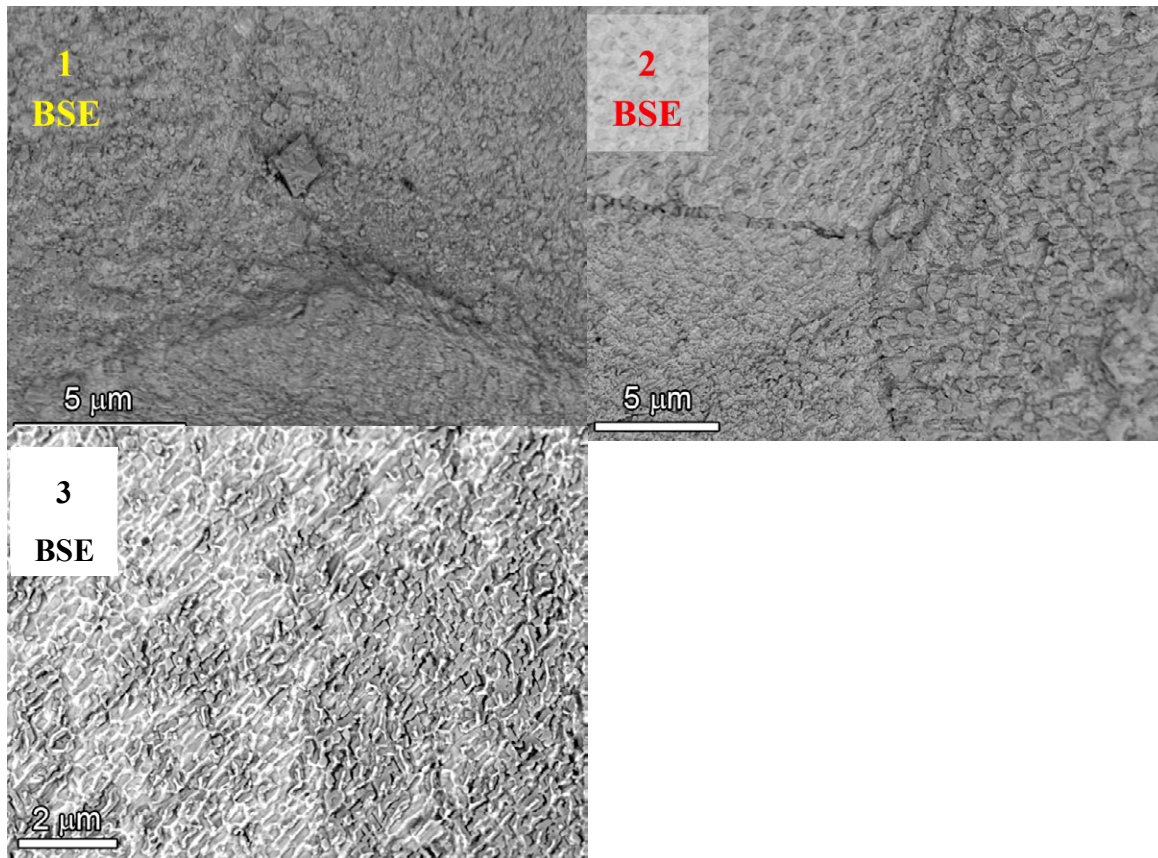
Figure 103. High magnification SEM-BSE images of IG cracking of various regions denoted in Figure 101.
