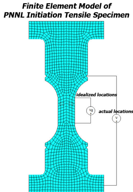
Figure 4. 2D representation of the axisymmetric finite element model. Actual gauge spot-weld locations versus idealized gauge spot weld locations are shown.
