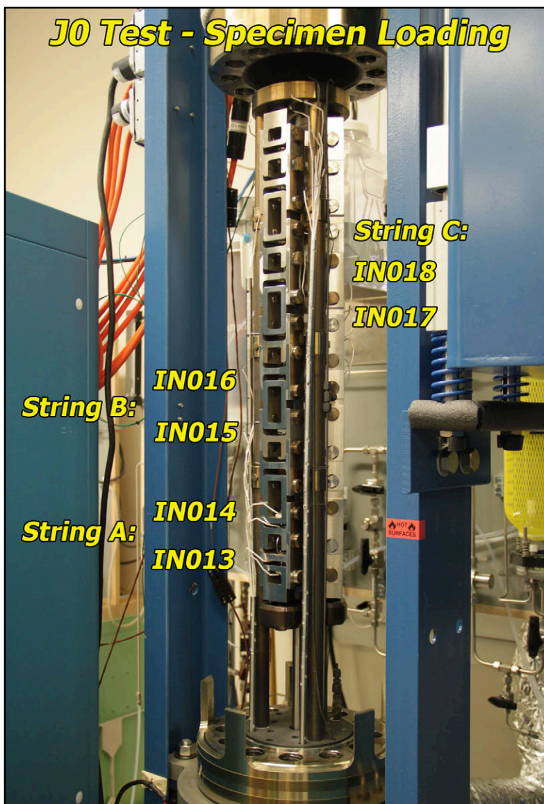
Figure 37. Load train for the LWR system #1 crack initiation test system set up for the demonstration test.
