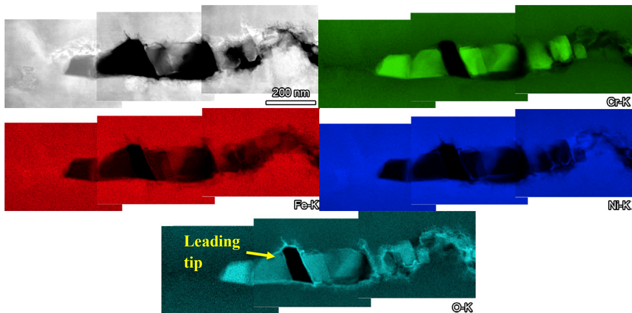
Figure 112. High magnification TEM angular DF and EDS elemental map montages crack #1 (see Figure 105).
