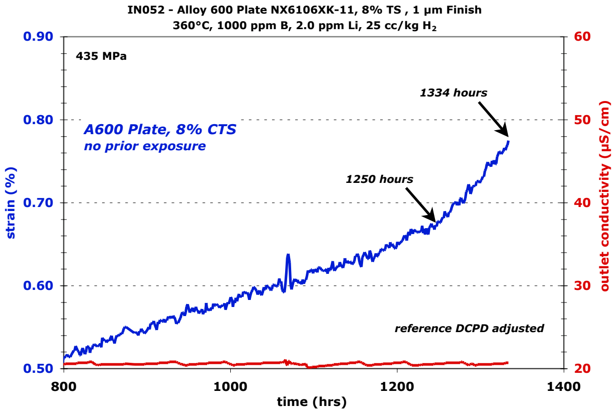
Figure 57. SCC initiation plot for the 8%TS alloy 600 specimen IN052 revealing evidence for crack nucleation at ~1250 hours.
