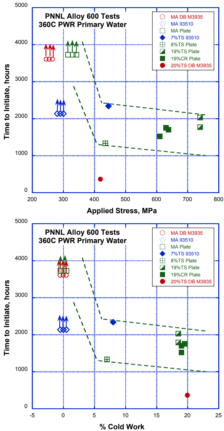
Figure 66. Summary of PNNL SCC initiation test results for alloy 600 heats showing no failures for as-received materials at applied stresses below ~400 MPa. All specimens were tested at their yield strength.
