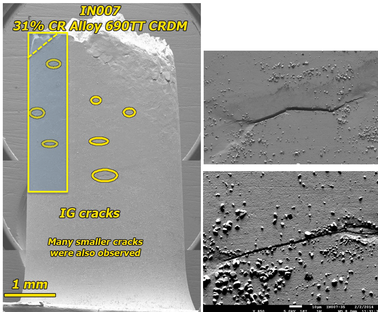
Figure 104. SEM-SE images from the gauge surface of the 31%CR CRDM specimen IN007. The yellow box indicates where a cross-section sample was prepared. The dotted line indicates a portion of the cross-section slice that was removed to due to necking damage.
