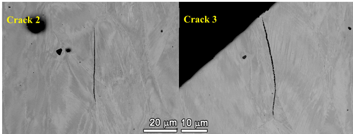
Figure 109. SEM-BSE images showing low magnification images of crack #2 and #3.
