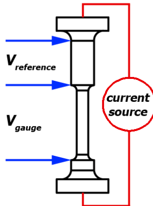
Figure 3. Schematic of the ideal DCPD measurement points on the tensile geometry.
