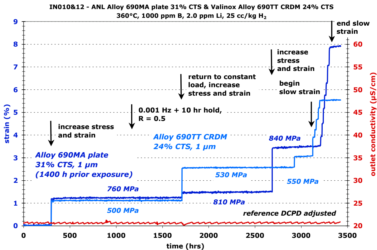
Figure 121. Overview of the entire test on the 31% tensile strained alloy 690 plate (IN010) combined with a 24% cold tensile strained alloy 690 CRDM specimen (IN012). Note that IN010 has 1400 hours of prior exposure.
