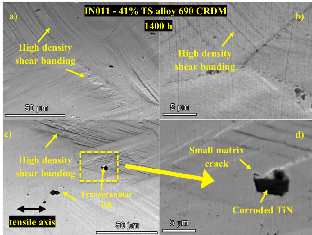
Figure 117. SEM-BSE images of the surface of 41% tensile strained alloy 690 CRDM specimen IN011 showing high levels of shear banding. No apparent IG crack initiation was observed. Representative grain structures are shown in a) and b). Corrosion and cracking of TG TiN particles was observed (c-d).
