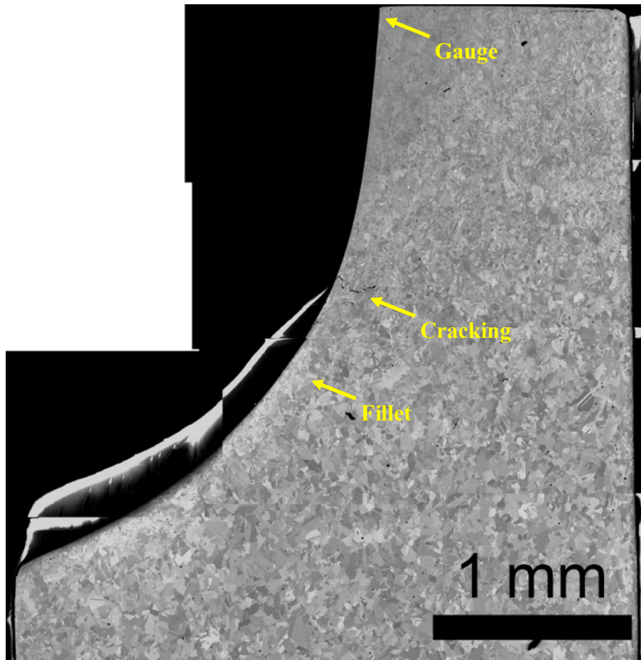
Figure 31. SEM (BSE) images of a cross-section from the alloy 600 tensile initiation specimen IN003 that exhibited cracking near the fillet. Note that strain contrast in the gauge section obscures the grain morphology.
