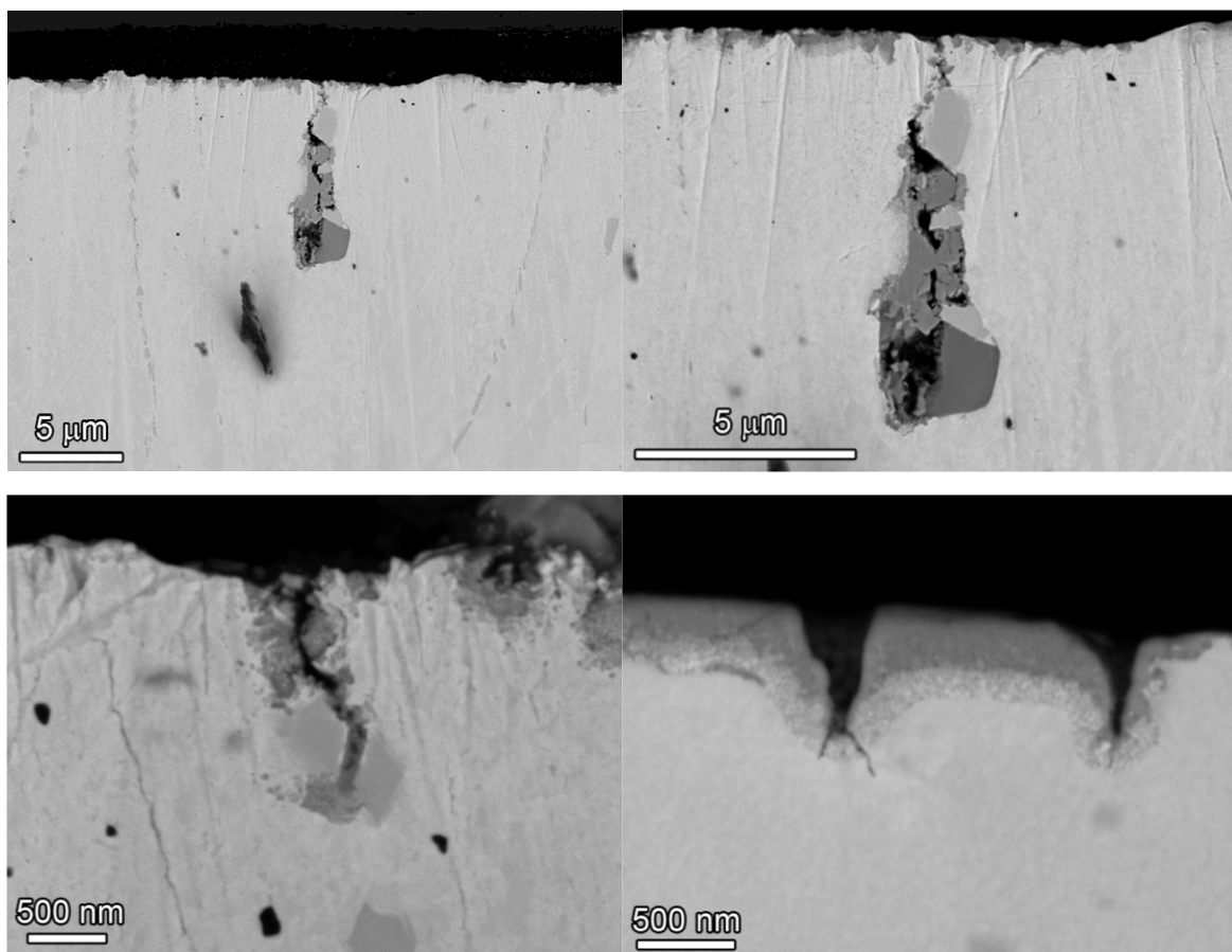
Figure 97. SEM-BSE images of IN006 cross-section after 9144 h.
