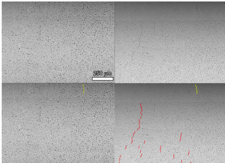
Figure 54. SEM-BSE images of IN023 Rotation #1 illustrating the extent of surface crack formation at 1713 hours (left) and 2591 hours (right). Upper and lower images are identical. In the lower images, present cracks that were present after 1713 hours are yellow while those found after 2591 hours are red.
