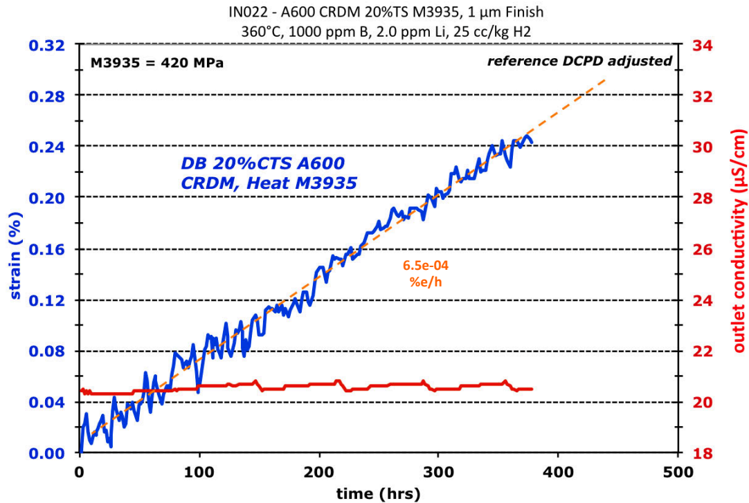
Figure 47. Strain versus time plot for specimen IN022 showing a steadily increasing strain during test in 360°C PWR primary water.
