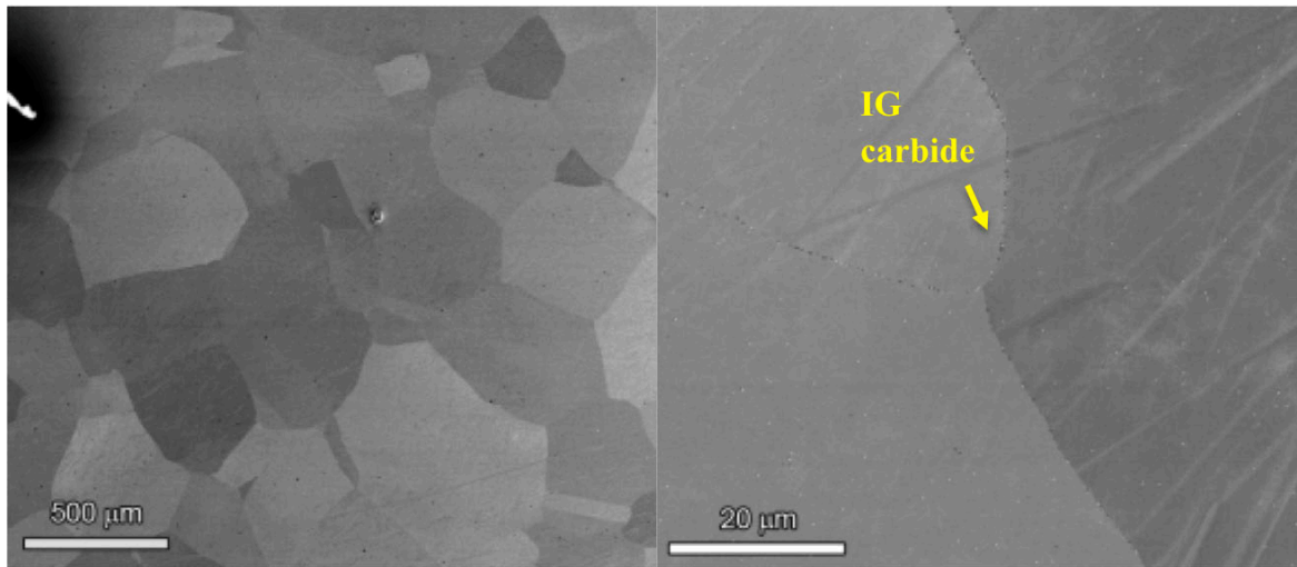
Figure 15. SEM (BSE) images illustrating the general microstructure and large grain size in the mill-annealed alloy 600 CRDM heat M3935 material.
