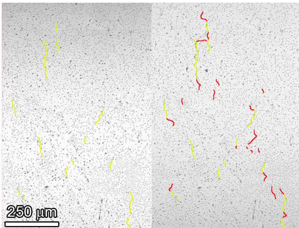
Figure 10. SEM (BSE) micrographs of the surface of an alloy 600 tensile specimen between two exposures (left 1870 hours and right 2750 hours). The presence of cracks at 1870 hours is highlighted in yellow and new cracks and crack extensions at 2750 hours are highlighted in red.
