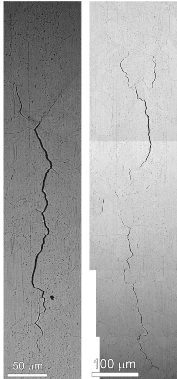
Figure 58. SEM-BSE images of the two primary IGSCC cracks identified on the IN052 gauge.
