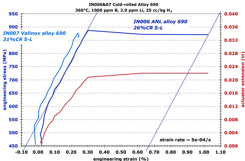
Figure 92. Plastic strain applied to the 26%CR ANL alloy 690 plate specimen IN006 at ~7600 h.
