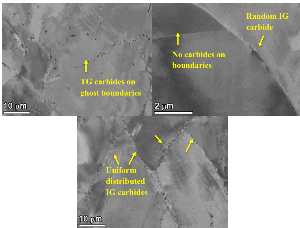
Figure 26. SEM (BSE) micrographs illustrating the microstructure of plate material NX6106XK-11 and the intergranular nature of the carbides.
