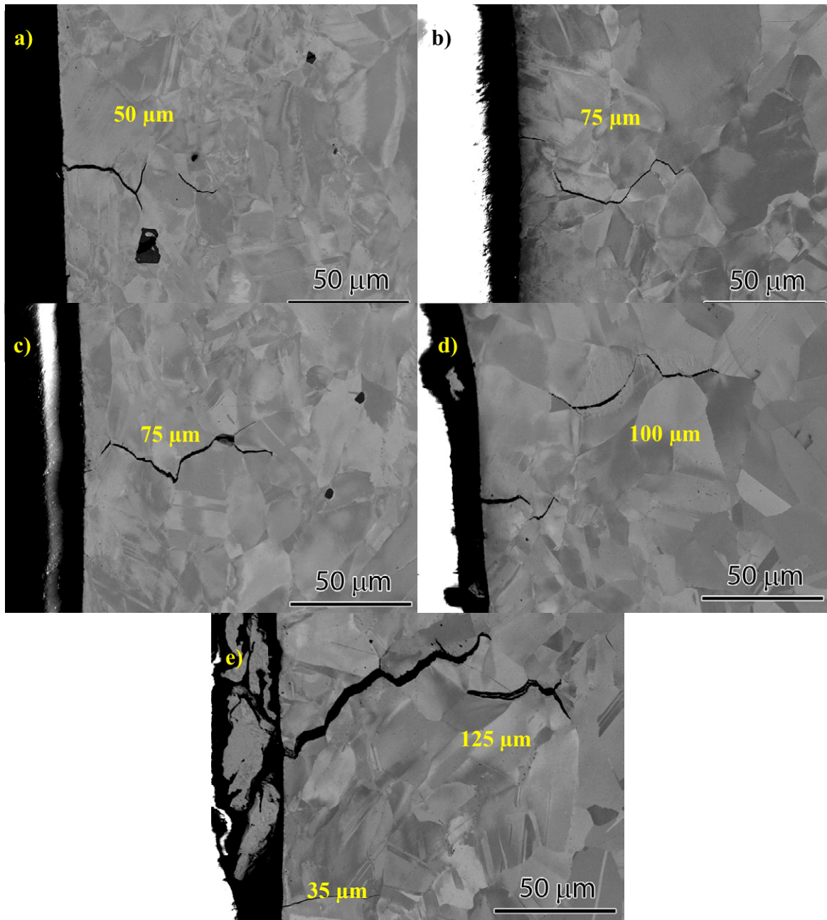
Figure 32. SEM-BSE images of a cross-section for the alloy 600 tensile initiation specimen IN003 showing deep SCC cracks initiating from the surface. Apparent crack depths are listed for each figure.
