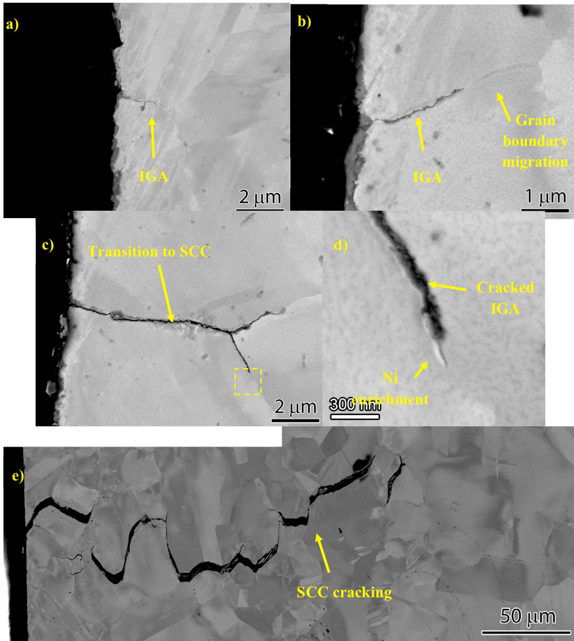
Figure 34. SEM-BSE images of the cross-section for the alloy 600 initiation specimen IN003 highlighting various stages of SCC cracking: (a,b) IG attack in gauge section without cracks, (c,d) IG attack transitioning to an IGSCC crack and e) a long IGSCC crack in the fillet region.
