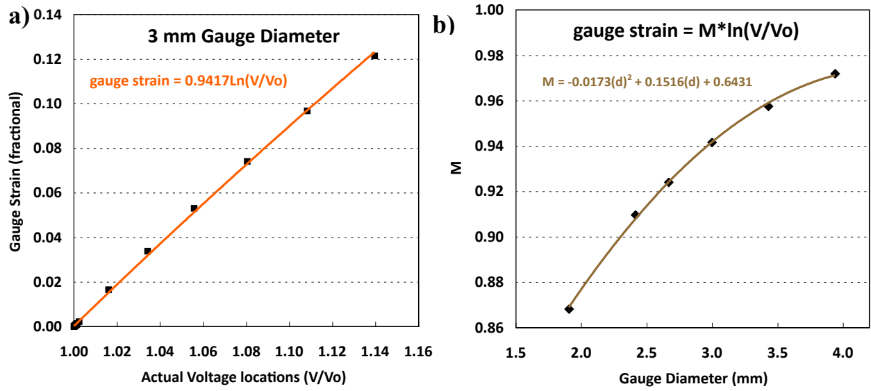
Figure 5. Results of finite element simulations to determine the relationship between strain and voltage measured from the actual locations on the specimen as shown in Figure 4.
