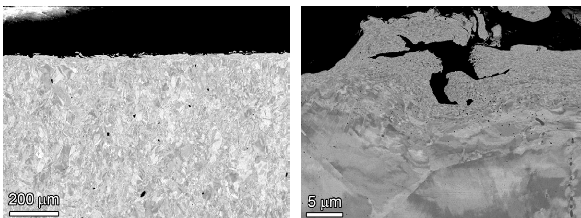
Figure 13. SEM (BSE) micrographs of the cross-section of an alloy 600 miniature tensile specimen ground using a rotary tool (left) and the edge of a SiC blade attachment (right).
