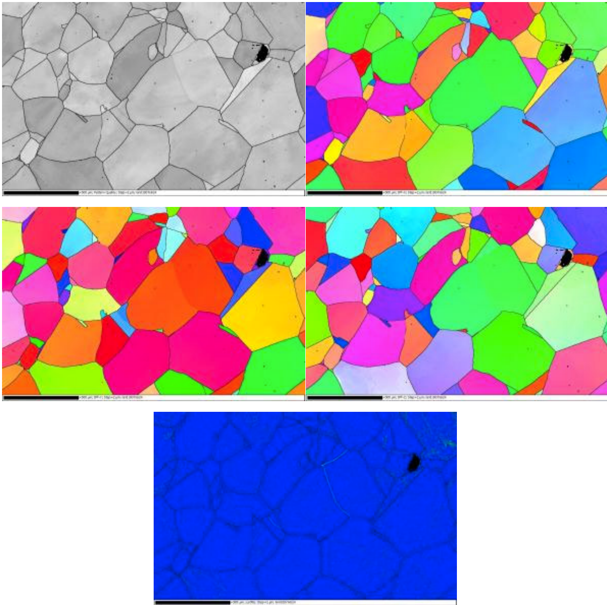
Figure 17. EBSD pattern quality map is shown in upper left image, inverse pole figure maps in upper right (X orientation), middle left (Y orientation) and middle right (Z orientation) images along with misorientation density map in bottom center for Davis Besse heat M3935.
