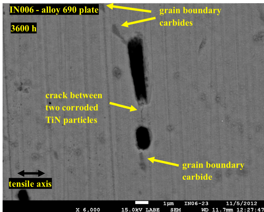
Figure 79. SEM-BSE image showing a crack between two corroded TiN particles that appears to be on a grain boundary in the 26%CR plate specimen IN006 after 3600 h.
