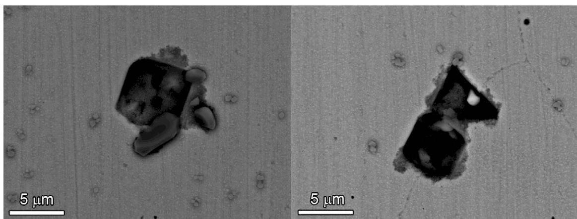
Figure 98. SEM-BSE images of IN007 surface at 9144 h showing two TiN inclusions, one TG (left) and one IG (right). Attack of the surrounding metal is observed at TiN, but no IG cracks were observed.
