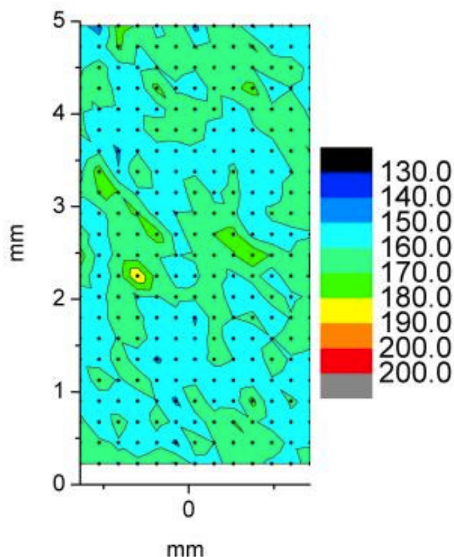
Figure 18. Vickers hardness map for Davis Besse heat M3935. The average measured hardness was 160.2 \text{ kg/mm}^2 with a standard deviation of 6.5 \text{ kg/mm}^2 .
