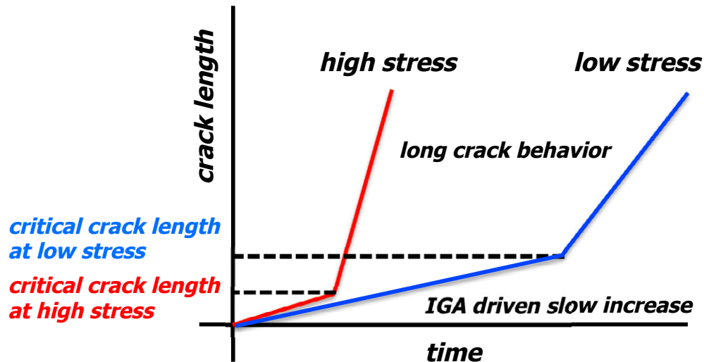
Figure 67. Qualitative representation of possible differences in initiation response between a material in a low cold work and a high cold-work condition that are tested at their yield stress.
