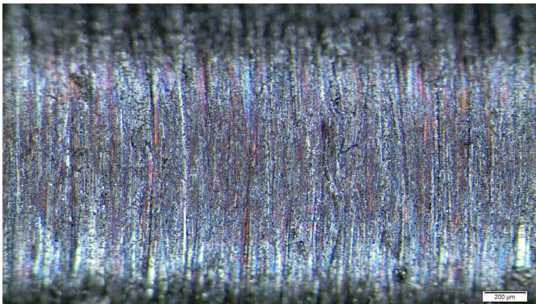
Figure 42. Optical image of the heavily ground IN018 gauge section after SCC initiation test.
