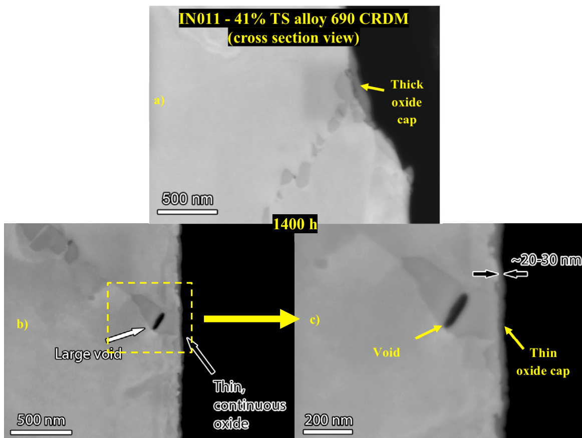
Figure 120. SEM-BSE images of the 41% tensile strained alloy 690 CRDM illustrating a thin, 20-30 nm, continuous oxide at the surface and voids between IG carbides.
