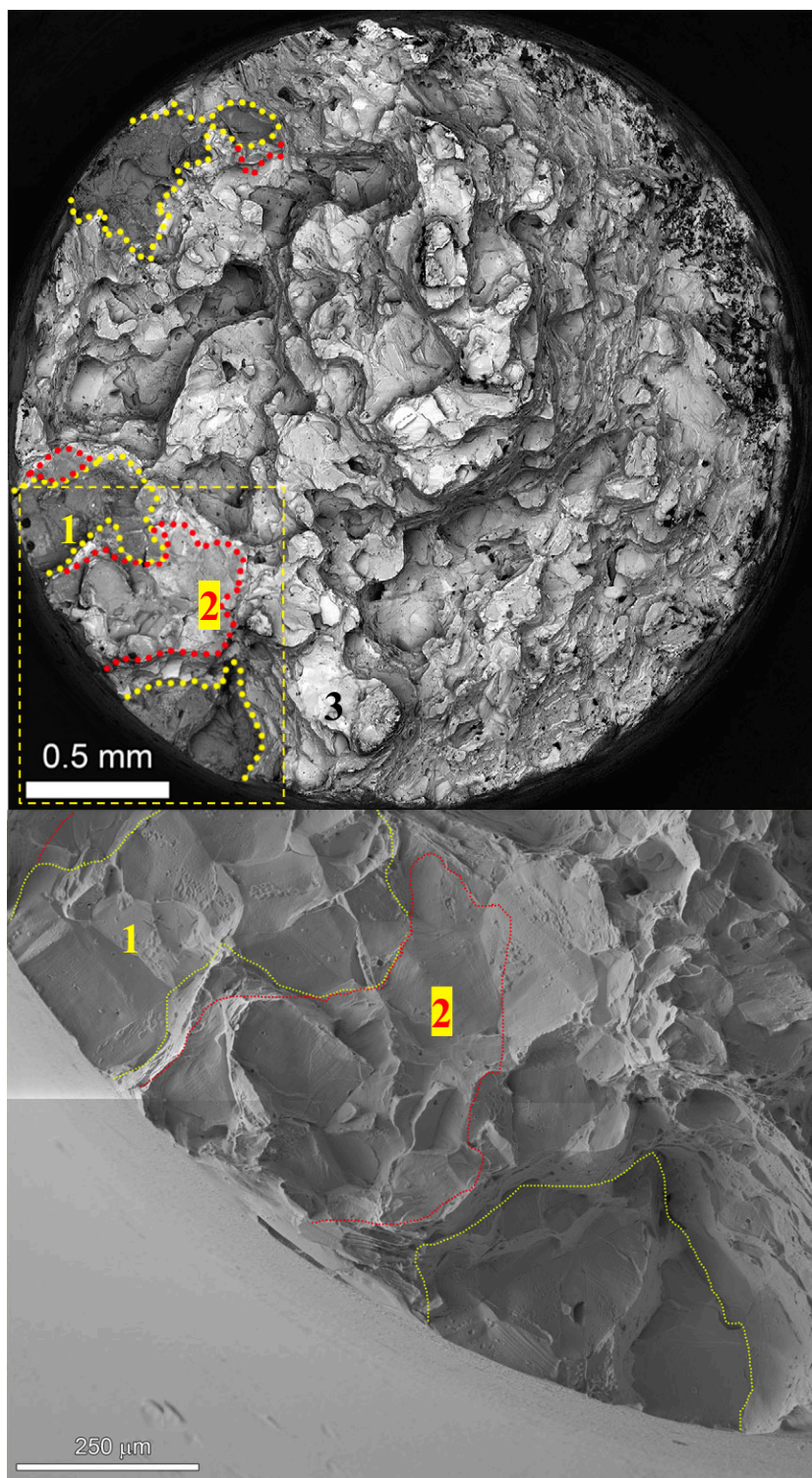
Figure 101. Low kV SEM-BSE of the fracture surface and high kV SEM-SE micrographs illustrating the fracture surface for the 31%CR CRDM specimen IN007. Several pockets of IG cracking were found where yellow is initial SCC, red is secondary SCC. Remainder of fracture surface appears to be mixture of IG and TG fracture with no apparent oxide.
