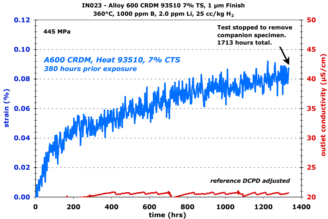
Figure 50. Strain versus time plot for specimen IN023 after restart showing DCPD adjusted strains during testing in 360°C PWR primary water with 1713 hours total exposure at this point.
