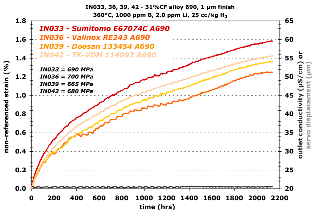
Figure 146. Non-referenced strain response for four heats of 31% CF alloy 690 undergoing long term constant load exposure at 360°C in the PNNL 36-specimen initiation test system. For each heat of material at this CW level, there are 3 specimens in the test rig.
