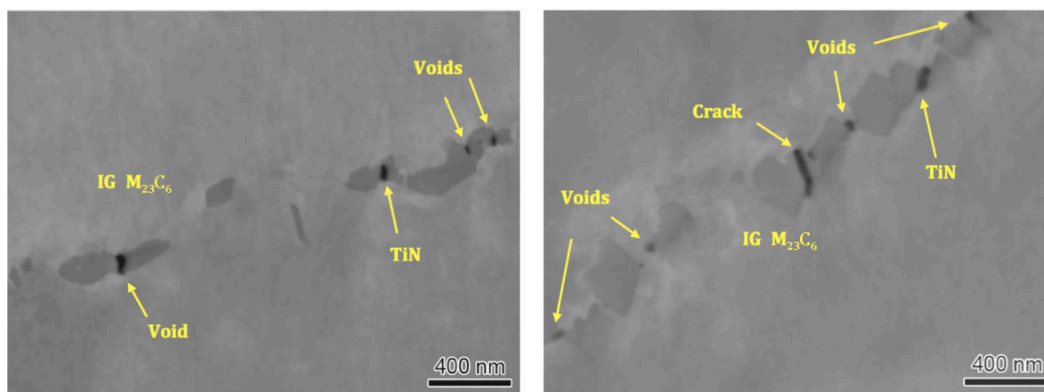
Figure 71. SEM-BSE images of the Valinox 31%CR alloy 690TT CRDM material showing voids and cracked carbides on grain boundaries in this material.
