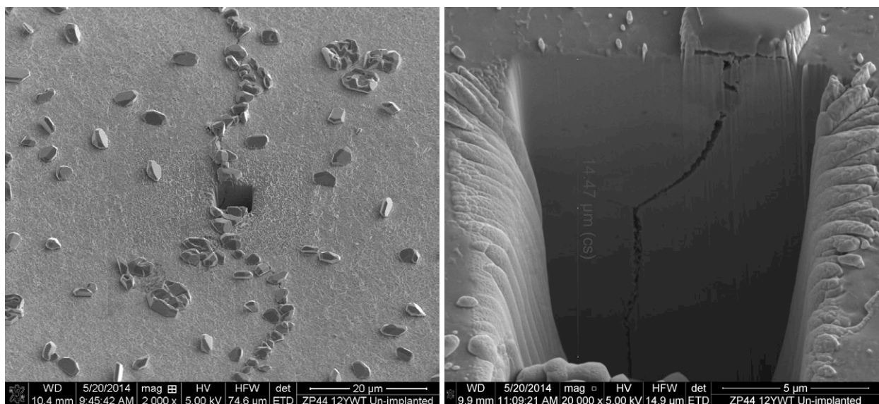
Figure 52. SEM-SE image of a FIB trench into IN023 surface to examine crack depth from the specimen surface.
