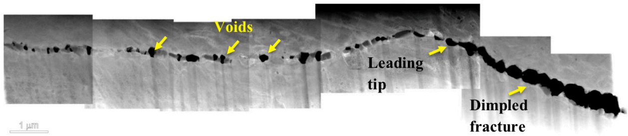
Figure 113. TEM Angular DF montage of crack #3 (see Figure 105).
