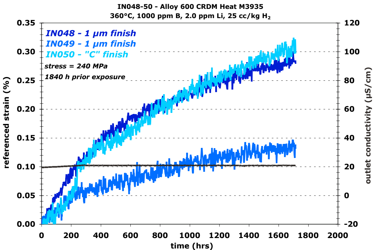
Figure 65. DCPD response for the alloy 600 CRDM specimens from PWR service (IN048, IN049 and IN050) during the ongoing second exposure in 360°C PWR primary water.
