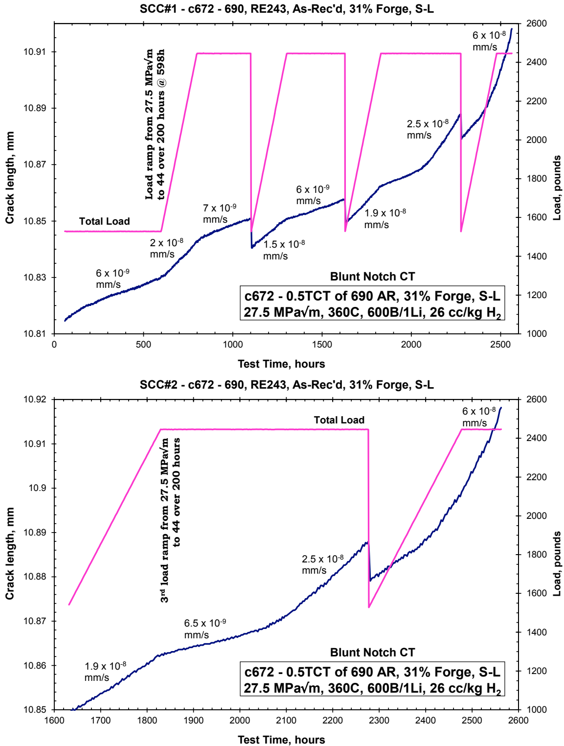
Figure 125. Crack length versus time response for the 31%CF Valinox CRDM specimen c672 blunt notch specimen.
