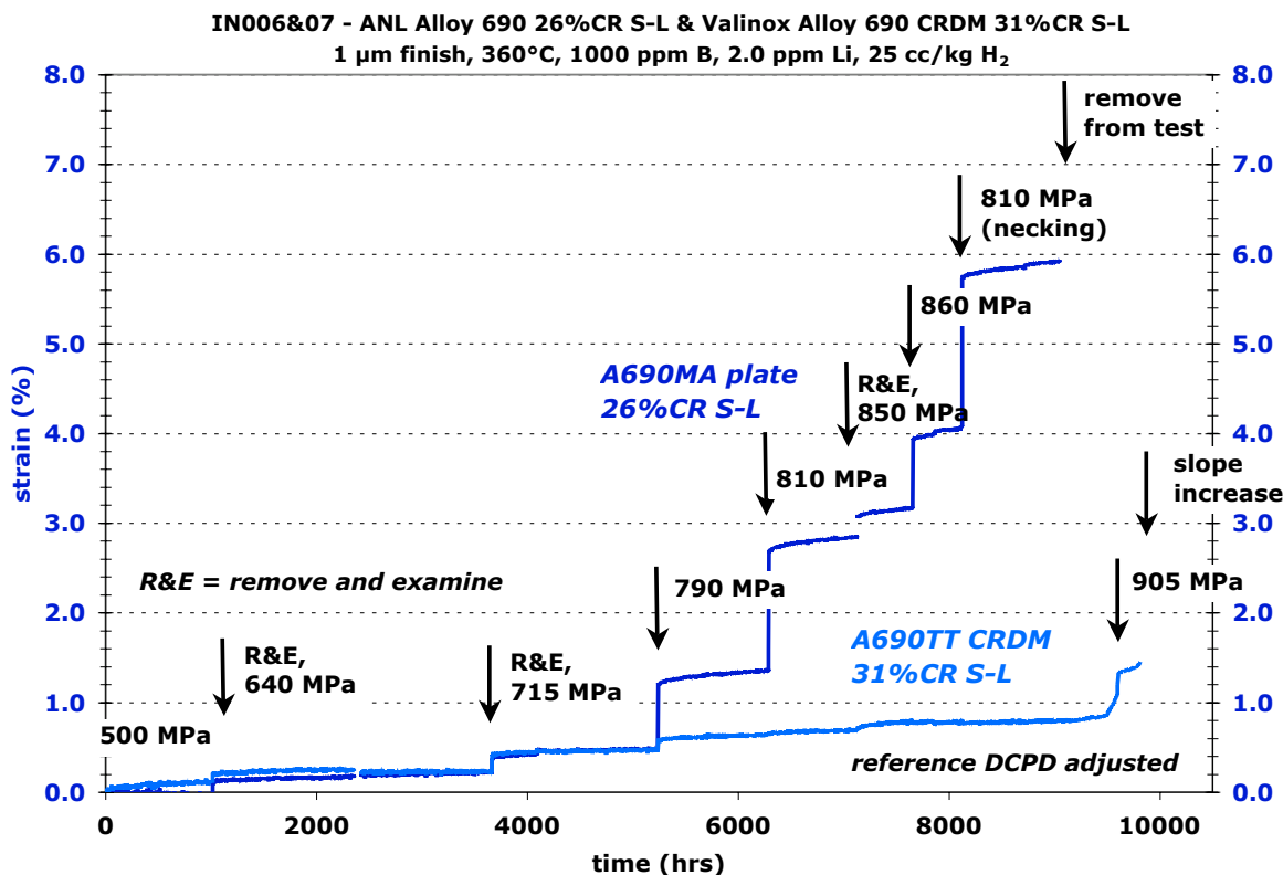
Figure 74. Overview of the test on the two cold-rolled and SCC susceptible alloy 690 specimens, IN006 and IN007. Changes in stress on the specimens are listed.
