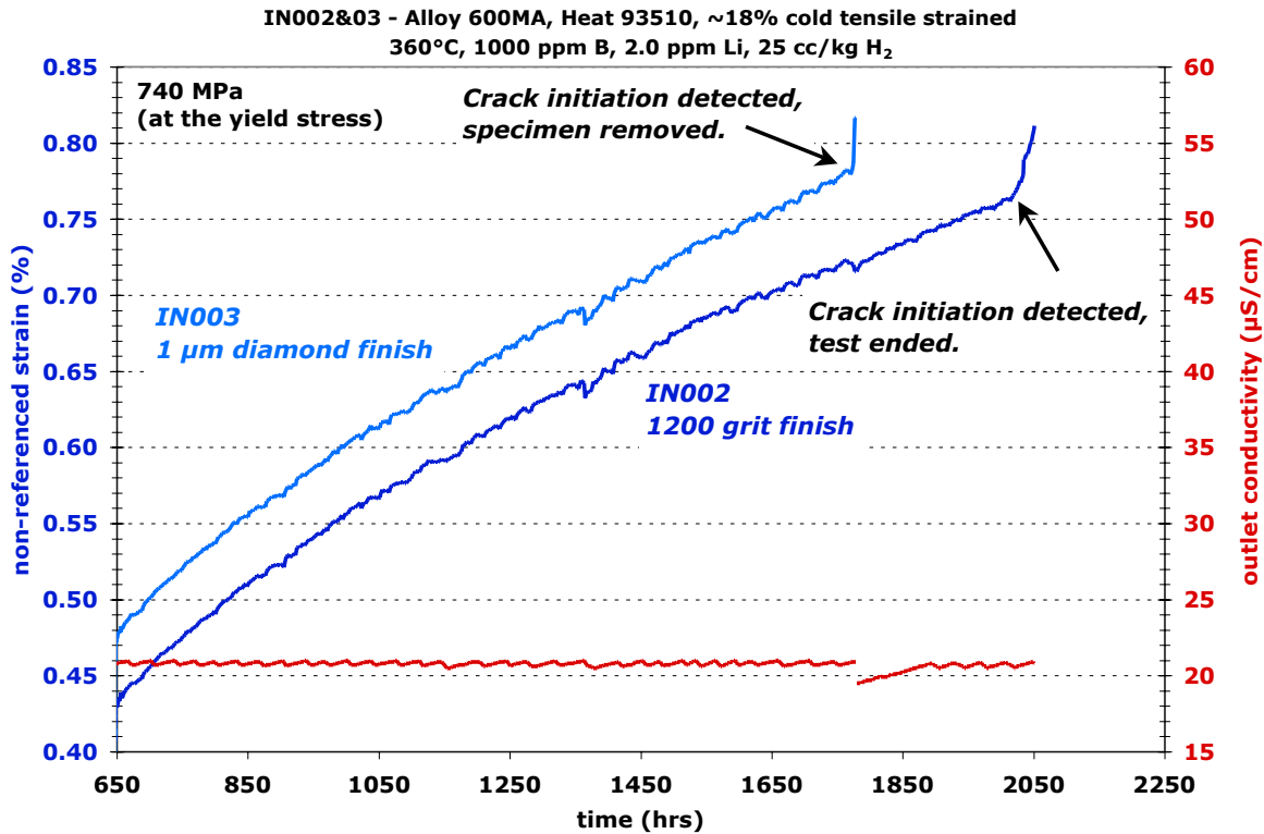
Figure 27. SCC crack initiation tests on 18% tensile prestrained alloy 600 CRDM Heat 93510.
