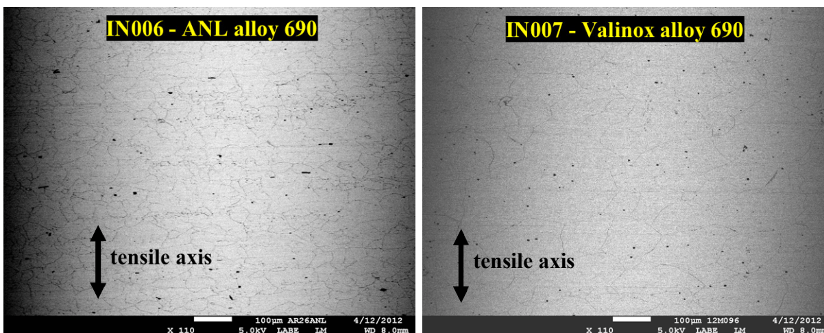
Figure 73. SEM-BSE images of a portion of the polished gauge section of IN006 and IN007 prior to testing revealing grain boundary carbides and TiN particles intersecting the specimen surface.
