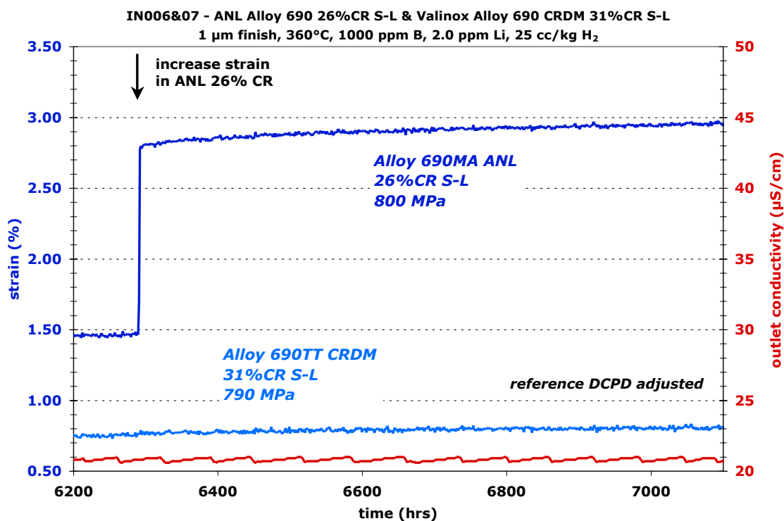
Figure 84. DCPD-based strain response of the two CR alloy 690 specimens (IN006 and IN007) from 6200 - 7100 hours after plastic deformation in plate specimen IN006.
