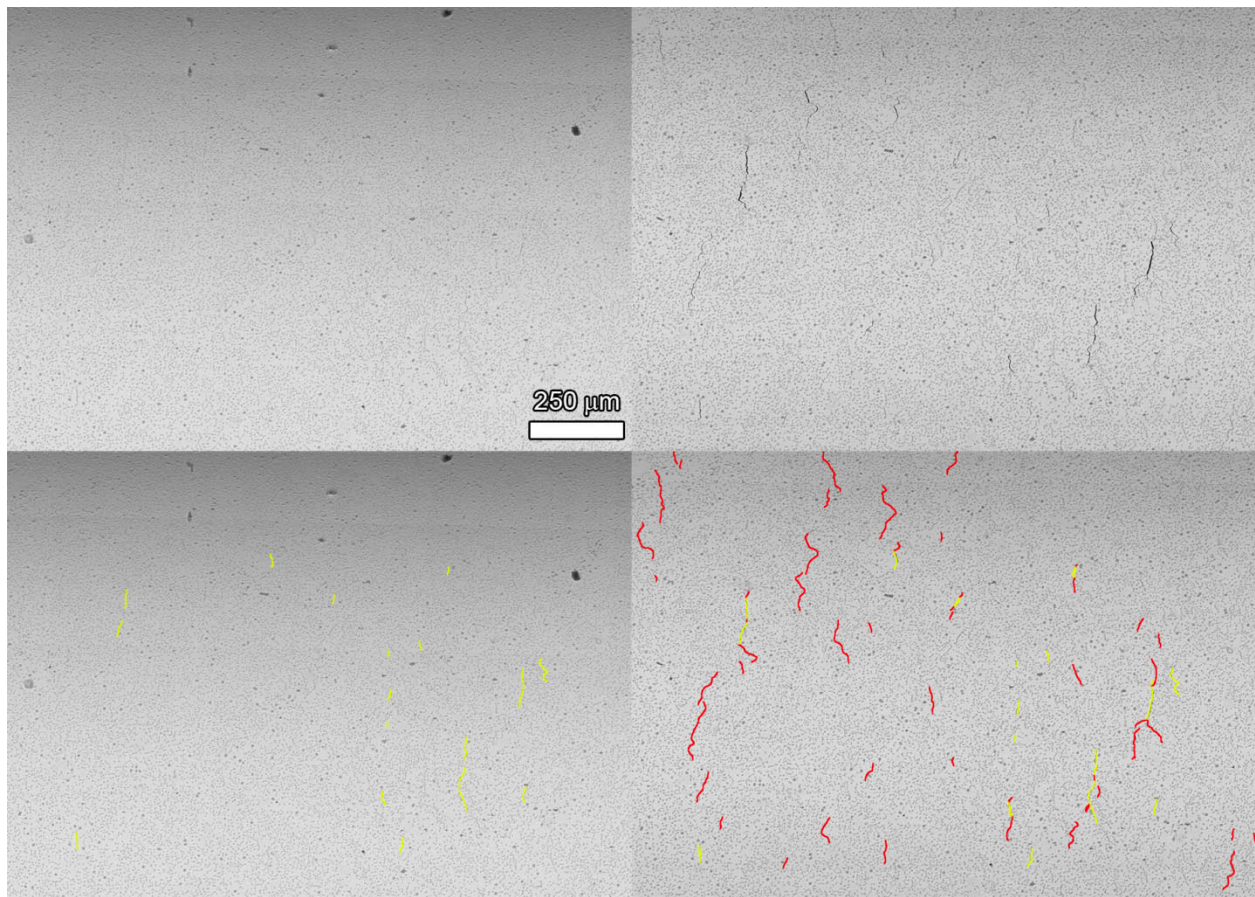
Figure 56. SEM-BSE images of IN023 Rotation 3 illustrating the sample at 1713 hours (left columns) and 2591 hours (right columns). The bottom two figures highlight the cracks in yellow present at 1713 hours and new cracks in red present at 2591 hours (red).
