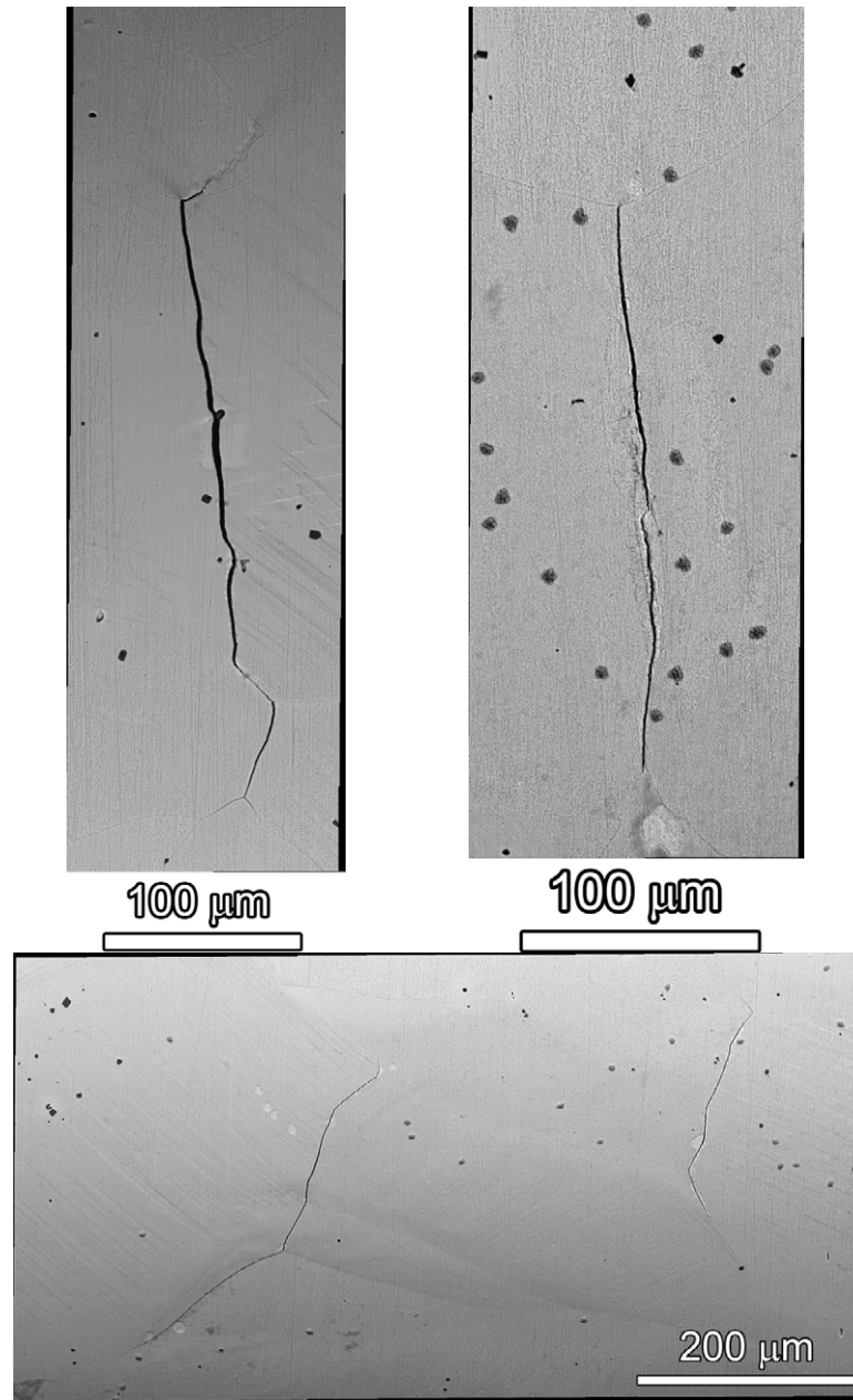
Figure 48. SEM-BSE images illustrating morphology of several large IGSCC cracks on the gauge surface of the IN022 specimen.
