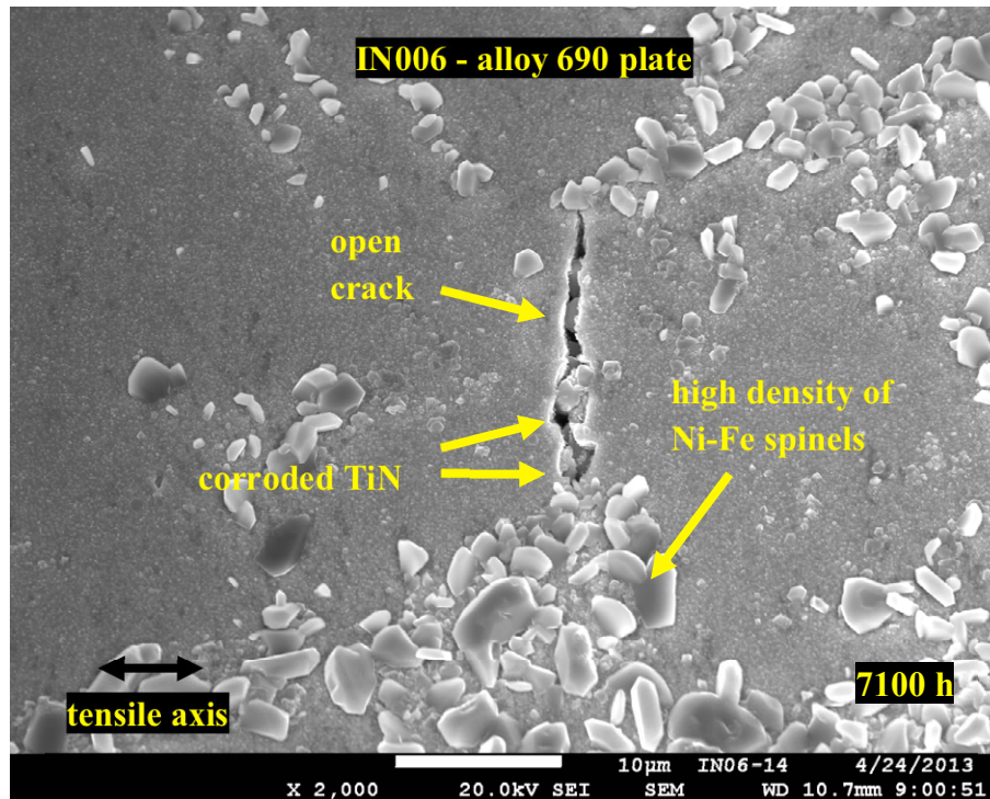
Figure 86. Example of surface crack morphology in the 26%CR plate specimen (IN006) after ~7100 hours of exposure.
