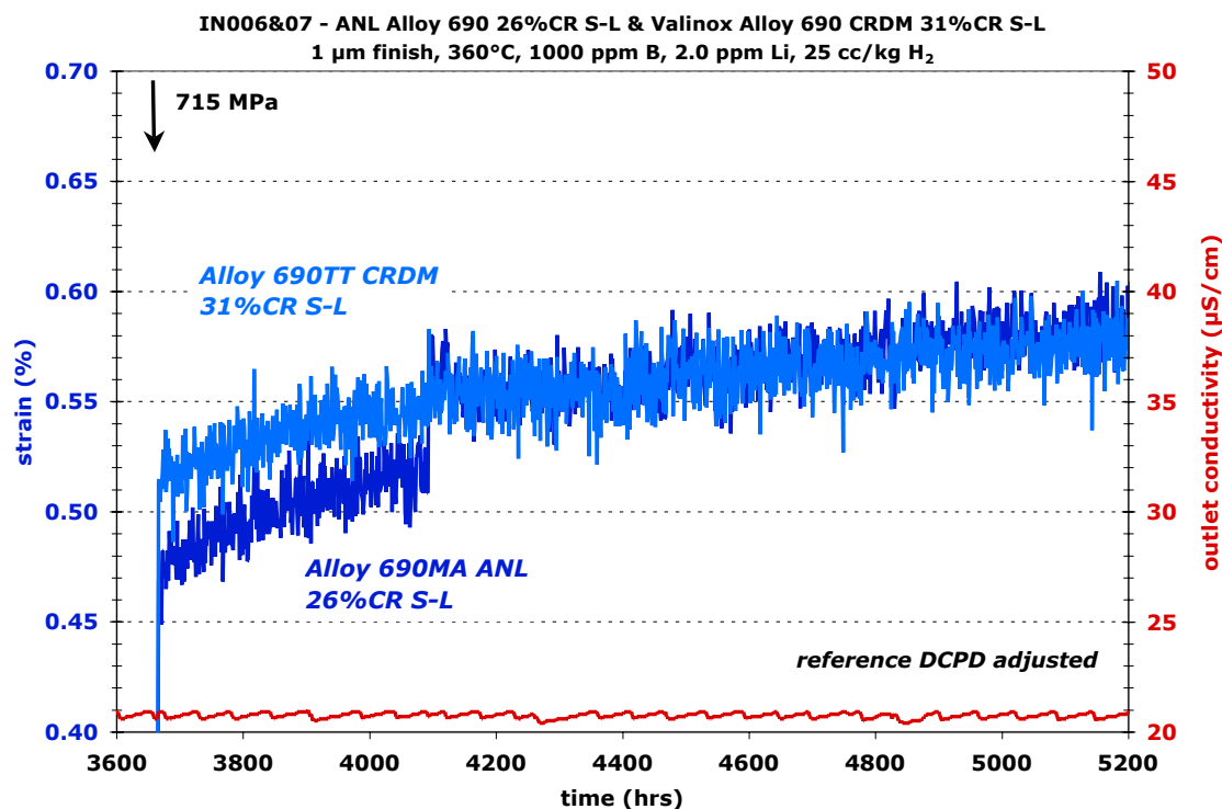
Figure 80. DCPD-based strain response of the two cold-rolled alloy 690 specimens (IN006 and IN007) from 3630 - 5200 hours after stress increase to 715 MPa.
