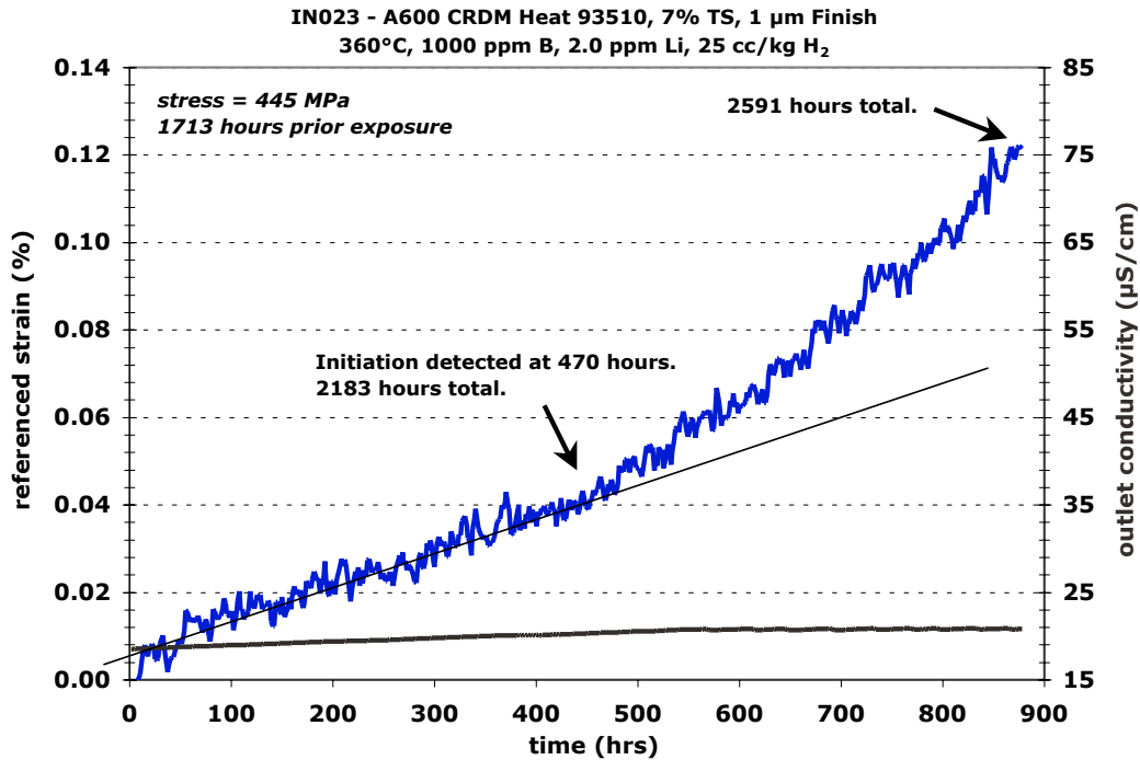
Figure 53. SCC initiation plot for specimen IN023 showing reference DCPD adjusted equivalent strains during the third exposure in 360°C PWR primary water. Initiation detected after 2183 hours total.
