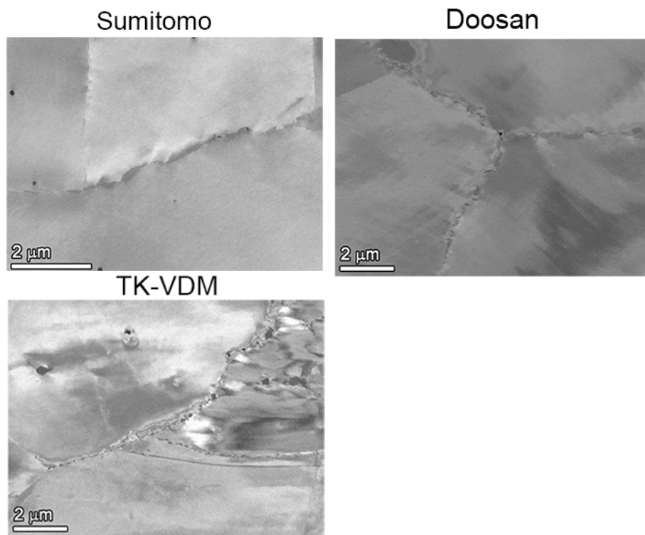
Figure 69. SEM-BSE micrographs showing carbide microstructure of the Sumitomo, Doosan and TK-VDM materials.
