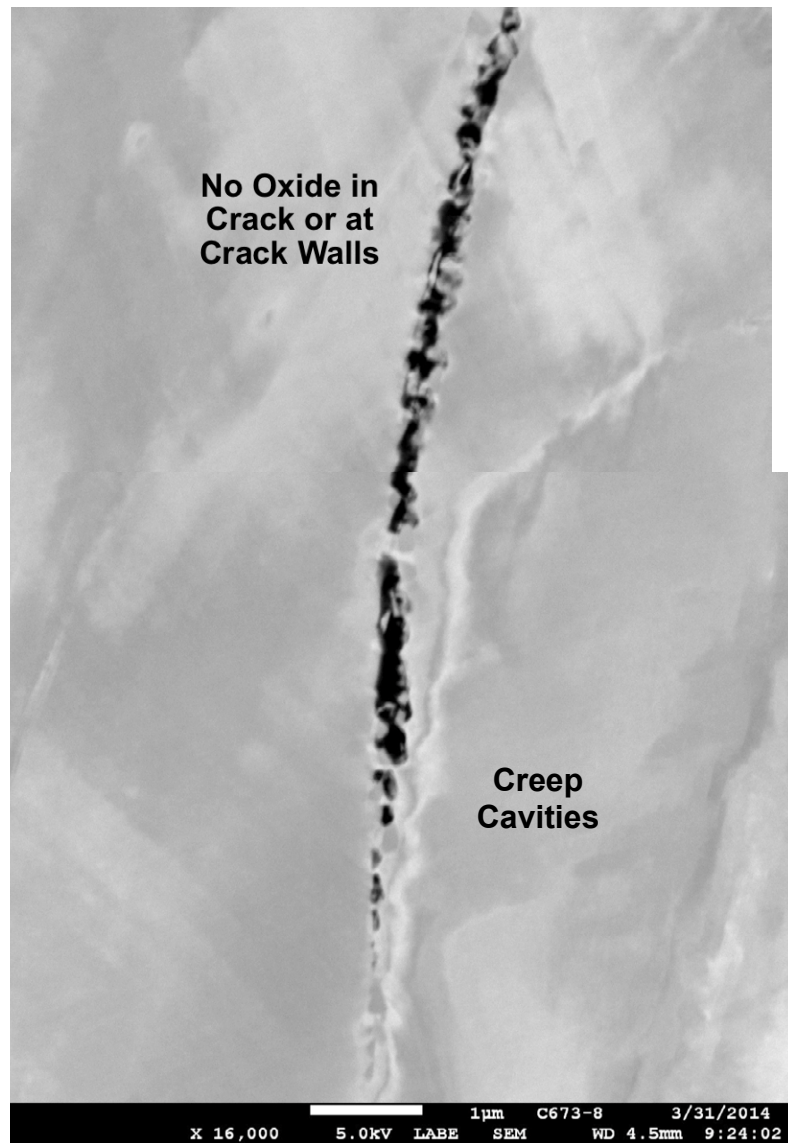
Figure 138. Example of IG creep crack and cavities in cross-section slice #2 from blunt notch specimen c672.
