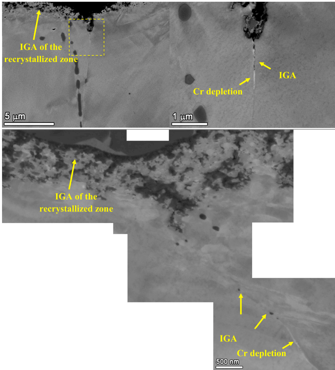
Figure 45. SEM-BSE micrographs of IN018 showing IG attack of boundaries that intersect the surface as well as a boundary below the recrystallized layer.
