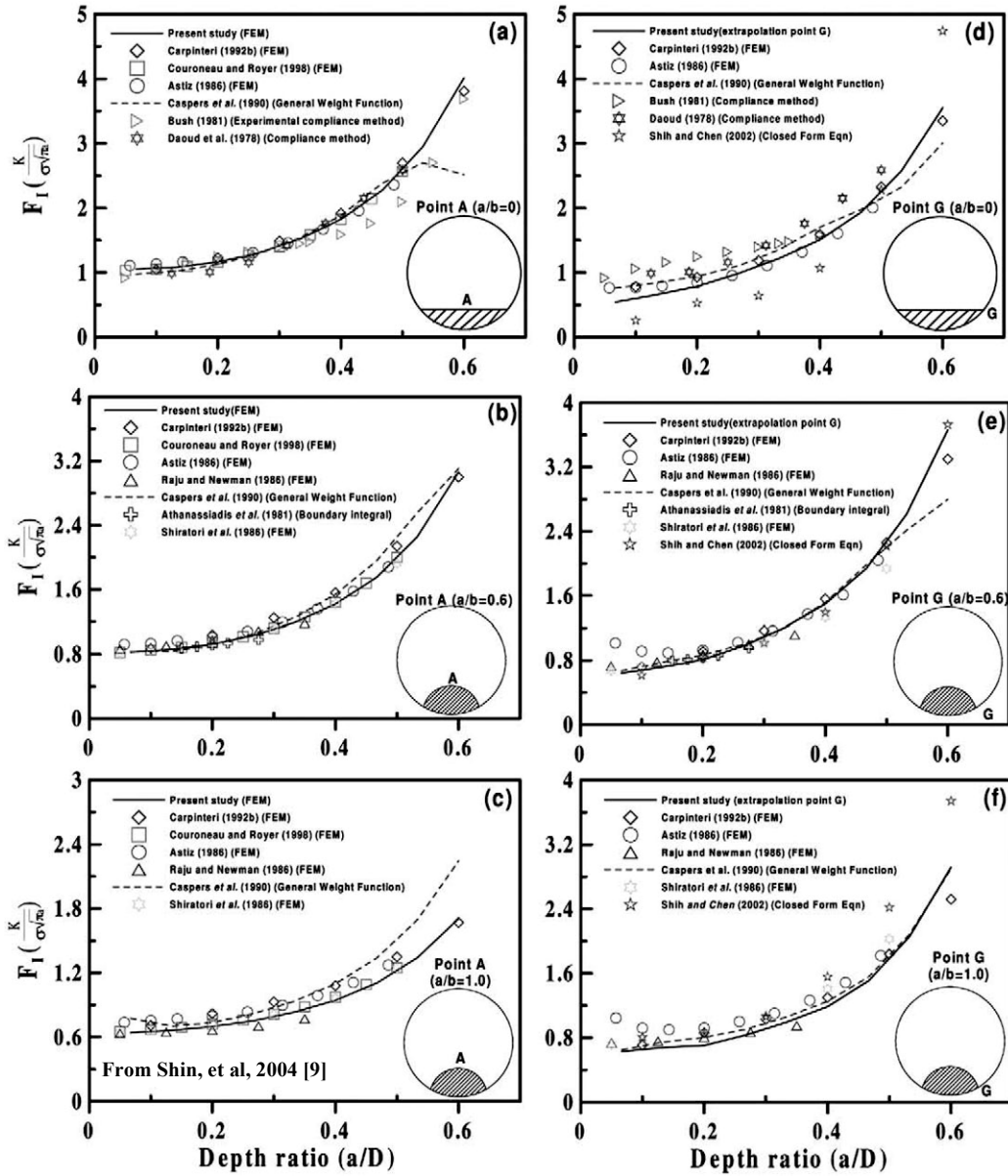
Figure 7. Dimensionless stress intensity factor at either the center or edge of the crack plotted against a/D for three different crack shapes as given by Shin [9].
