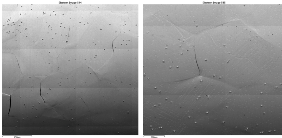
Figure 64. Examples of apparent SCC cracks in the IN049 specimen after the demonstration test exposure for 1840 hours under constant load at the yield stress in 360°C PWR primary water.
