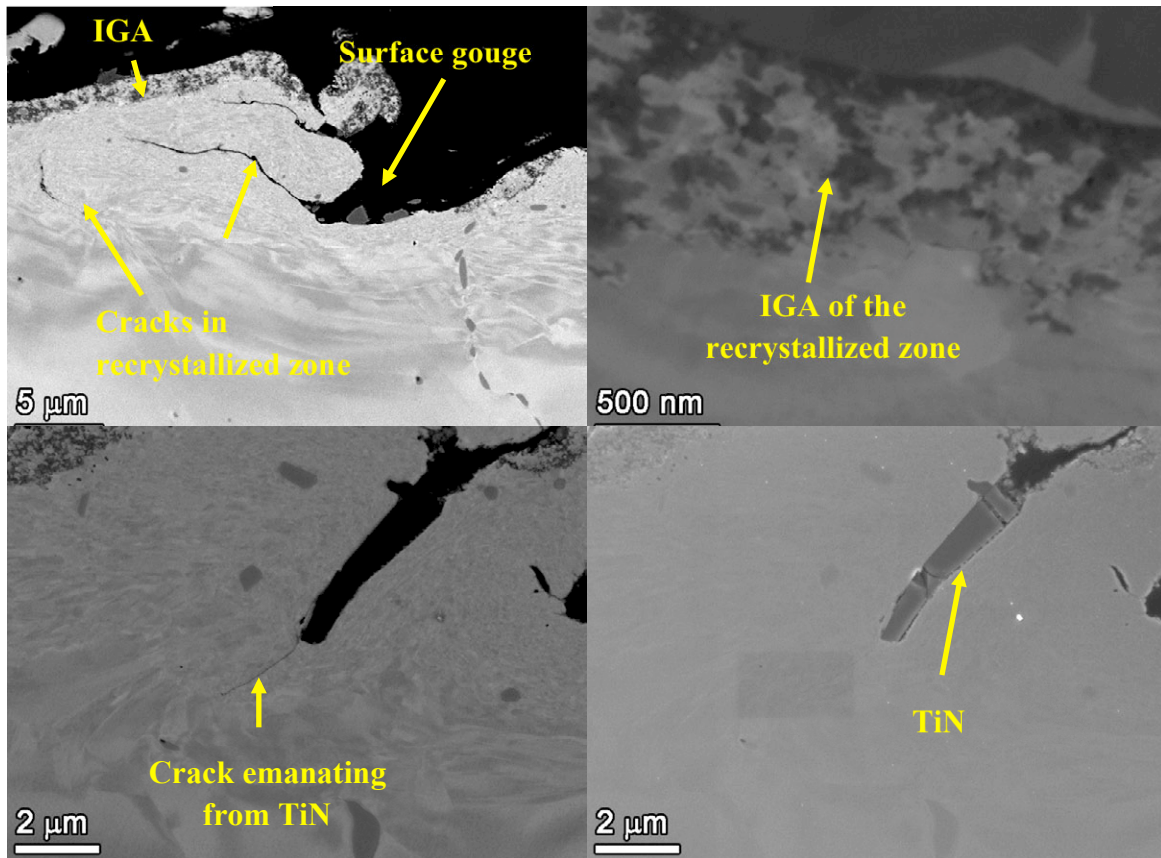
Figure 44. SEM-BSE image of the IN018 cross-section showing that the surface is comprised of a recrystallized zone of nanocrystalline grains. Once exposed, this surface slowly corrodes. Random cracking within the nanocrystalline zone was observed and was most likely imparted during grinding. Lastly, cracks were observed to emanate from TiN particles near the surface.
