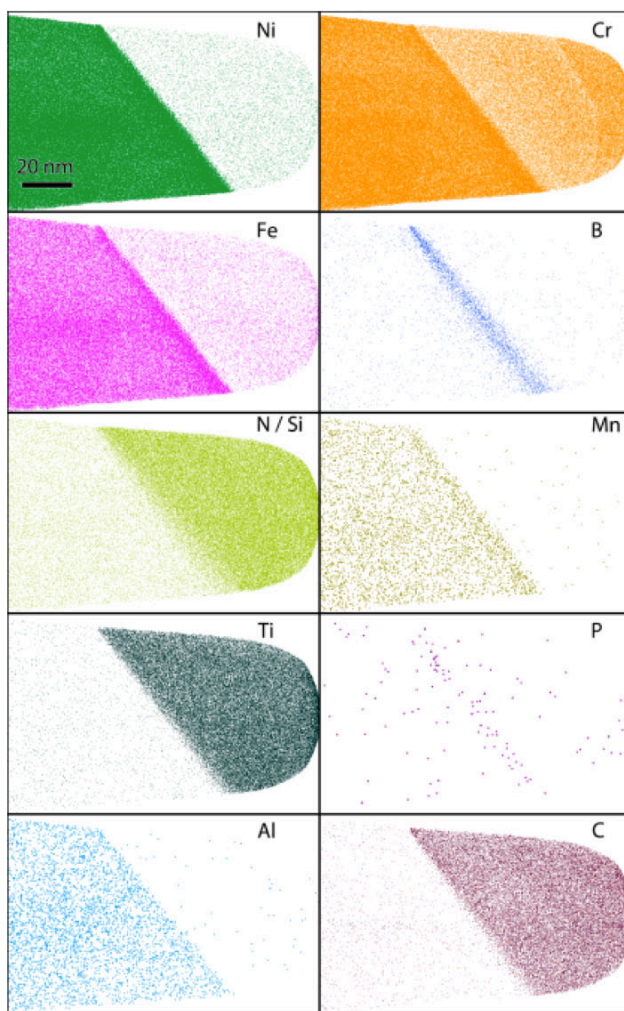
Figure 20. Atom map (10 nm image depth) of an IG Ti carbo-nitride in Davis Besse CRDM heat M3935. Strong interfacial segregation is apparent for B and weak segregation for P. Note that Si and N peaks are convoluted with one another and impossible to differentiate.
