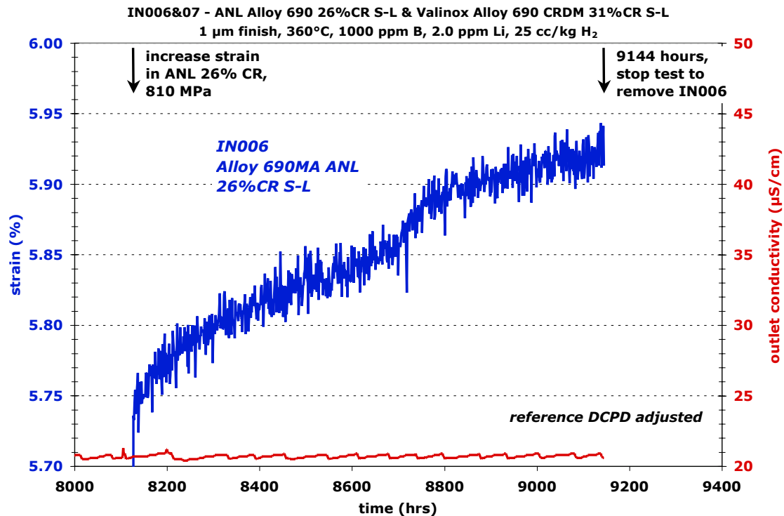
Figure 95. DCPD-based strain response of the 26%CR ANL alloy 690 plate specimen IN006 from 8150 to 9144 hours.
