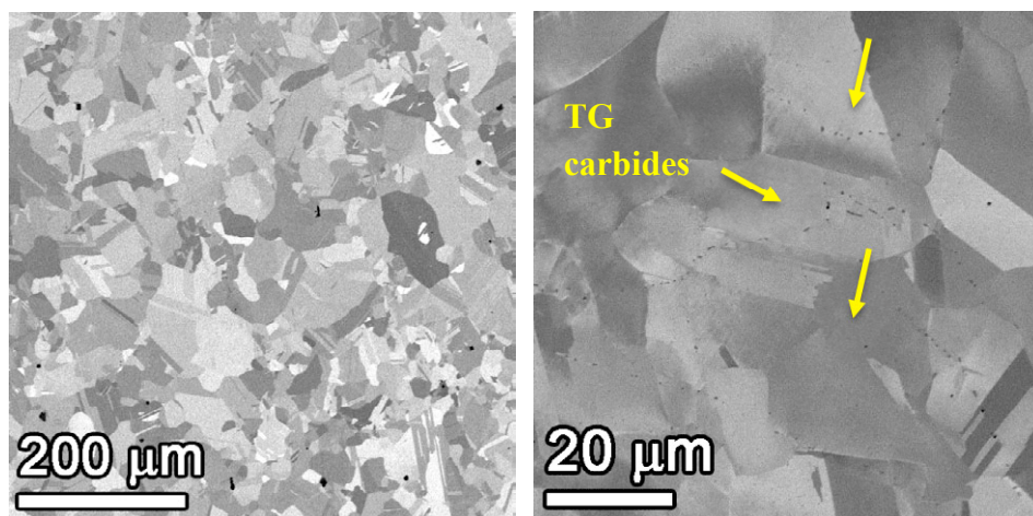
Figure 25. SEM (BSE) micrographs illustrating the microstructure of CRDM tube heat 93510 and the transgranular nature of the carbides.
