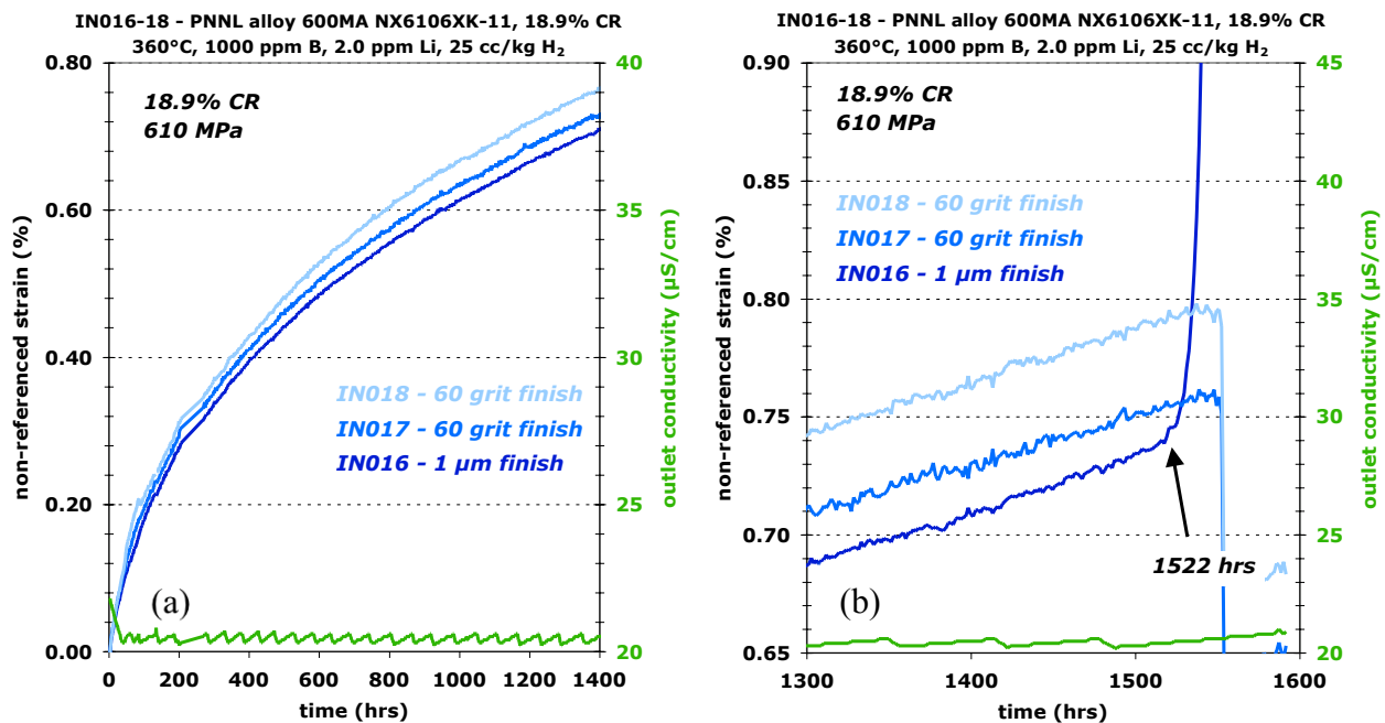
Figure 38. SCC initiation test plots for 19%CR alloy 600 specimens IN016, IN017 and IN018 during testing in 360°C PWR primary water: (a) early DCPD response and (b) observation of crack initiation and growth for the IN016 specimen.
