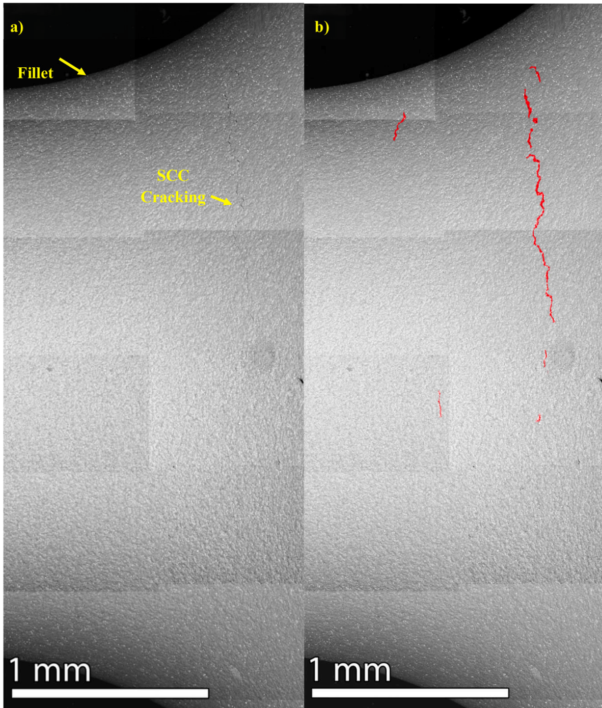
Figure 28. SEM (BSE) images of the alloy 600 tensile initiation specimen IN003 surface that exhibited cracking near the fillet. Image (b) is identical image to (a), but cracks have been colored red as guide to the eye. The longest crack observed in this region was nearly 1 mm in length.
