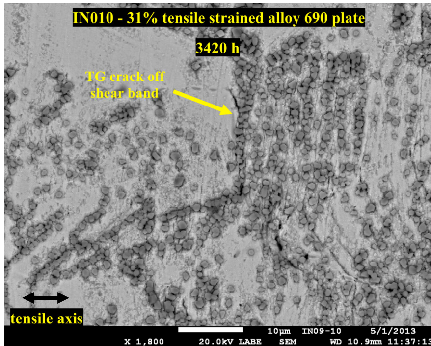
Figure 123. SEM-BSE image of the surface the 31%TS ANL alloy 690 plate specimen (IN010) showing shear bands intersecting the surface. Cracks appear to have formed at many shear bands. Large Ni-Fe spinels on the surface obscure the view.
