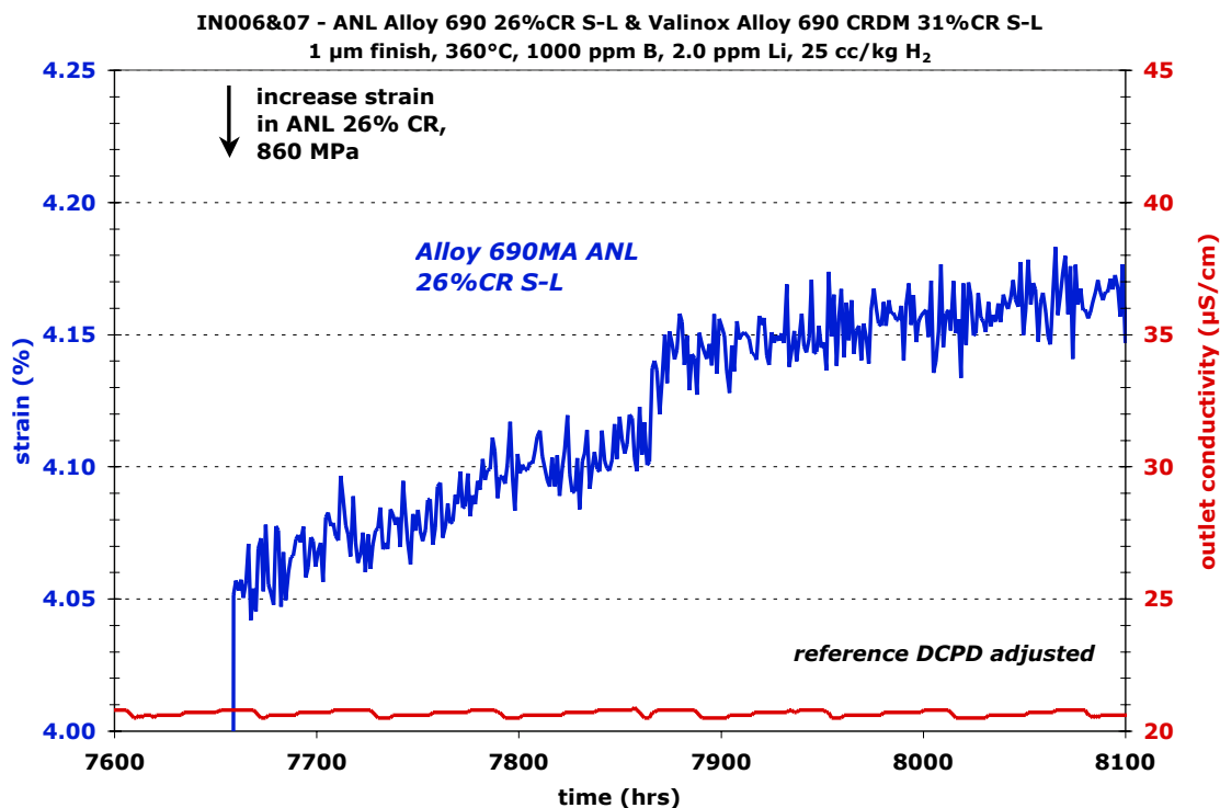
Figure 93. DCPD-based strain response of the 26%CR ANL alloy 690 plate specimen IN006 from 7650 to 8100 hours.
