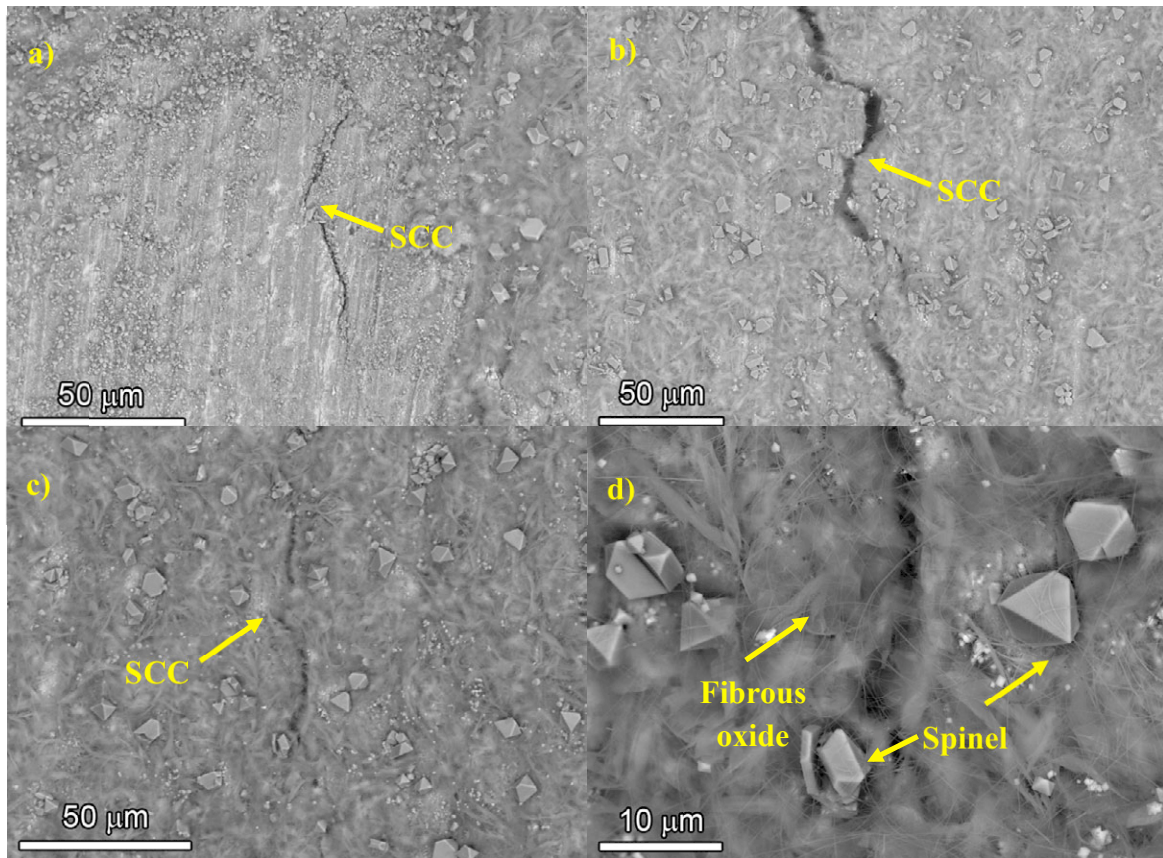
Figure 30. Low magnification SEM (BSE) images of the surface of the IN003 alloy 600 tensile initiation specimen illustrating various SCC cracks and surface oxides.
