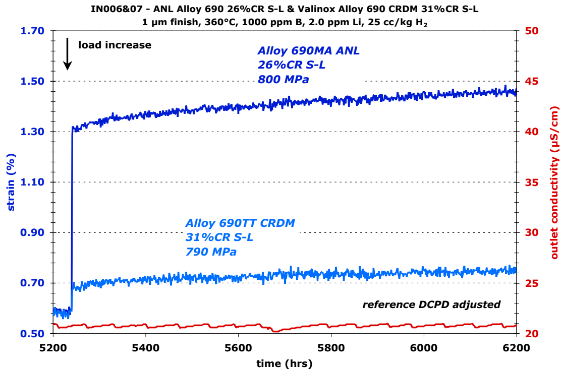
Figure 82. DCPD-based strain response for the IN006 and IN007 specimens from 5220 to 6200 hours after another load increase to 790-800 MPa.
