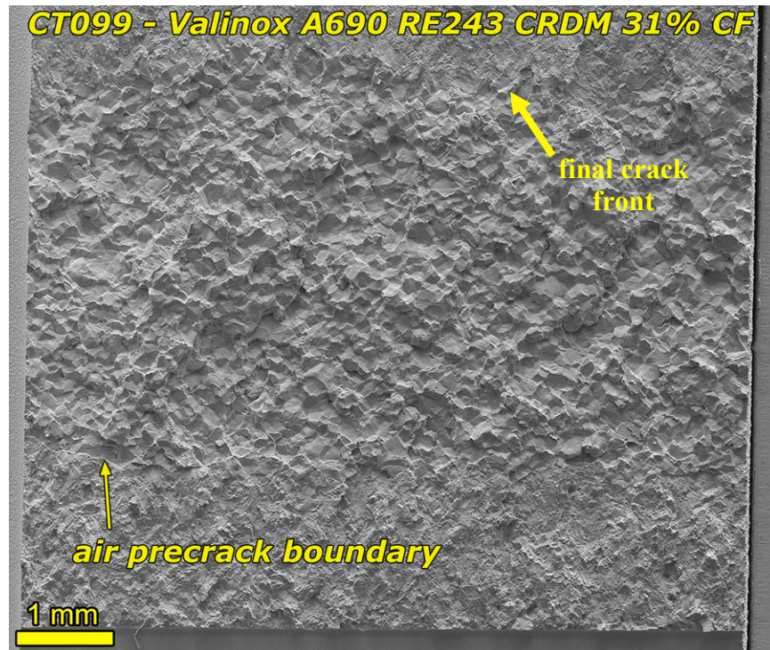
Figure 144. SEM-SE image of the entire crack growth surface of CT099 (Sumitomo CRDM).
