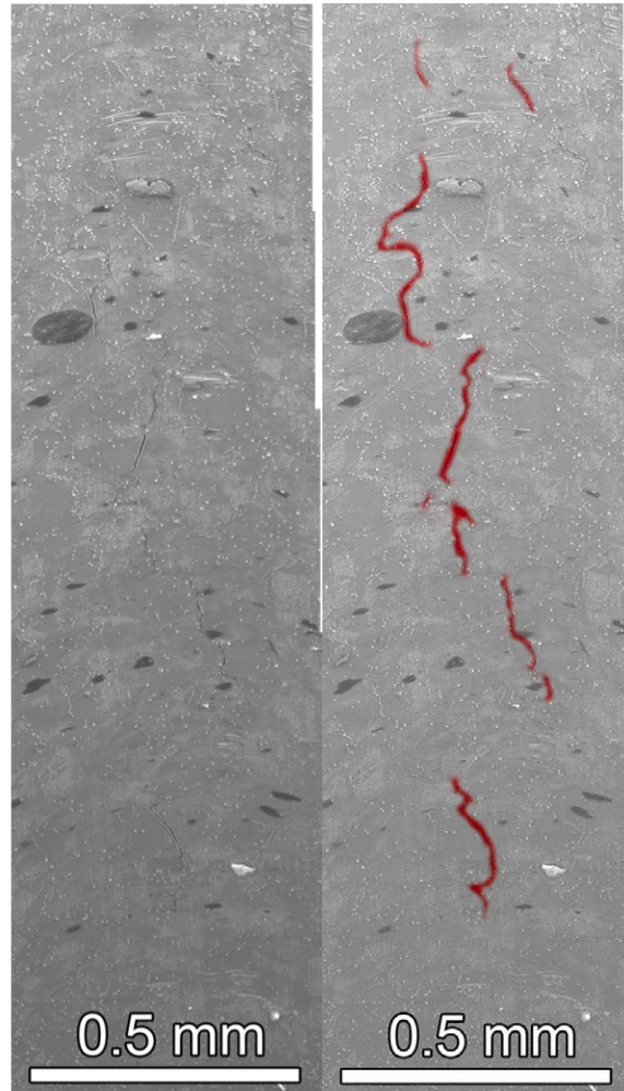
Figure 129. SEM-SE image of a portion of the 31%CF Valinox CRDM specimen c672 notch showing several nucleated cracks (highlighted by red marker in right image). Note that the image was taken at an oblique angle.
