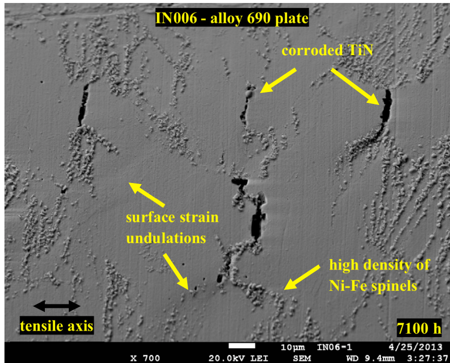
Figure 87. Observable surface strains on the 26%CR plate specimen (IN006) after ~7100 hours of exposure. Surface strains were often obscured by Ni-Fe spinels.
