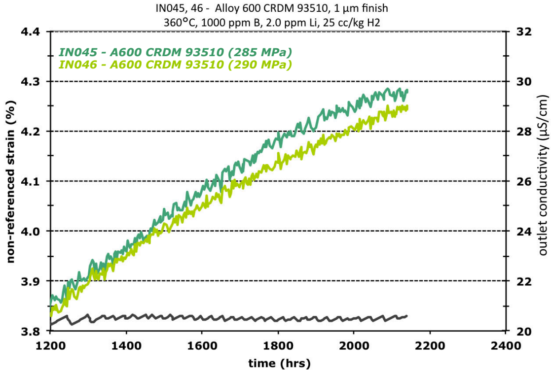
Figure 62. DCPD response for as-received alloy 600 CRDM specimens IN045 and IN046 during their first exposure in 360°C PWR primary water. IN047 was not instrumented in this exposure.
