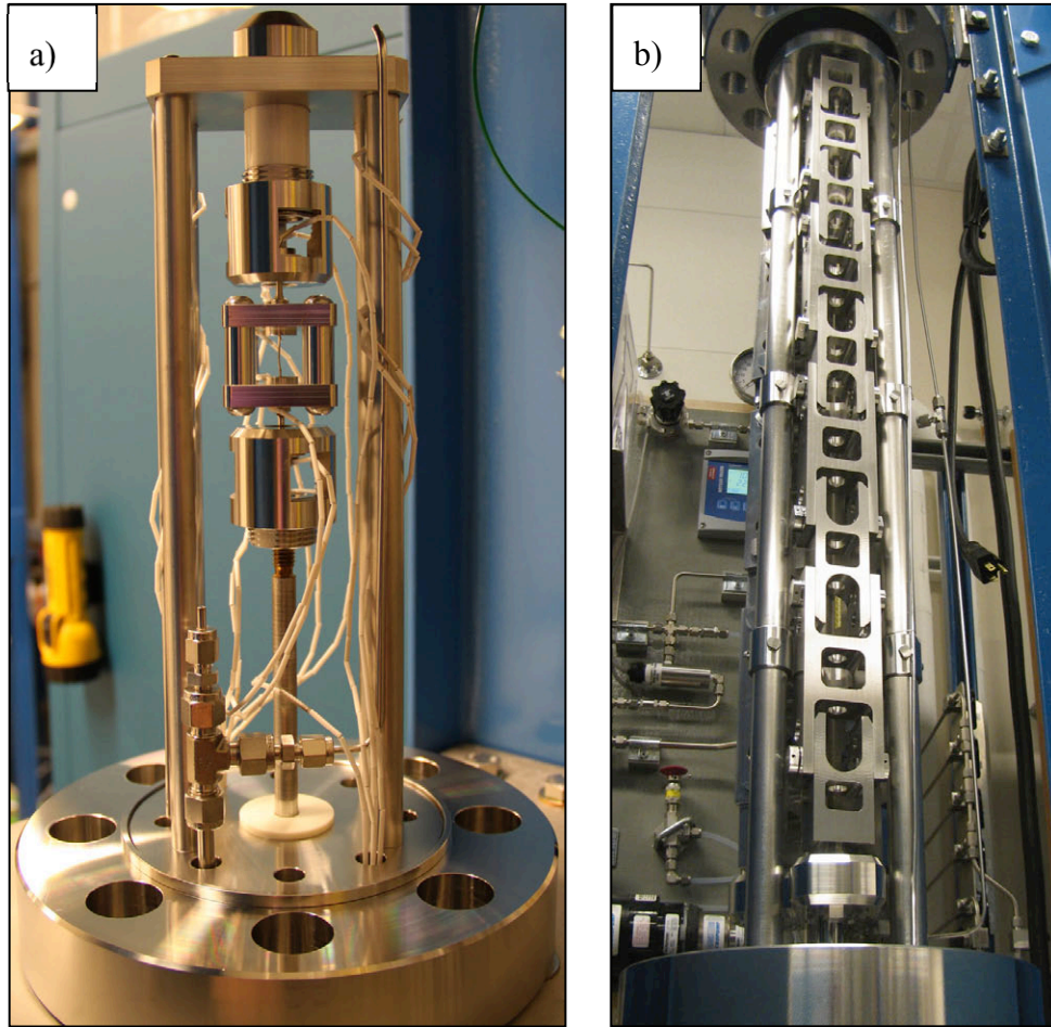
Figure 8. Crack initiation test system load trains at PNNL for (a) 1-3 specimens and (b) up to 36 specimens.
