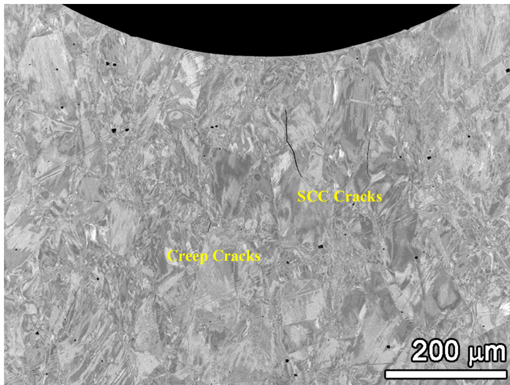
Figure 135. Blunt notch c672 cross-section slice #1 showing what are identified as SCC and creep cracks.
