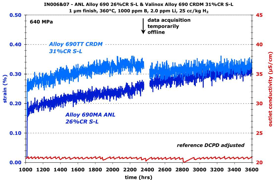
Figure 77. DCPD-based strain response for specimens IN006 and IN007 after stress increase to 640 MPa.
