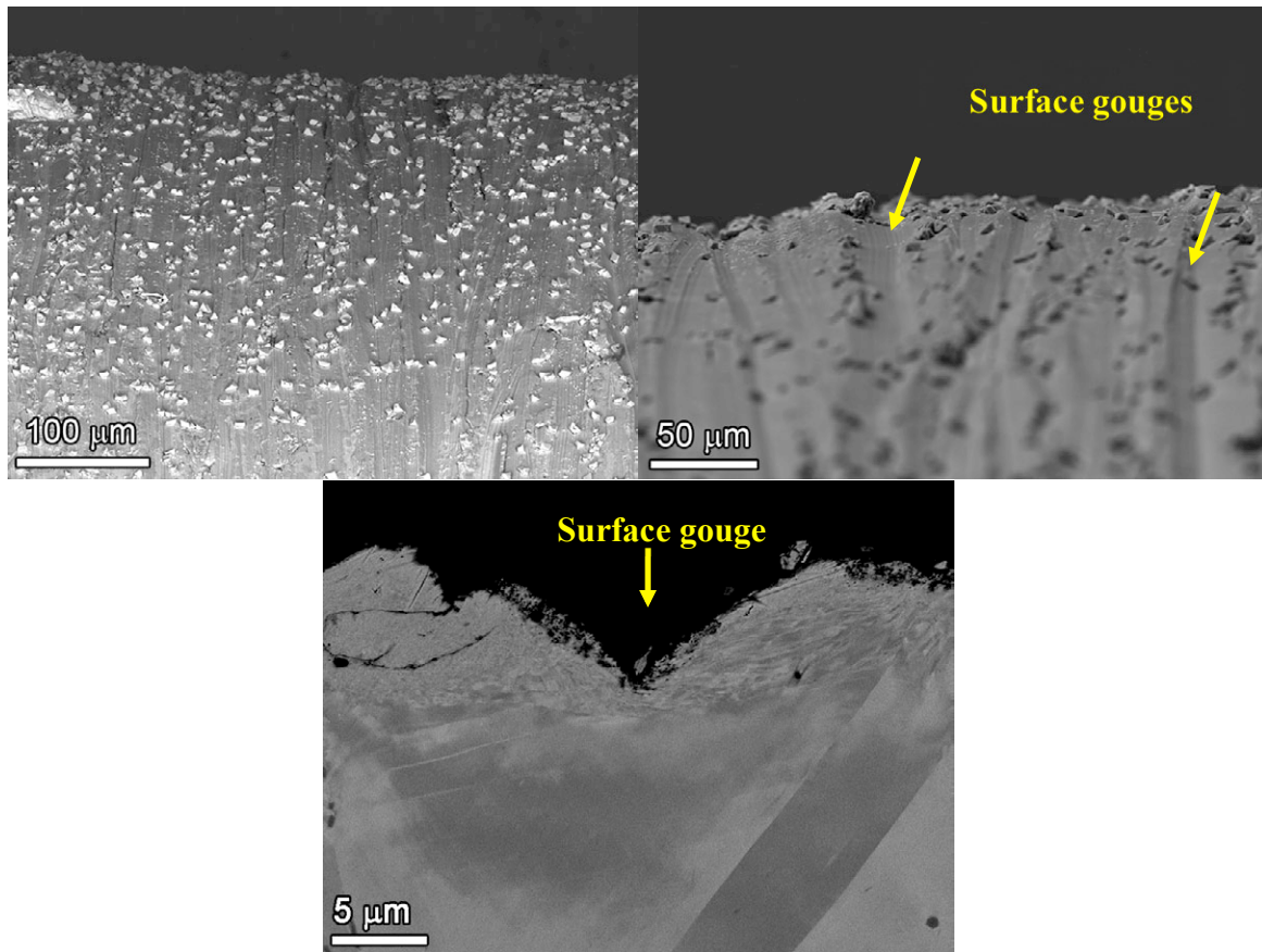
Figure 43. SEM-BSE images of IN018 gauge section in both plan view at two different angles as well as a cross-sectional example. The depth and microstructure of the gouges observed in the plan view can clearly be observed in the cross-section image to be on the order of tens of micrometers.
