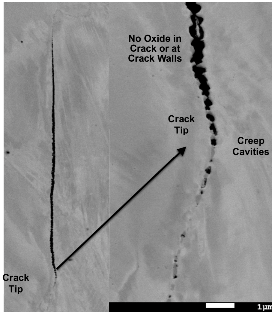
Figure 139. SEM-BSE cross-section image of c673 slice #4 showing creep crack tips. This slice had many large SCC cracks.
