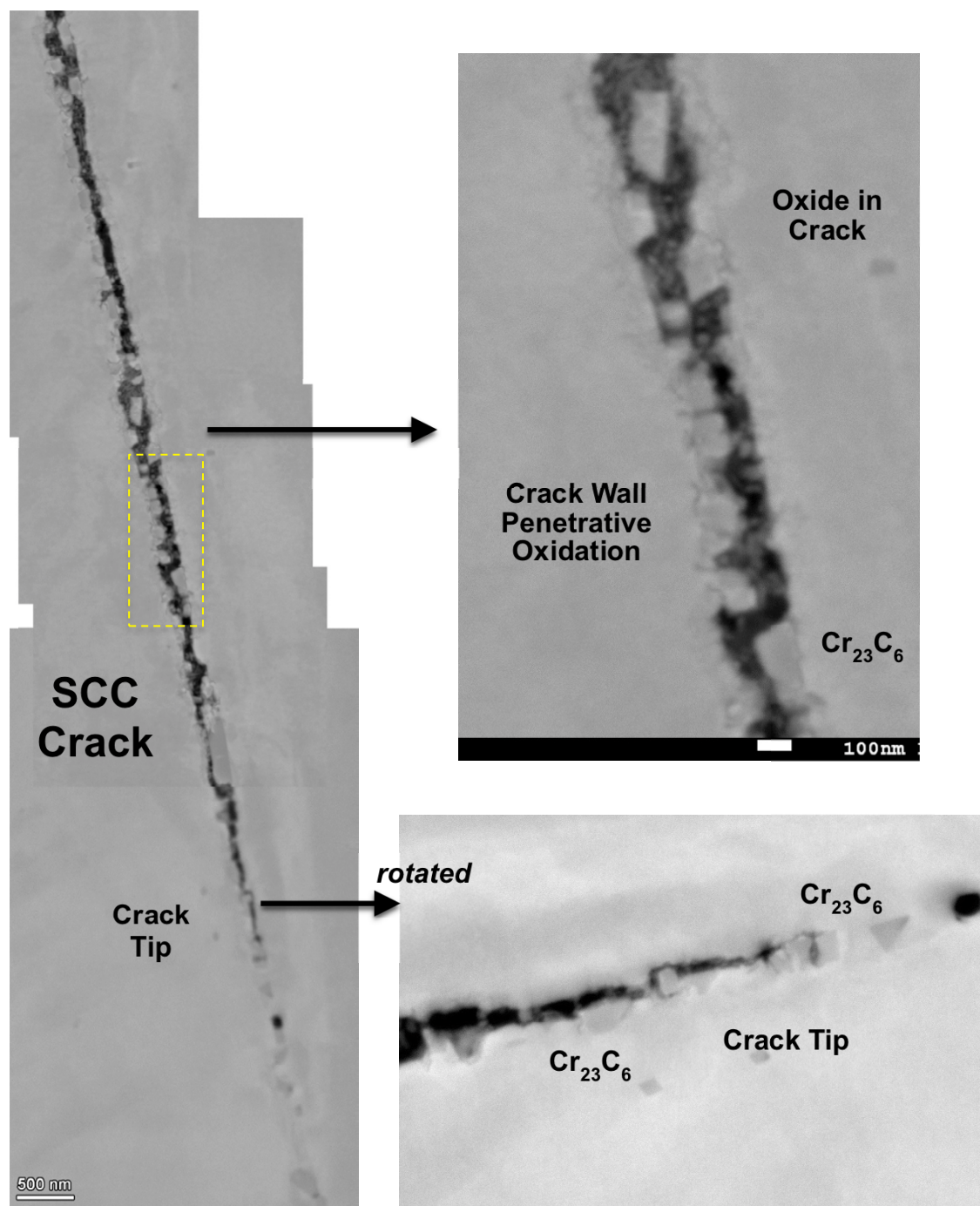
Figure 108. SEM-BSE images showing penetrative oxidation in the dashed red box in Figure 106.
