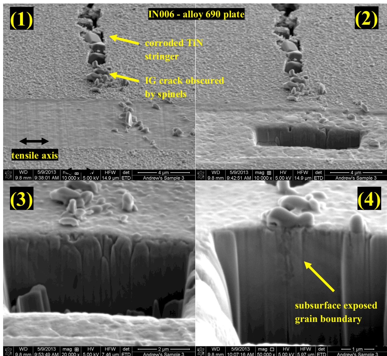
Figure 89. Step-by-step imaging of the formation of a trench into the surface of the 26%CR plate specimens (IN006) to reveal a subsurface IG crack in cross section.
