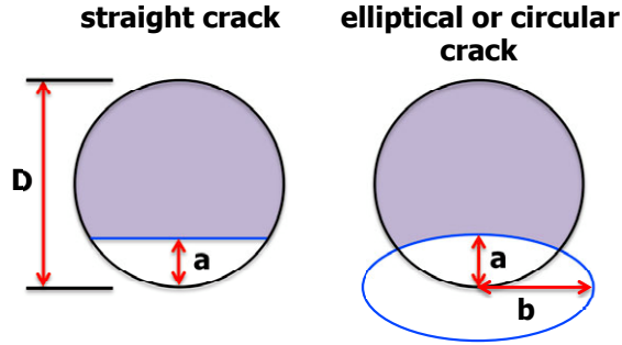
Figure 6. Types of cracks considered for stress intensity calculations.
