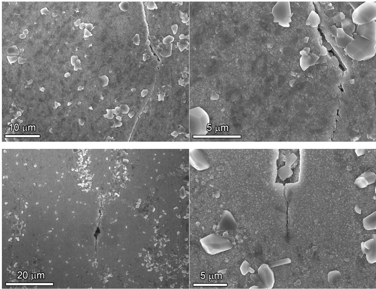
Figure 96. SEM-SE images of the gauge surface appearance for specimen IN006 after 9144 h.
