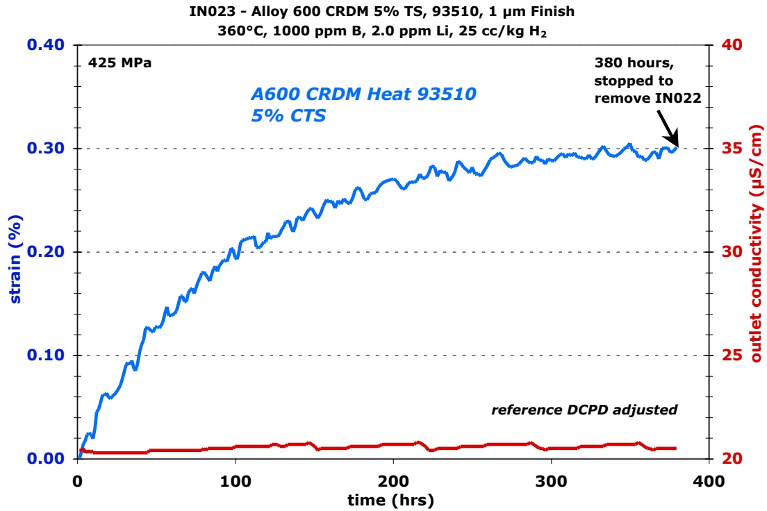
Figure 49. Strain versus time plot for specimen IN023 showing reference DCPD adjusted strains during testing in 360°C PWR primary water.
