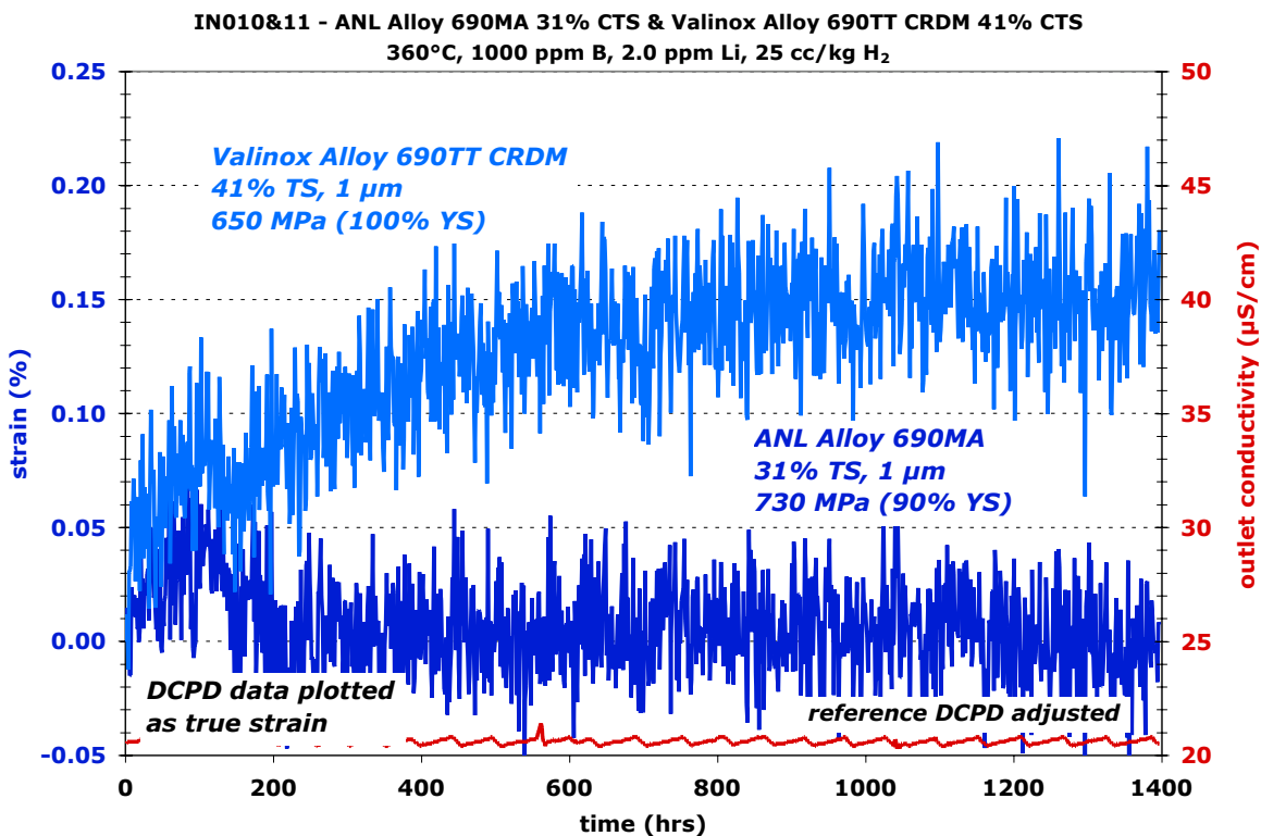
Figure 116. 31% tensile strained ANL alloy 690 plate (IN010) and 41% tensile strained alloy 690 CRDM (IN011) response during exposure in 360°C simulated PWR primary water at constant load near the yield stress.
