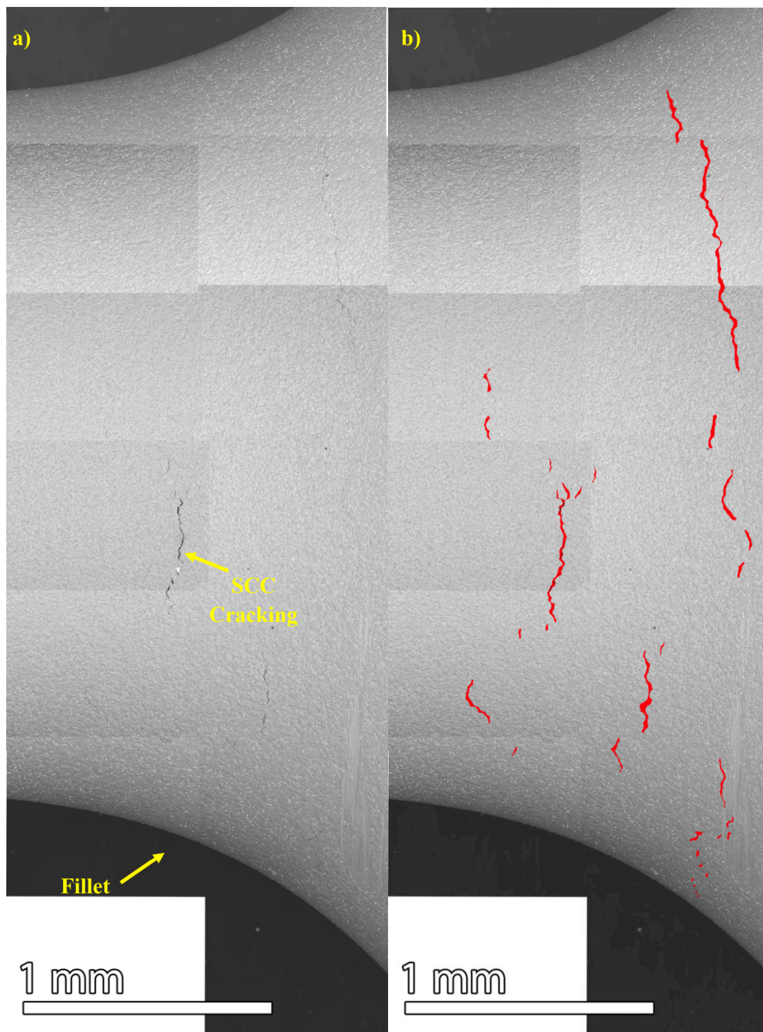
Figure 29. SEM (BSE) image of the alloy 600 tensile initiation specimen IN003 (rotated 120° from Figure 28) that exhibits cracking near the fillet. Image (b) is the identical image but cracks have been colored red as guide to the eye. SCC cracks were observed with a circumferential length as long as ~1 mm.
