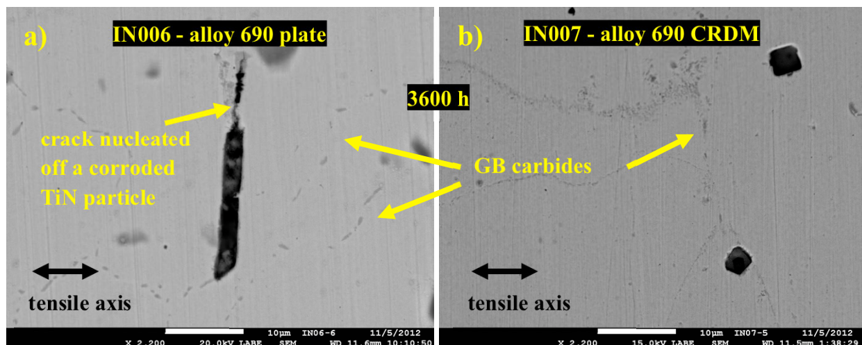
Figure 78. SEM-BSE images of the 26%CR plate and 31%CR CRDM specimens revealing grain boundary carbides and corroded TiN particles. Cracks nucleated from the ends of corroded TiN stringers were observed in the plate material while no cracking was observed in the CRDM material.
