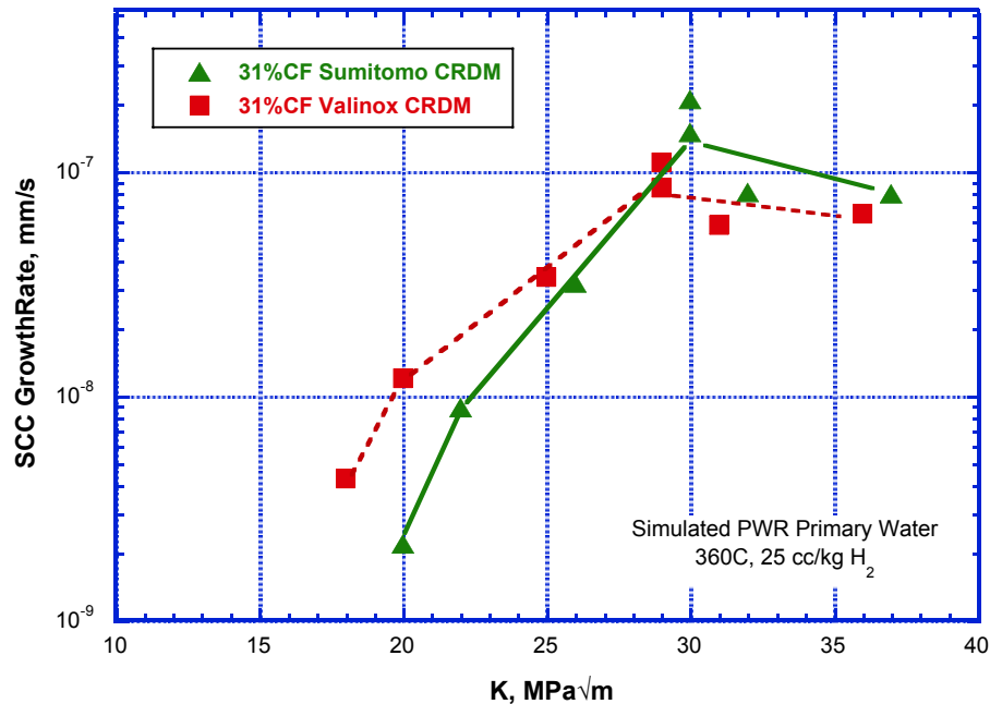
Figure 145. Crack growth rate as a function of K for the 31%CF alloy 690 CRDM materials in 360°C PWR primary water.
