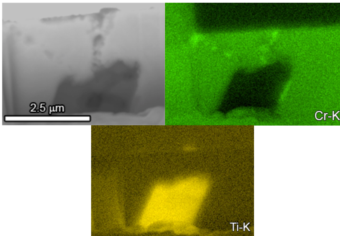
Figure 99. Near-surface grain boundary microstructure from a FIB trench in the IN007 specimen after 9144 h. Corrosion of the grain boundary is observed extending from the TiN inclusion.
