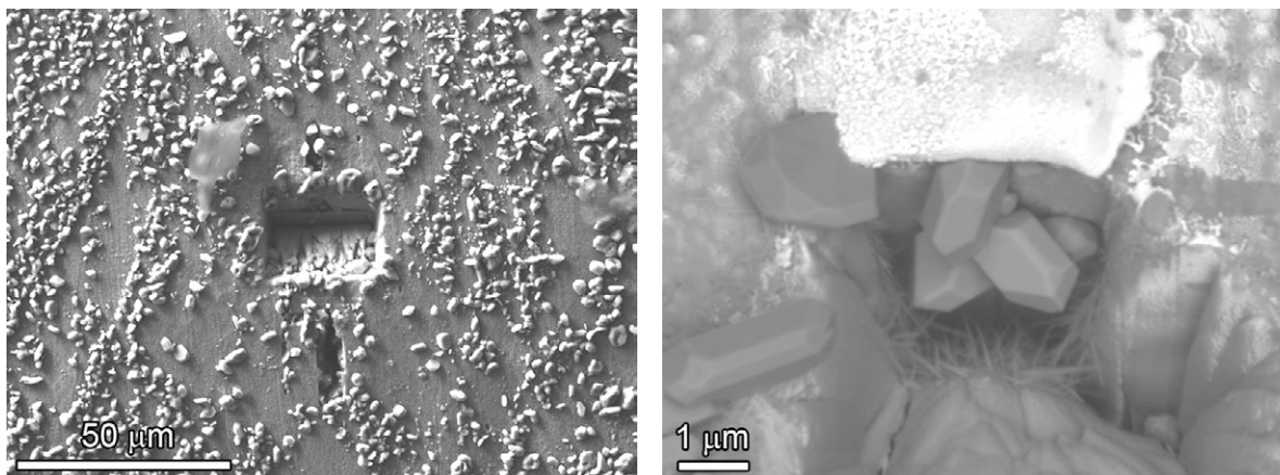
Figure 12. SEM (SE and BSE) images of an alloy 690 initiation sample that had been FIB milled and then subsequently exposed. No apparent enhanced cracking emanated from these trenches (which could be on the order of tens of micrometers). In certain cases, surface spinels nucleated in the trench.
