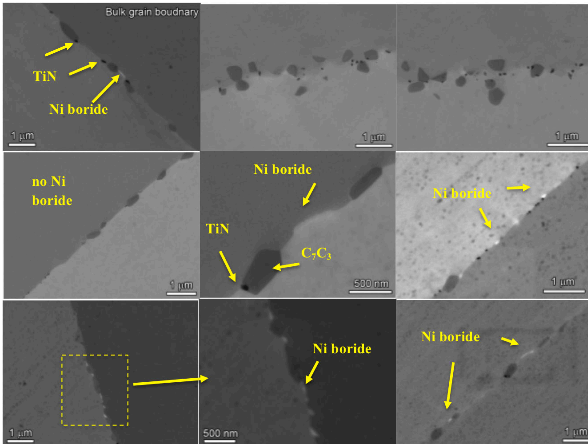
Figure 16. SEM (BSE) images illustrating the general microstructures in the mill-annealed alloy 600 CRDM heat M3935 material at higher magnification illustrating the distribution of \text{Cr}_7\text{C}_3 , TiN and Ni borides on the grain boundaries.
