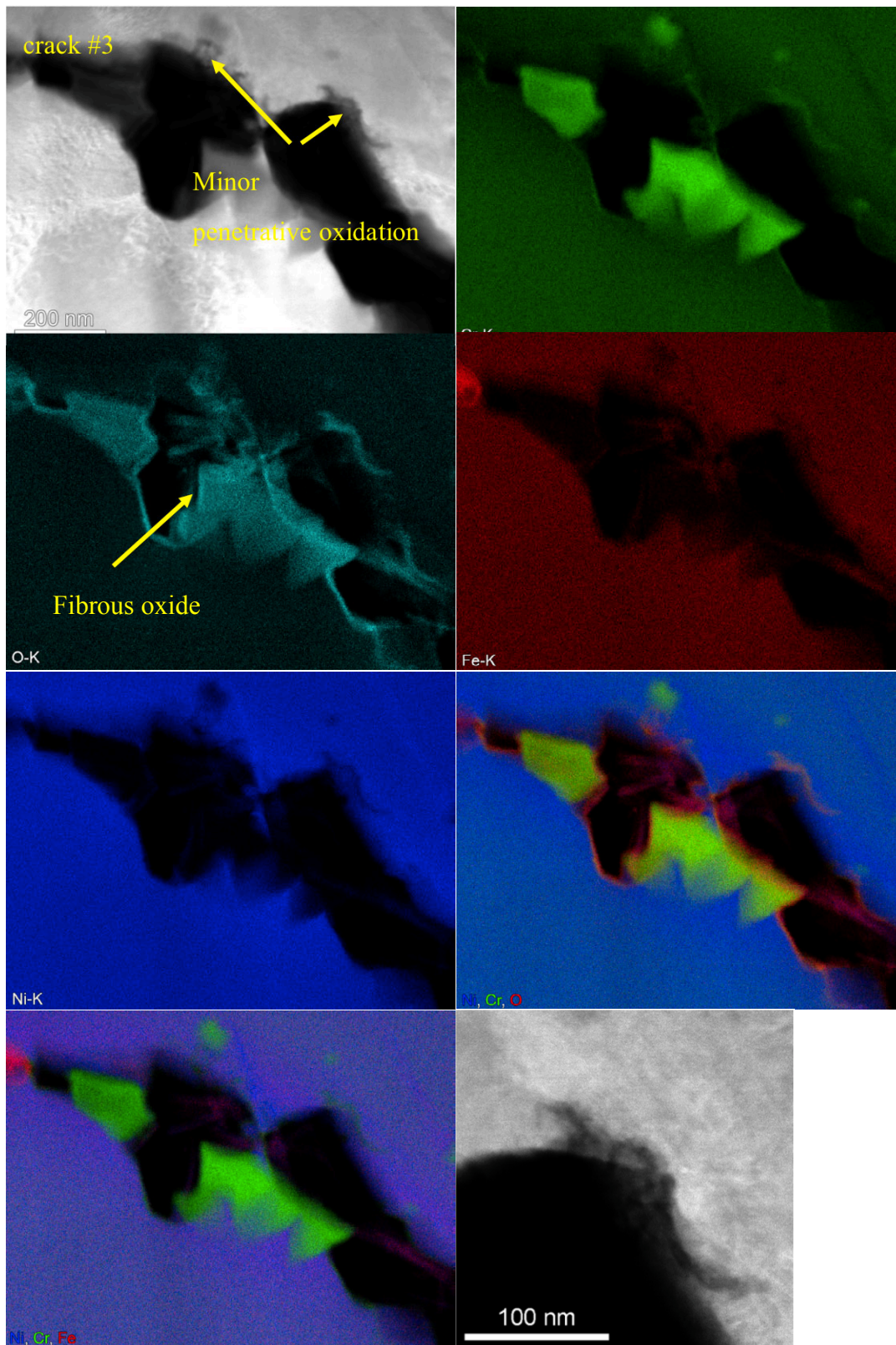
Figure 115. TEM Angular DF and EDS elemental maps of crack tip #3 (see Figure 105).
