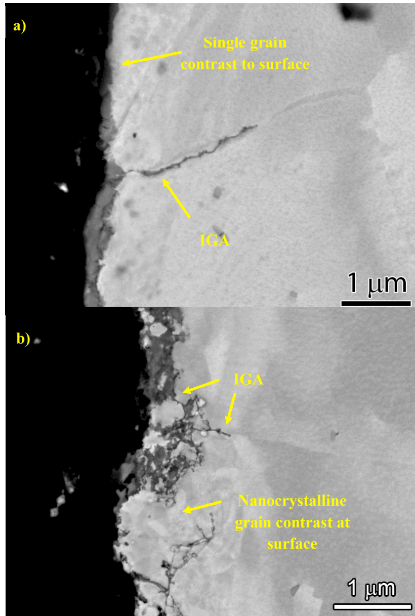
Figure 36. SEM-BSE images of cross-sections from the alloy 600 initiation specimens with surfaces of 1 μm diamond (IN003) and 1200 grit SiC (IN002) after exposure to PWR primary water.
