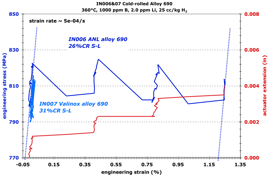
Figure 83. Tensile straining performed on the alloy 690 materials. The 26%CR plate (IN006) underwent \sim 1.2\% plastic strain while the 31%CR CRDM (IN007) did not yield.
