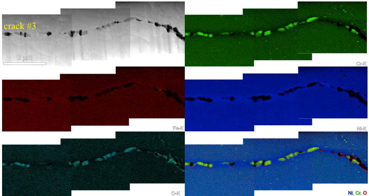
Figure 114. TEM Angular DF and EDS elemental map montages of crack #3 (see Figure 105).
