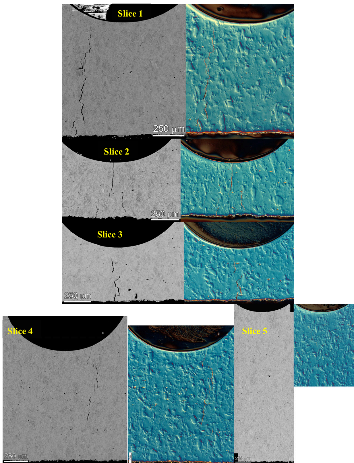
Figure 134. SEM-BSE and optical micrographs of five cross-section slices in C673.
