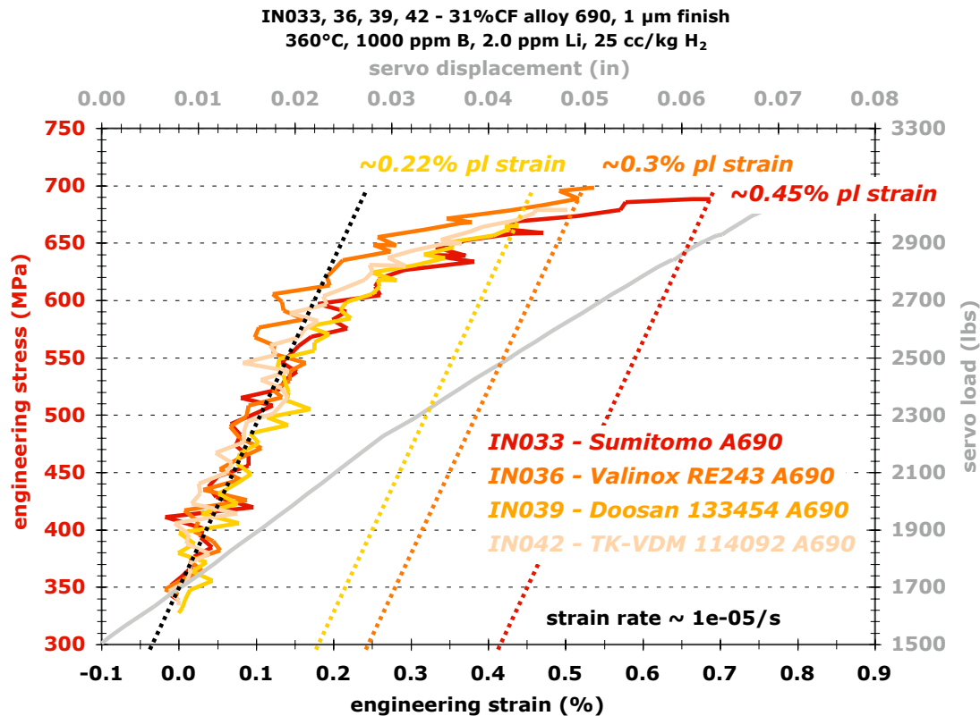
Figure 9. Typical stress versus strain response when loading up multiple specimens for the start of an SCC initiation test. The loading process is typically arranged to take \sim 1 hour.
