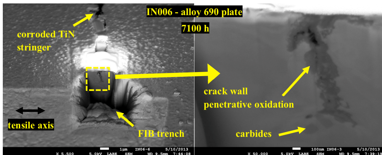
Figure 90. Strain driven IG crack in the 26%CR plate specimen as viewed in cross section using the FIB trench process. Cracking was limited to a depth of \sim 1 \mu\text{m} .
