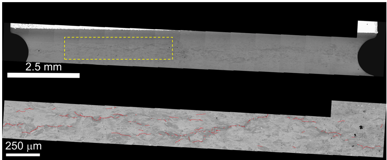
Figure 128. SEM-BSE montage of a) the entire notch of C673 (31%CF Sumitomo CRDM) and b) a selected higher magnification montage of the dashed yellow box in a) showing cracks.
