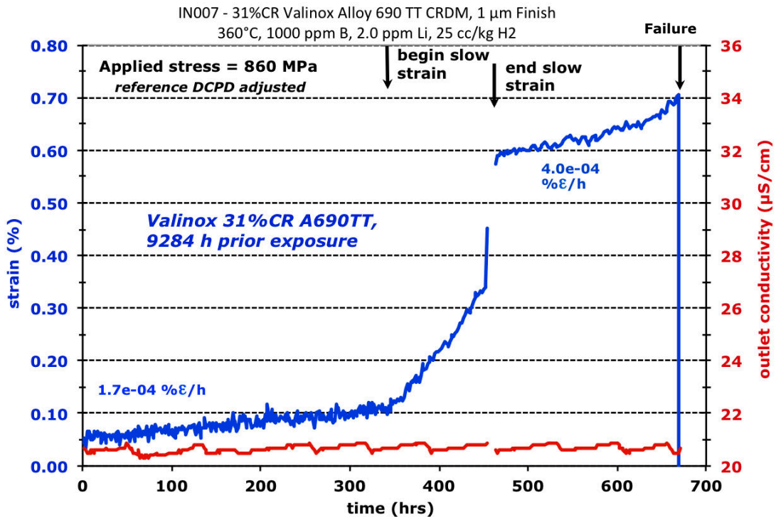
Figure 100. DCPD-based strain response of the 31%CR alloy 690 CRDM specimen IN007 after restart at the yield stress (860 MPa).
