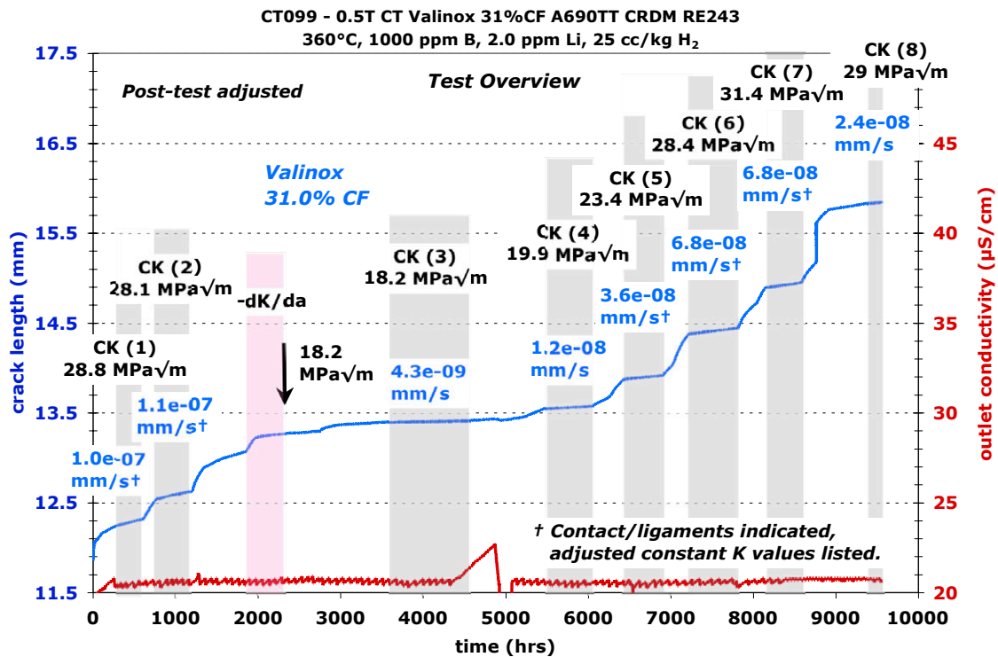
Figure 143. Overview of the entire SCC test on the 31%CF S-L/S-T Valinox CRDM RE243 specimen CT099 showing crack growth rate at each of the different stress intensity levels.
