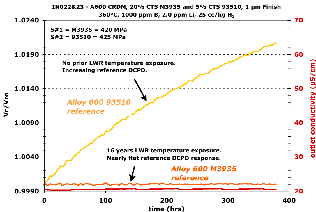
Figure 46. DCPD response for the reference locations in specimens IN022 and IN023.
