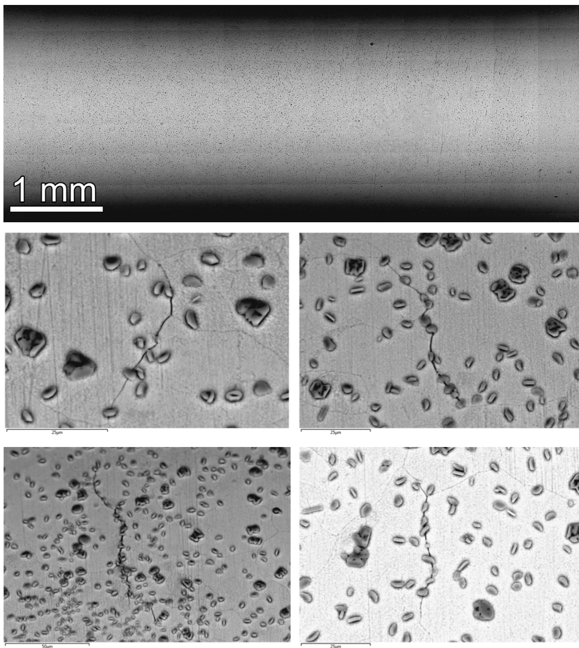
Figure 51. SEM-BSE examples of small surface cracks on the IN023 specimen gauge after a combined test time of ~1870 hours. The top image shows rotation 1 at low magnification illustrating that no obvious SCC cracks are present. The bottom four images provide examples of typical small cracks that were extremely tight and reached lengths approaching ~100 \mu\text{m} in isolated locations.
