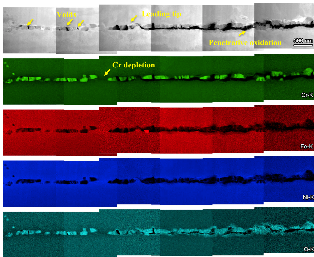
Figure 111. TEM Angular DF and EDS elemental map montages of crack #1 (see Figure 105).
