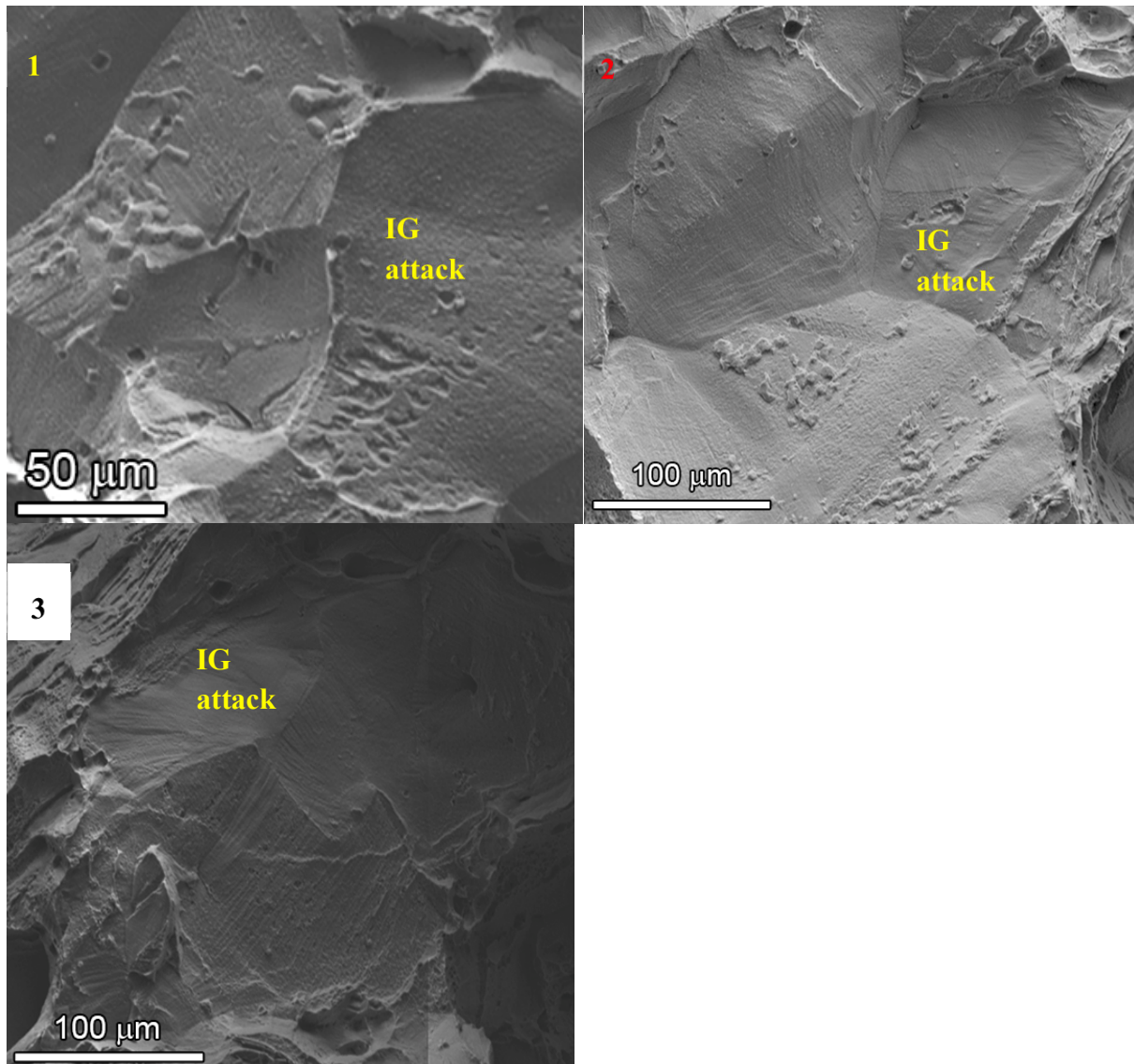
Figure 102. SEM-SE images of IG cracking of various regions denoted in Figure 101.
