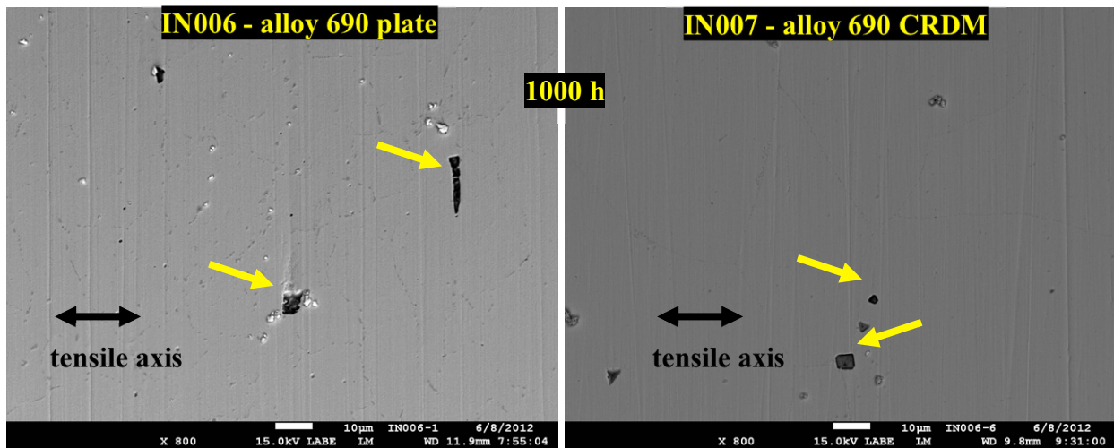
Figure 76. SEM-BSE images of the 26%CR plate and 31%CR CRDM specimen gauge sections, respectively, revealing small grain boundary carbides and larger matrix TiN particles (identified by arrows) that have partially corroded.
