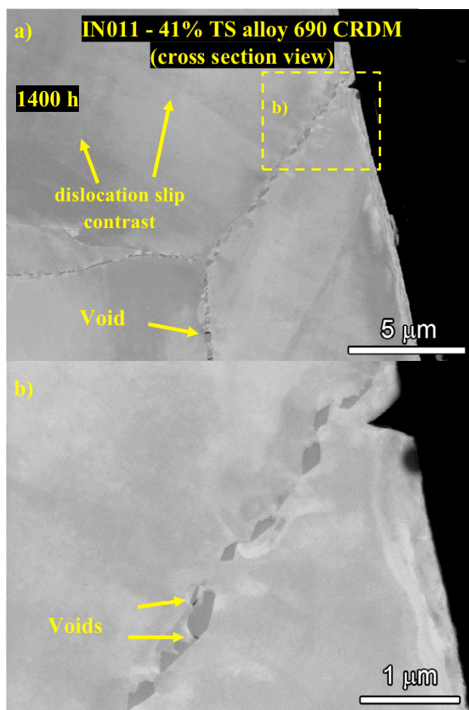
Figure 119. These cross section images illustrate deformation seen close to a grain boundary intersecting the surface of the specimen. The V-shaped feature is likely a result of a slip band. Void formation adjacent to carbides as shown here was seen throughout the necked region, including in the bulk away from the surface. No evidence for localized grain boundary corrosion or oxidation is seen.
