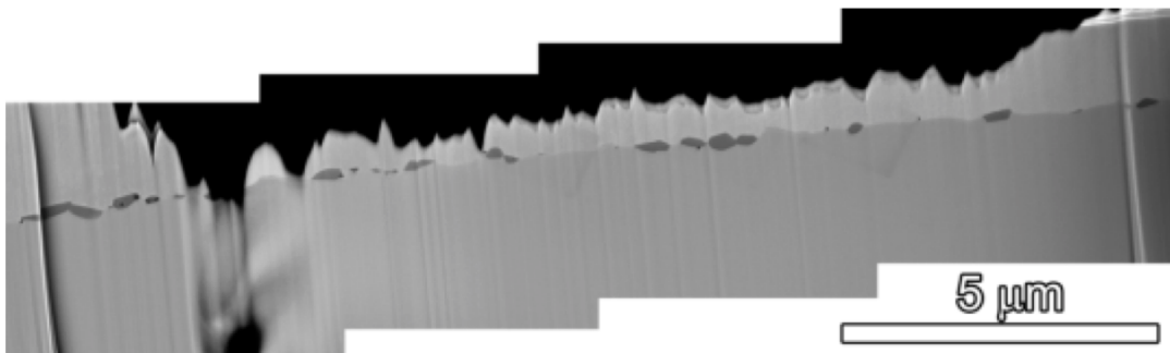
Figure 19. SEM (BSE) montage of FIB machined TEM plate sample containing a grain boundary from alloy 600 M3935. In this region, there does not appear to be any Ni boride particles.
