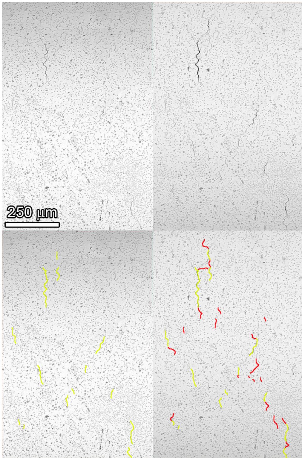
Figure 55. SEM-BSE images of IN023 Rotation #2 illustrating the sample at 1713 hours (left columns) and 2591 hours (right columns). The bottom two figures highlight the cracks in yellow present at 1713 hours and new cracks in red present at 2591 hours (red).
