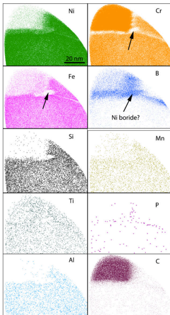
Figure 22. Atom maps from an IG Cr carbide and surrounding grain boundary in Davis Besse CRDM heat M3935. Very strong Cr depletion and B enrichment are apparent along the grain boundary and metal/carbide matrix. Particularly strong localized B enrichment and Cr depletion is suggestive of possible Ni boride precipitations (arrowed).
