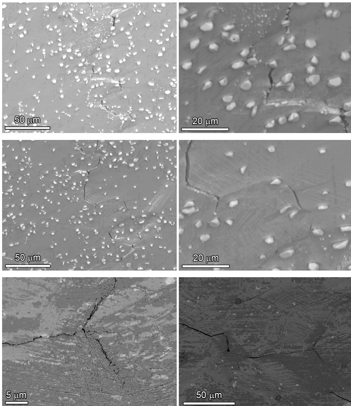
Figure 132. Higher magnification SEM images showing cracks on the notch of 31%CF Sumitomo CRDM specimen c673.
