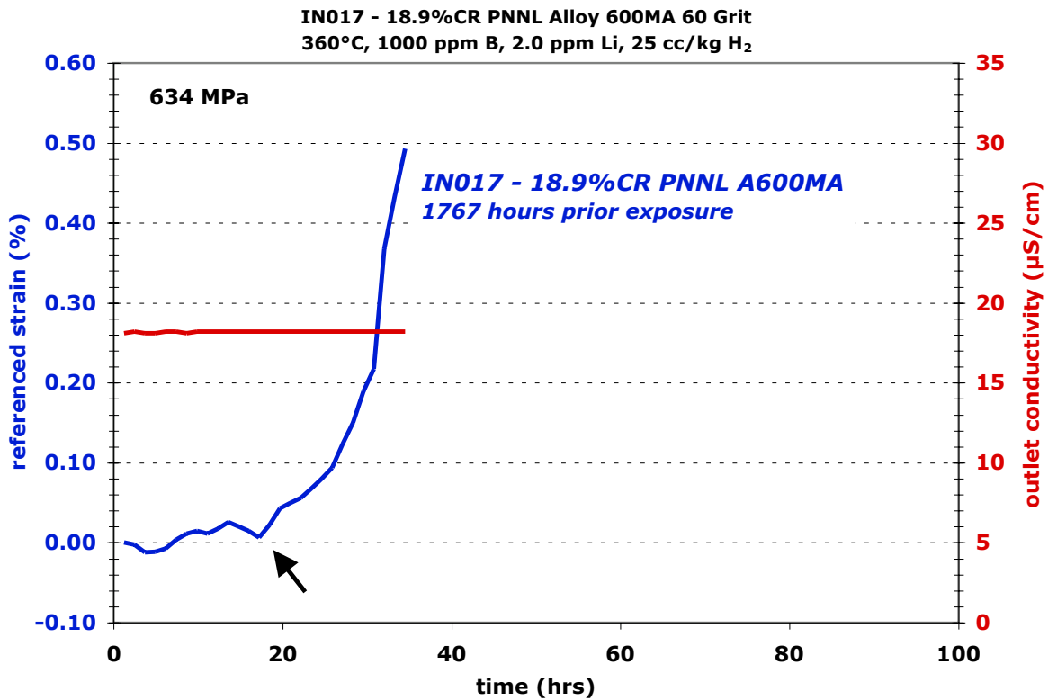
Figure 41. SCC initiation plot for 19%CR alloy 600 specimen IN017 that had a 60 grit finish.
