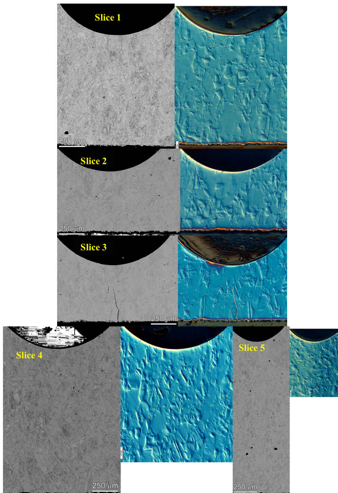
Figure 133. SEM (BSE) and optical micrographs of five slices in C672.
