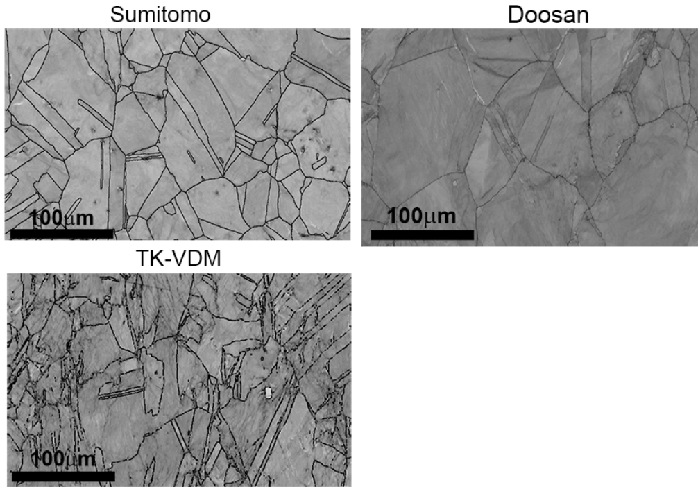
Figure 68. EBSD pattern quality images showing the grain size and microstructure of the Sumitomo, Doosan and TK-VDM materials.
