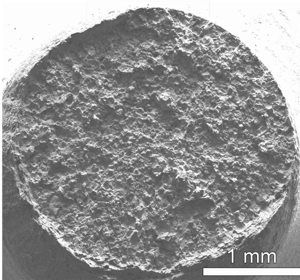
Figure 39. SEM-SE image showing IG fracture surface for 19%CR alloy 600 specimen IN016 after testing in PWR primary water.
