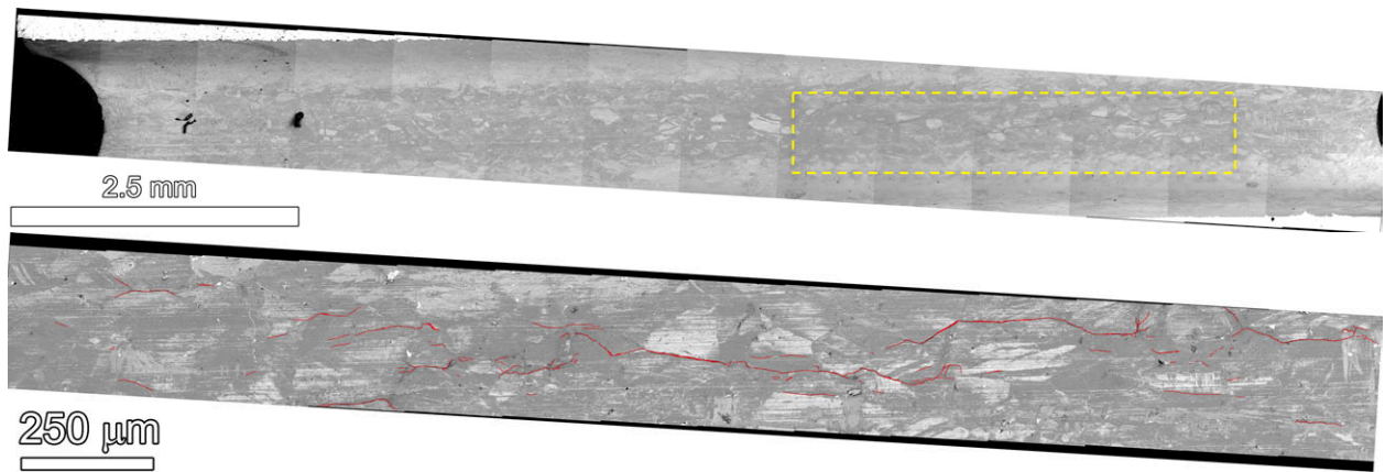
Figure 127. SEM-BSE montage of a) the entire notch of C672 (31%CF Valinox CRDM) and b) a selected higher magnification montage of the dashed yellow box in a) showing cracks.
