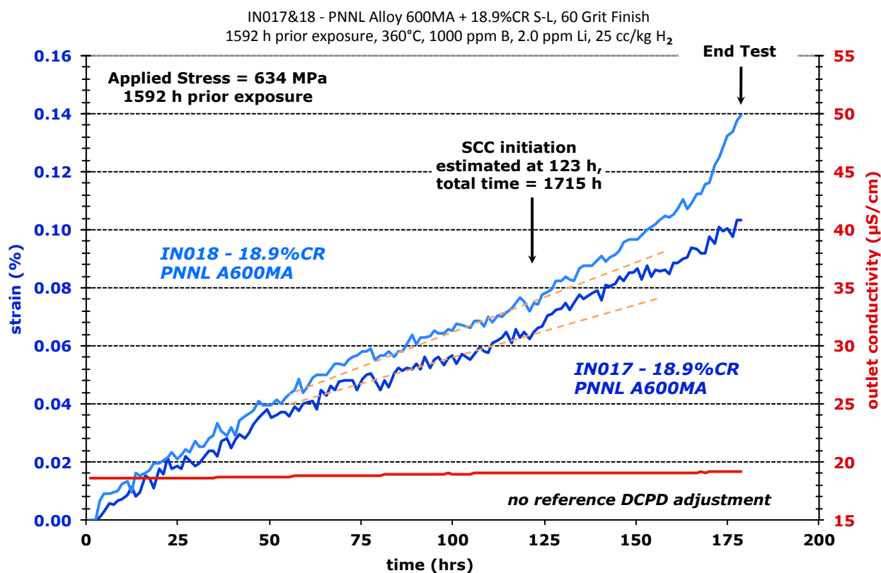
Figure 40. SCC initiation test plot for the continuing test on 19%CR alloy 600 specimens IN017 and IN018 in 360°C PWR primary water.
