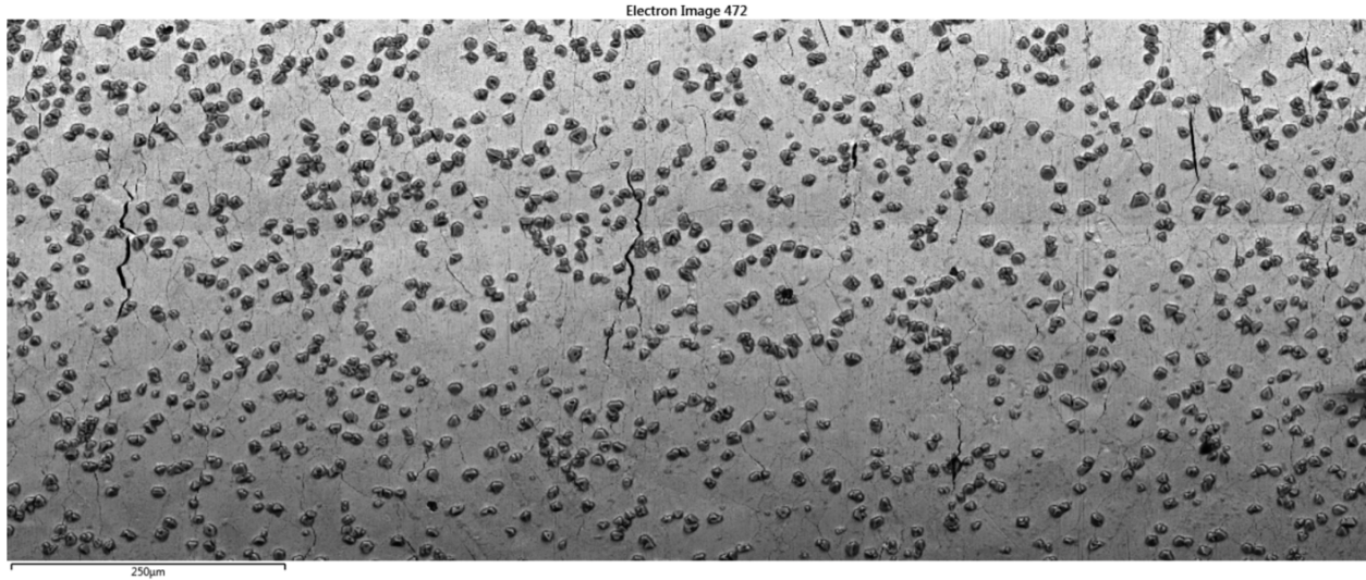
Figure 61. SEM-BES image showing examples of small surface cracks in the as-received alloy 600 plate IN013 specimen after testing in 360°C PWR primary water for a total of 3392 hours.
