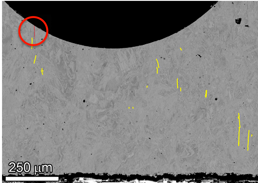
Figure 140. SEM-BSE image of C672 cross-section slice #2 showing cracks identified as SCC (red) and creep (yellow).
