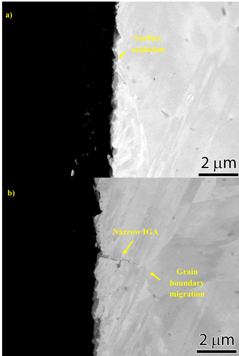
Figure 33. SEM-BSE images of a cross-section for the alloy 600 tensile initiation specimen IN003 illustrating representative TG (surface oxidation) and IG corrosion in the gauge section.
