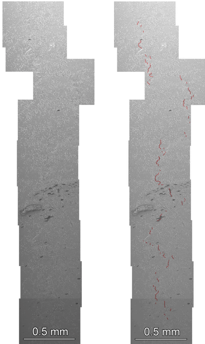
Figure 131. SEM-SE image of a portion of the 31%CF Sumitomo CRDM specimen c673 notch showing several nucleated cracks (highlighted by red marker in right image).
