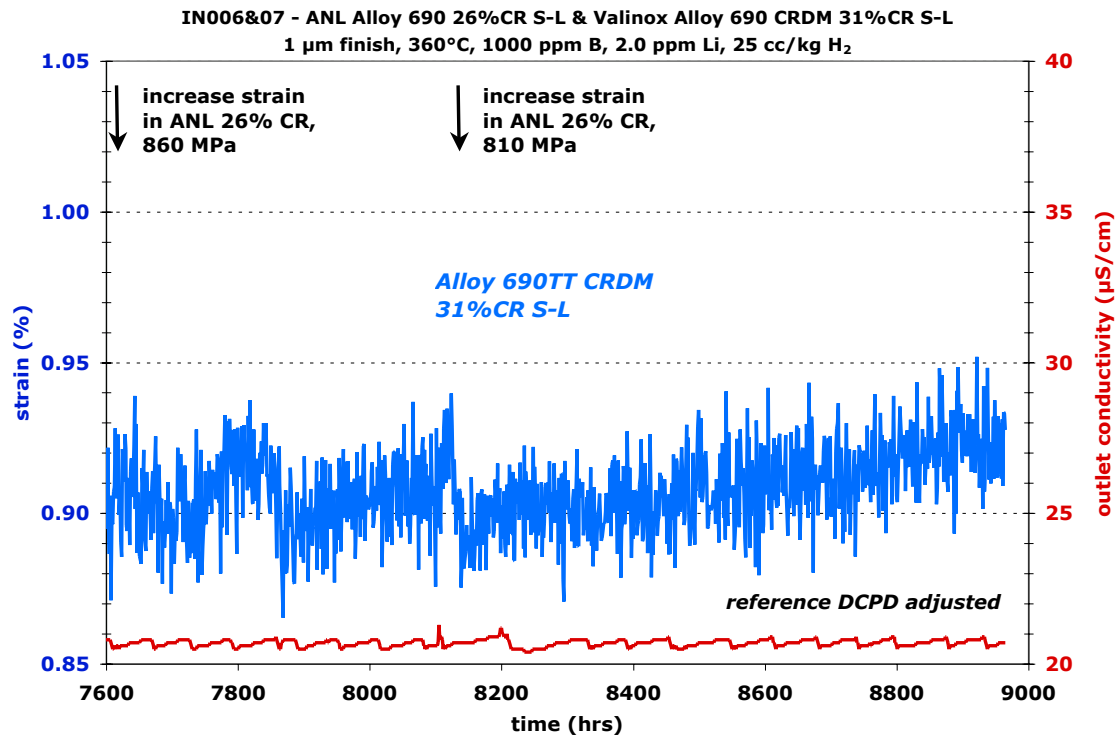
Figure 94. DCPD-based strain response of the 31%CR alloy 690 CRDM specimen IN007 from 7600 to 8950 hours.
