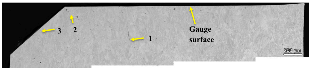
Figure 105. SEM-BSE cross-section image of the IN007 gauge section depicted in Figure 104. Cross-section is flipped and rotated 90 degrees.
