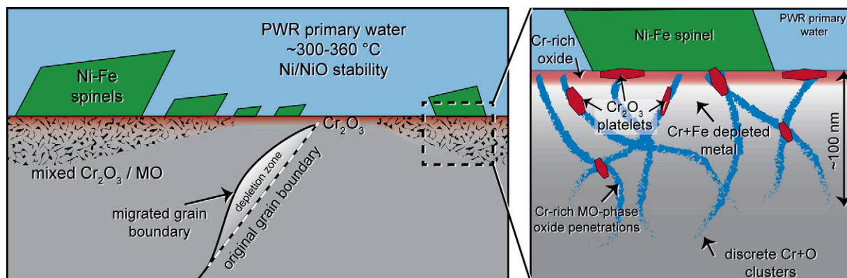
Figure 70. Enhanced Cr diffusion from grain boundaries allows protective \text{Cr}_2\text{O}_3 film ( \sim 0.5\text{-}1\ \mu\text{m} wide) to form over grain boundary. Non-protective thin film of \text{Cr}_2\text{O}_3 and Cr rich MO forms over bulk grains due to slower Cr bulk diffusion. Oxygen diffusion through non-protective film allows penetrative oxidation to occur in bulk grains. Additionally, increased Cr diffusion continues along grain boundary to edge of protective film and forms continuous \text{Cr}_2\text{O}_3 layer between bulk and penetrative oxidation.
