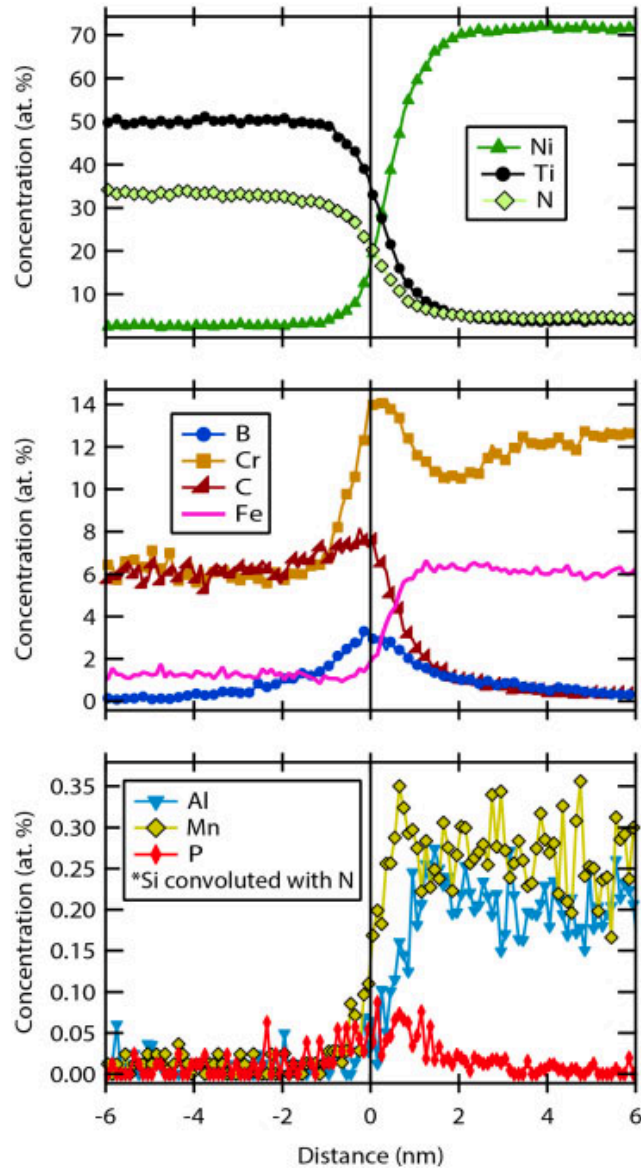
Figure 21. Proximity histogram across the Ti carbo-nitride/metal matrix interface in M3935. The precipitate contains a moderate concentration of Cr that is also strong segregated to the interface. B is strongly segregated ( \sim 3.3 at%) along with a small enrichment of P ( \sim 0.06 at%).
