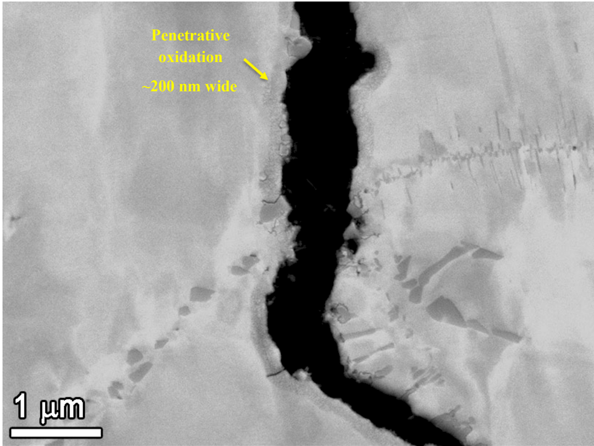
Figure 107. SEM-BSE image showing penetrative oxidation in the yellow box in Figure 106.
