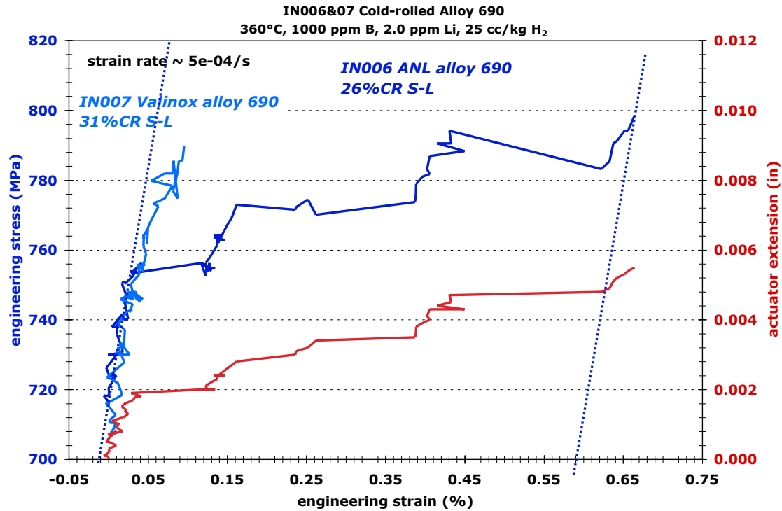
Figure 81. Tensile straining performed on the alloy 690 materials at ~5300 hours. The 26%CR plate material (IN006) underwent approximately 0.6% plastic strain while the 31%CR CRDM material (IN007) did not yield.
