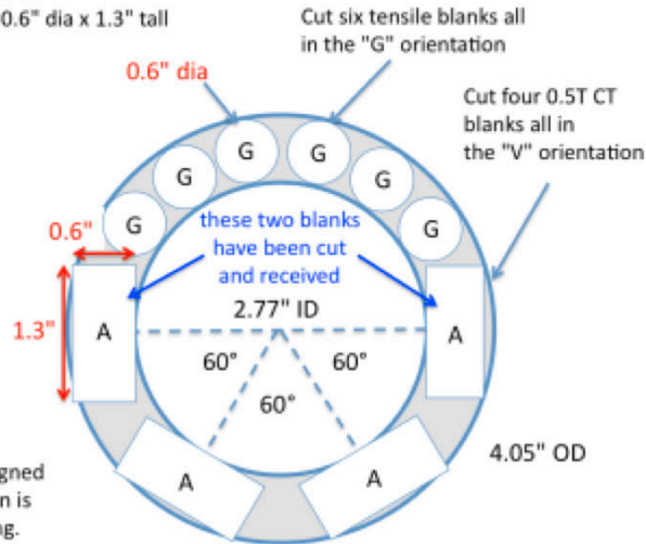
Figure 14. Sectioning plan for 0.5T CT specimens and tensile specimen blanks for a 1.4 inch tall slice of nozzle #1 of the original Davis Besse RPV head.
