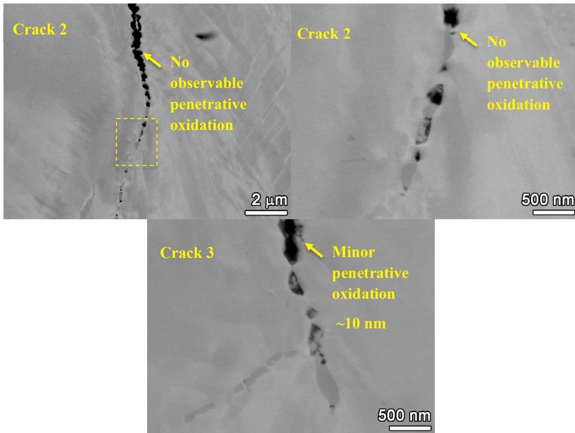
Figure 110. SEM-BSE images of crack #2 and crack #3 (see Figure 105), both of which were identified as creep cracks. No significant penetrative oxidation was observed.
