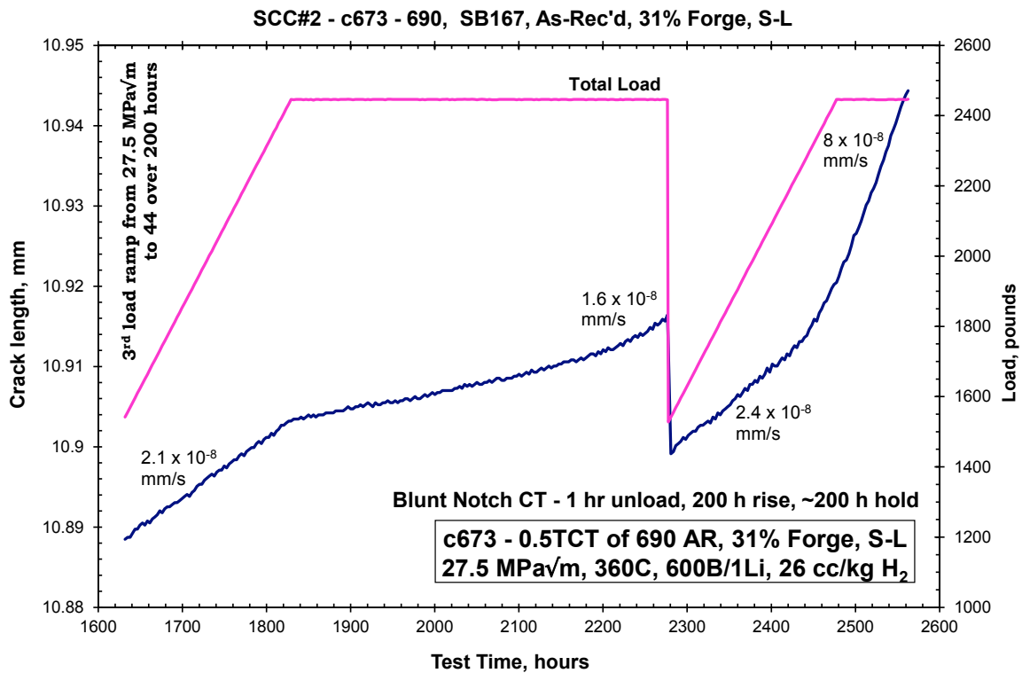
Figure 126. Crack length versus time response for the 31%CF Sumitomo CRDM specimen c673 blunt notch specimen.
