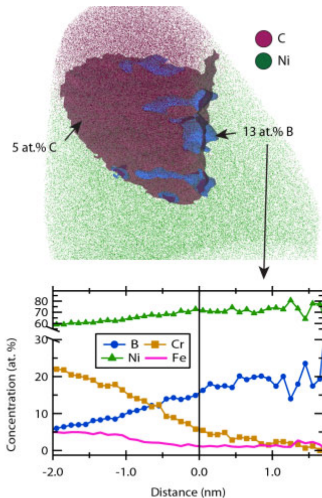
Figure 24. APT reconstruction of the IG carbide in the Davis Besse CRDM heat M3935. Isoconcentration surfaces at 5 at% C (maroon) and 13 at% B (blue) outline the Cr carbide and possible Ni boride, respectively. A proximity histogram (bottom) from around the 13 at% B isoconcentration surface confirms the coincident enrichment of Ni and B (up to 20 at%) that is suggestive of an interfacial Ni boride phase.
