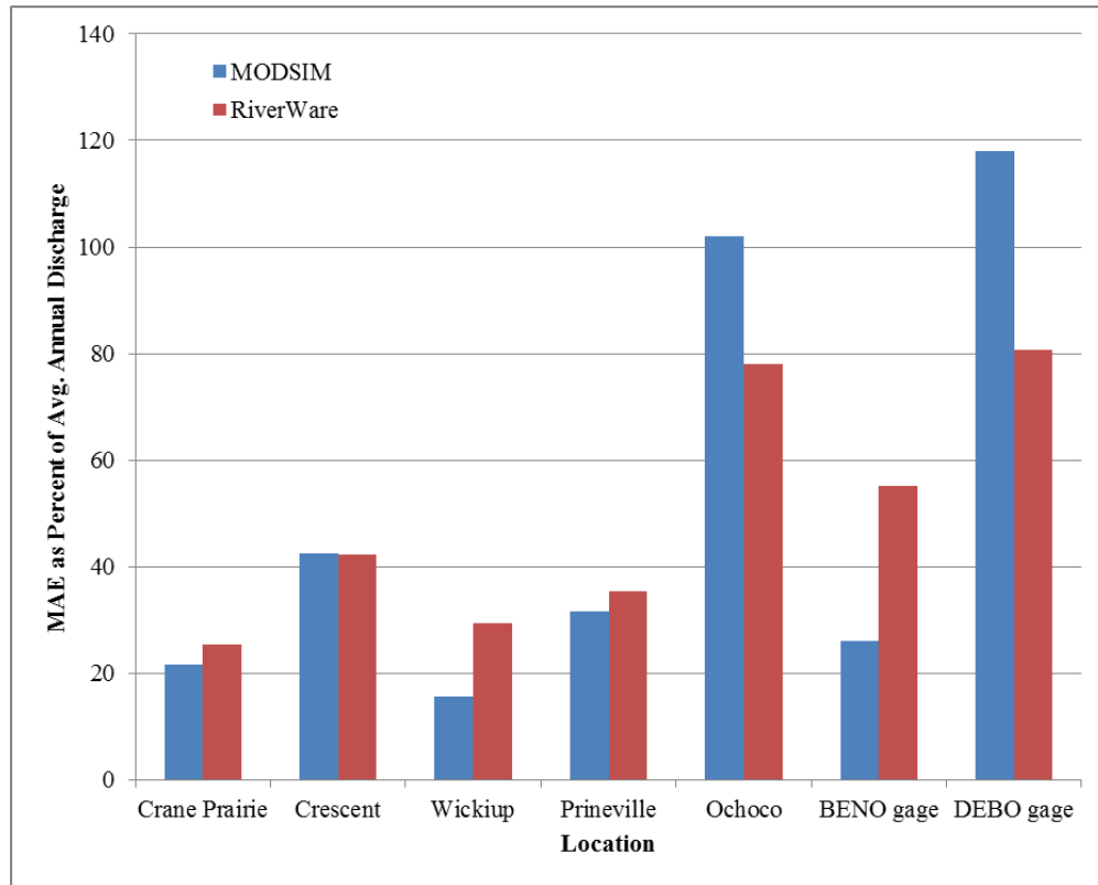
Figure 7.2. Mean absolute error (MAE) as a percent of average annual discharge.
