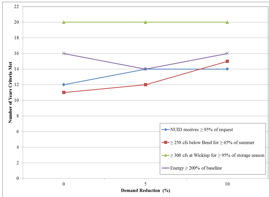
Figure 7.9. Number of years that target levels for value-based metrics were met based on simulated reductions in irrigation demand and a 250-cfs minimum flow below Wickiup Dam.
