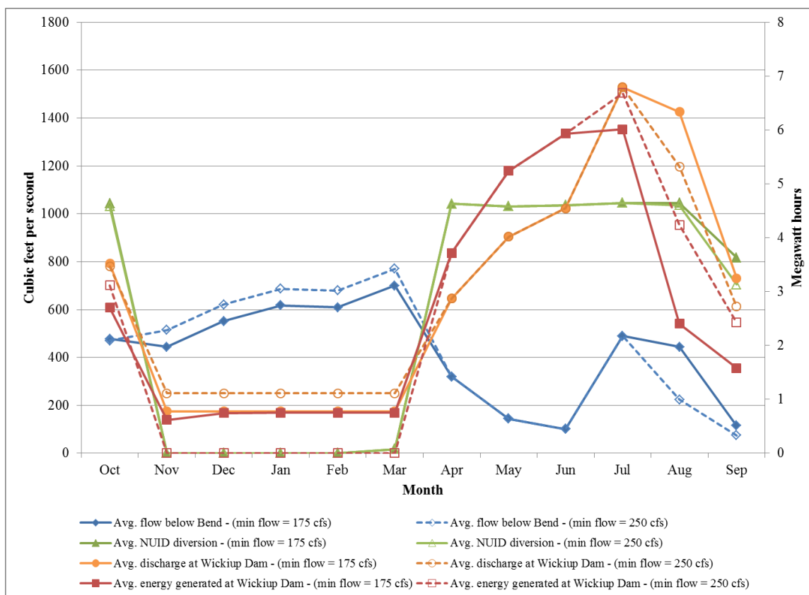
Figure 7.8. Monthly average flow below Bend and monthly average NUID diversion at the 175- and 250-cfs minimum flow trial levels.
