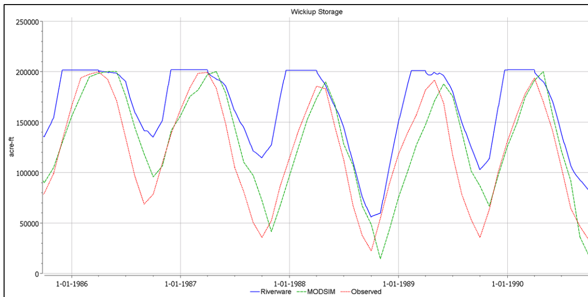
Figure 7.3. Observed and modeled storage at Wickiup Dam from 1985 to 1990.
