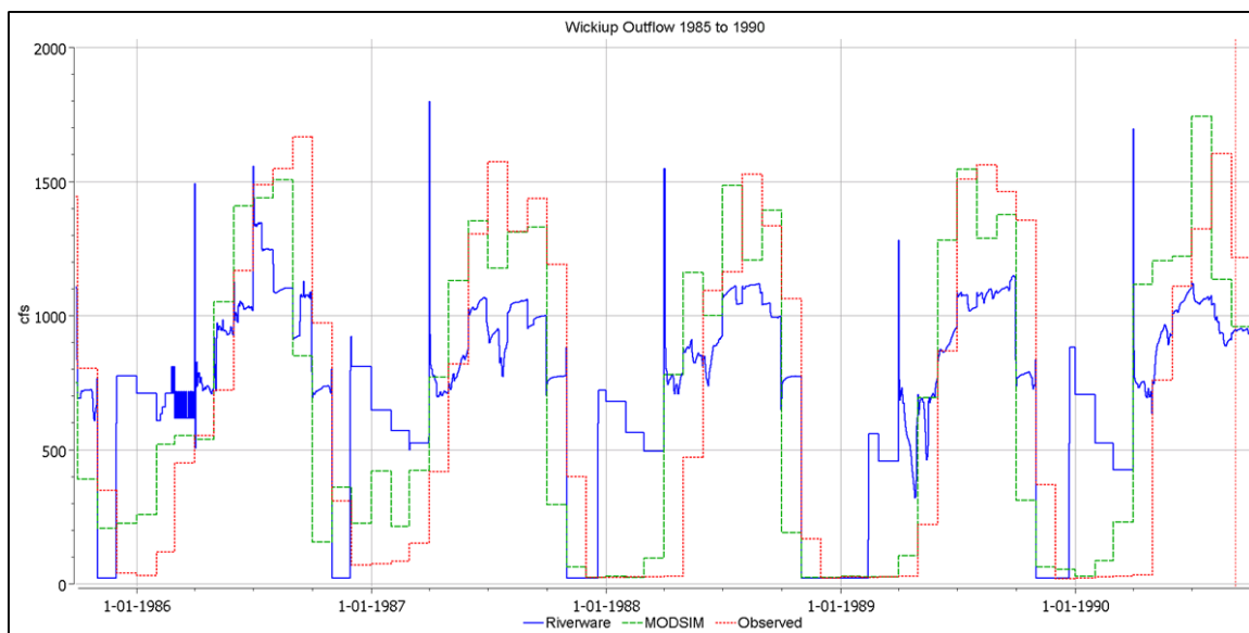
Figure 7.4. Observed and modeled discharge at Wickiup Dam from 1985 to 1990.
