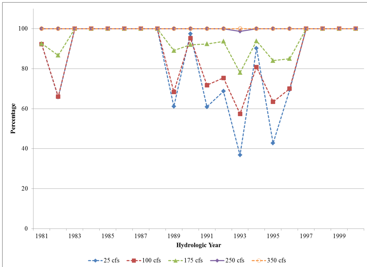
Figure 7.5. Percent of storage season flow is \geq 300 cfs below Wickiup Dam based on minimum flow trial levels with no demand reduction.
