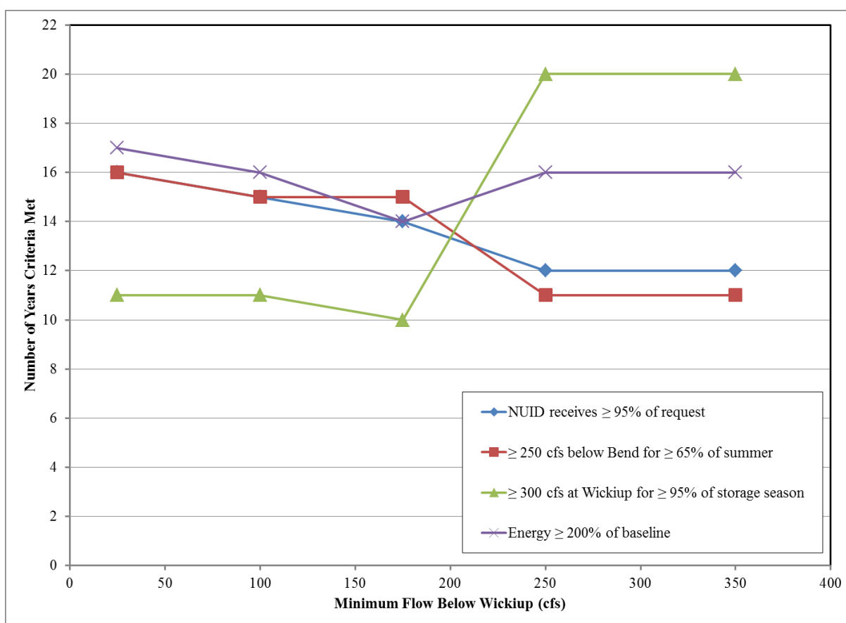
Figure 7.6. Number of years that meet example target levels for Deschutes River Scenario value-based metrics based on minimum flow trial levels.
