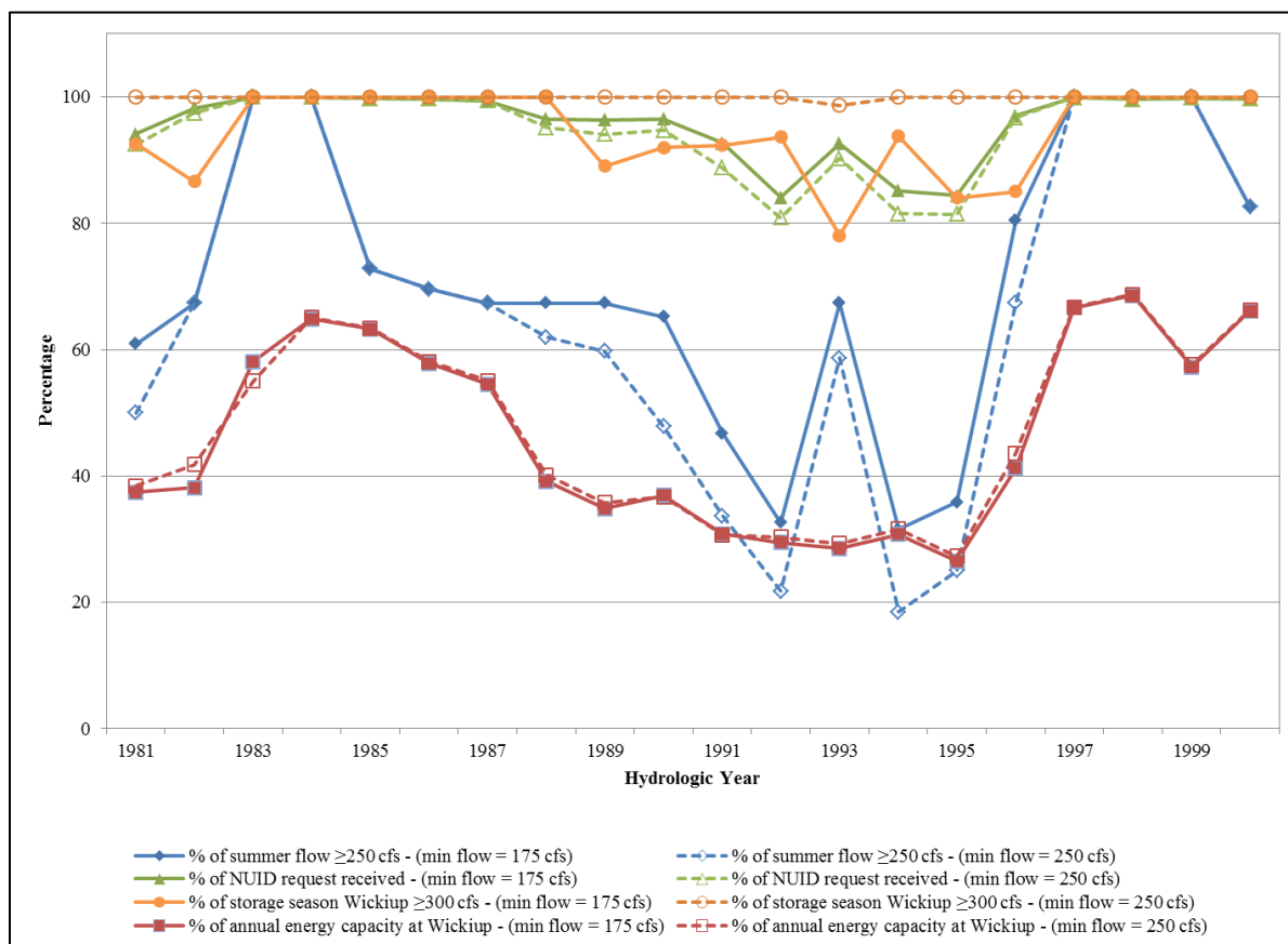
Figure 7.7. Annual trends for value-based metrics describing summer flows below Bend, NUID annual diversions, storage season flows below Wickiup Dam, and power generation at Wickiup Dam.
