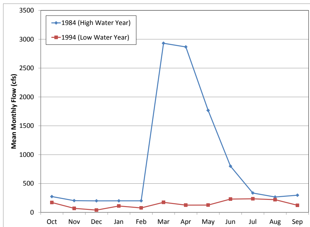
Figure 7.11. Monthly mean flows at Bowman Dam during high and low water years.
