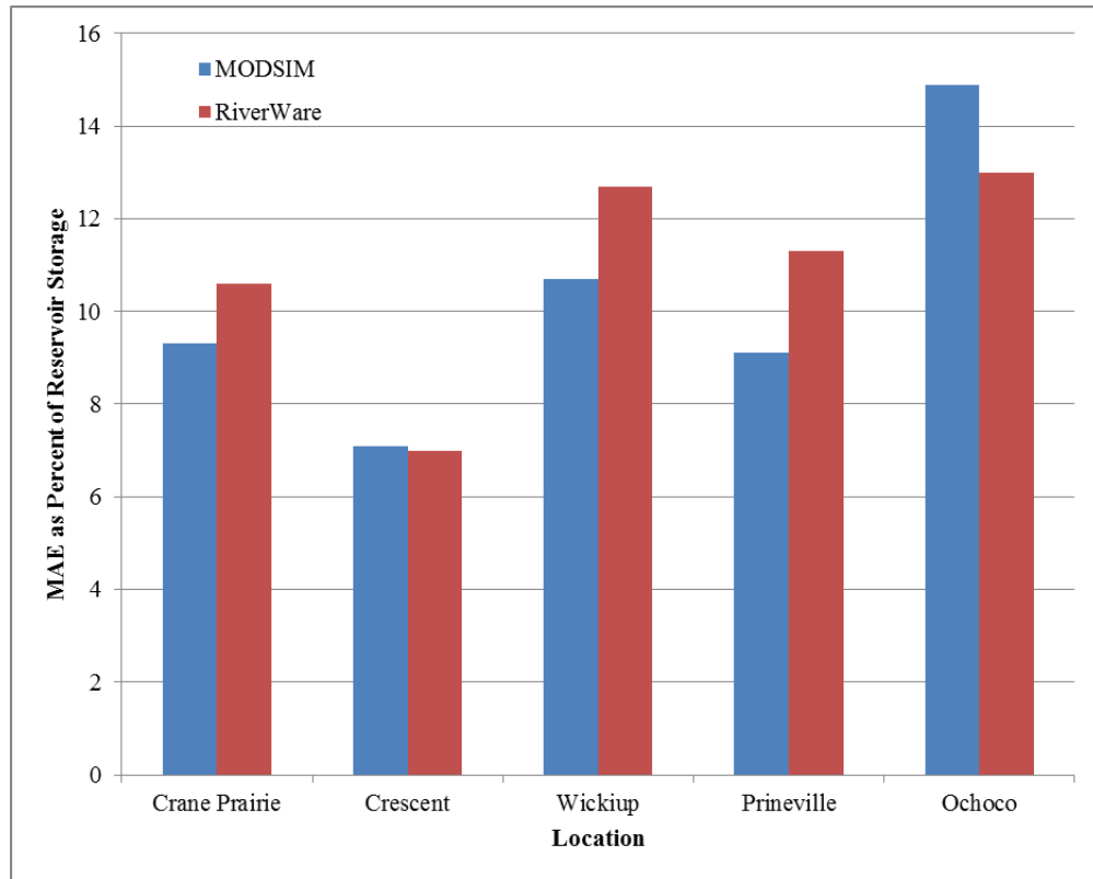
Figure 7.1. Mean absolute error (MAE) as a percent of reservoir storage.
