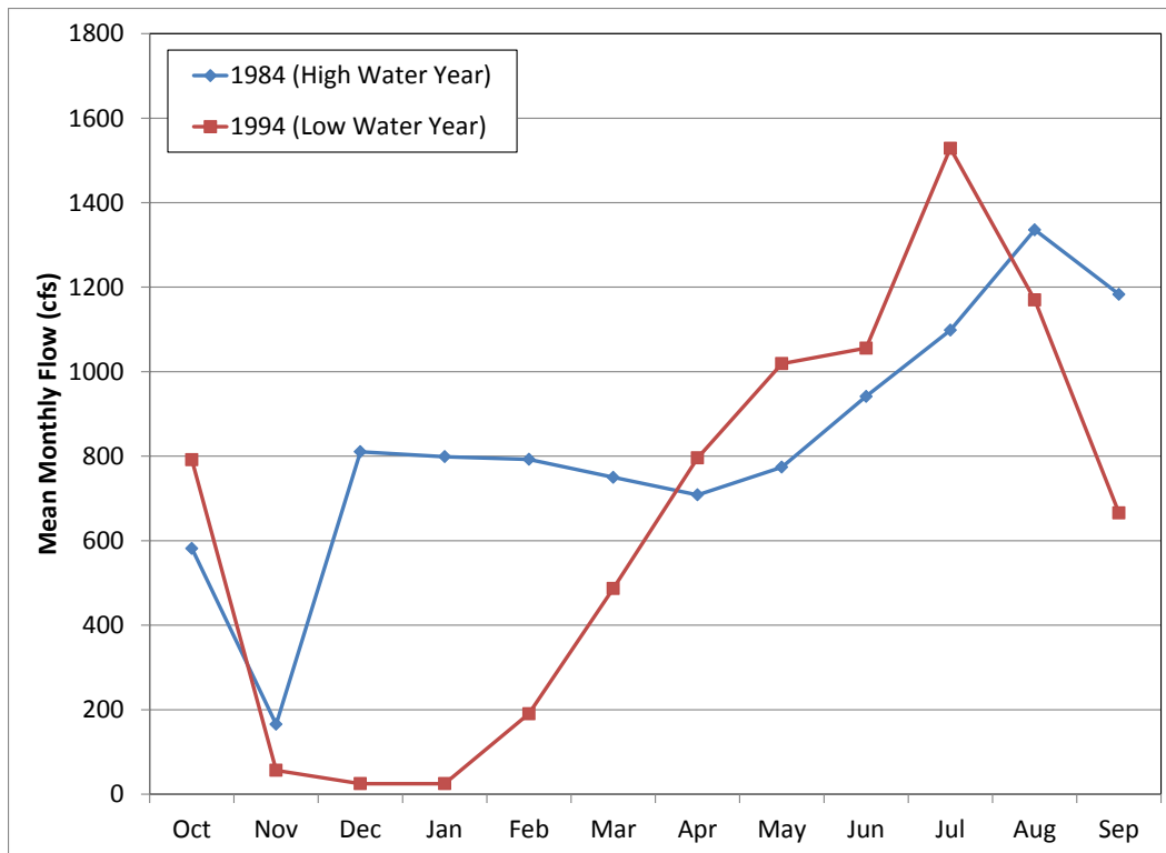
Figure 7.10. Monthly mean flows at Wickiup Dam during high and low water years.
