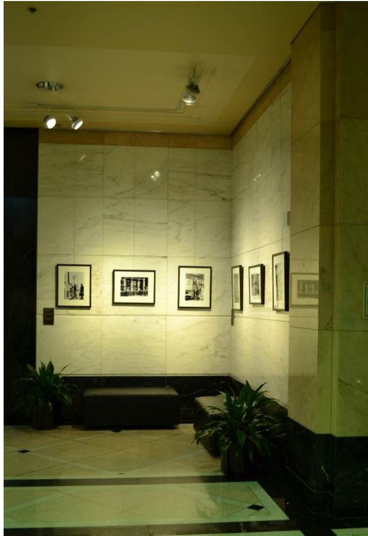
Figure 4. Lobby photos lighted with Cree LRP38 LED lamps (AFTER). Note that the beam is much more focused on the intended target. (Photo by Mike Hoffman, PNNL.)
