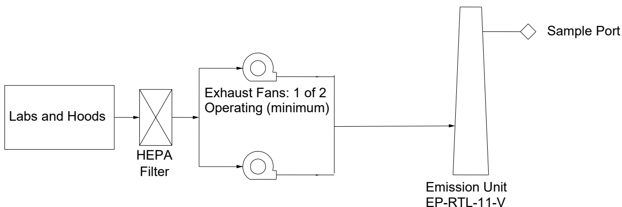
Figure F.2. RTL-11-V Effluent Pathway
