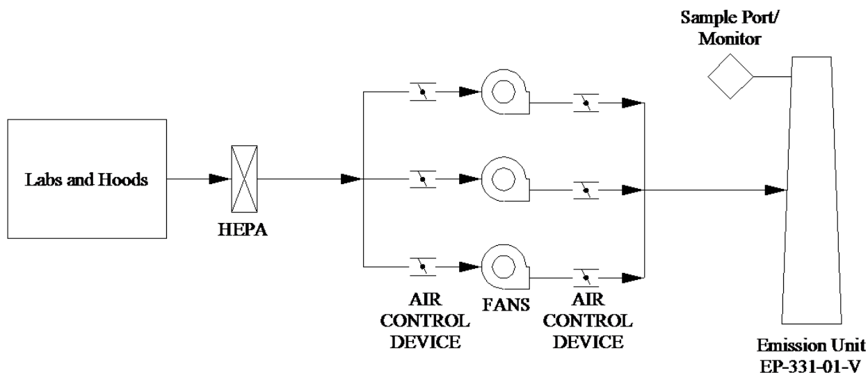
Figure D.2. 331-01-V Building Effluent Pathway
