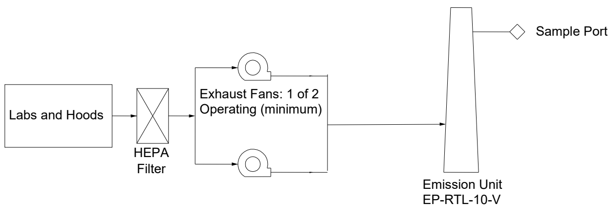
Figure F.1. RTL-10-V Effluent Pathway
