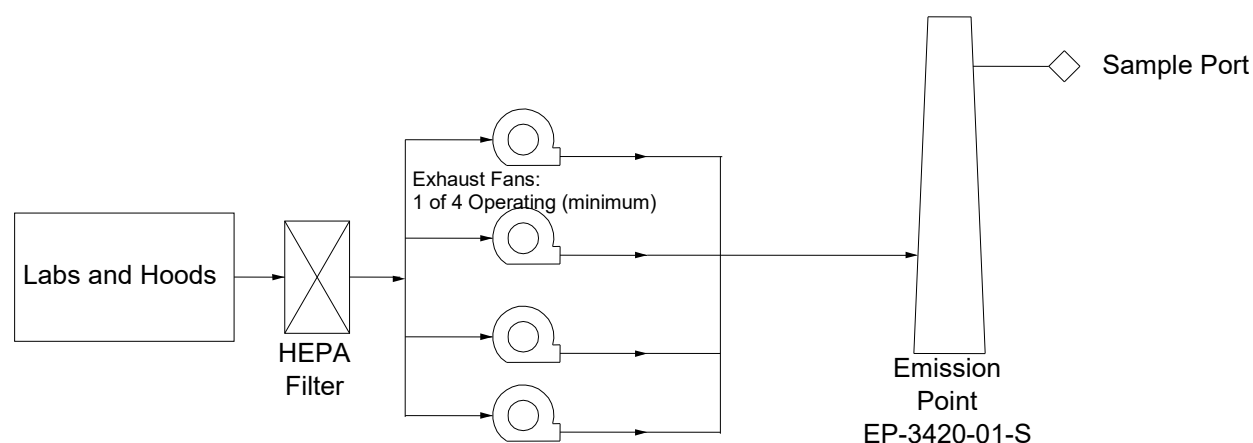
Figure D.4. 3420-01-S Building Effluent Pathway
