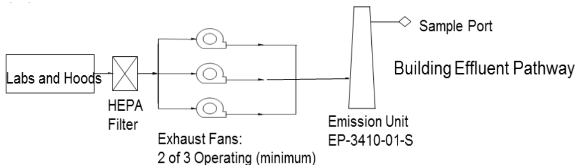
Figure D.3. 3410-01-S Effluent Pathway
