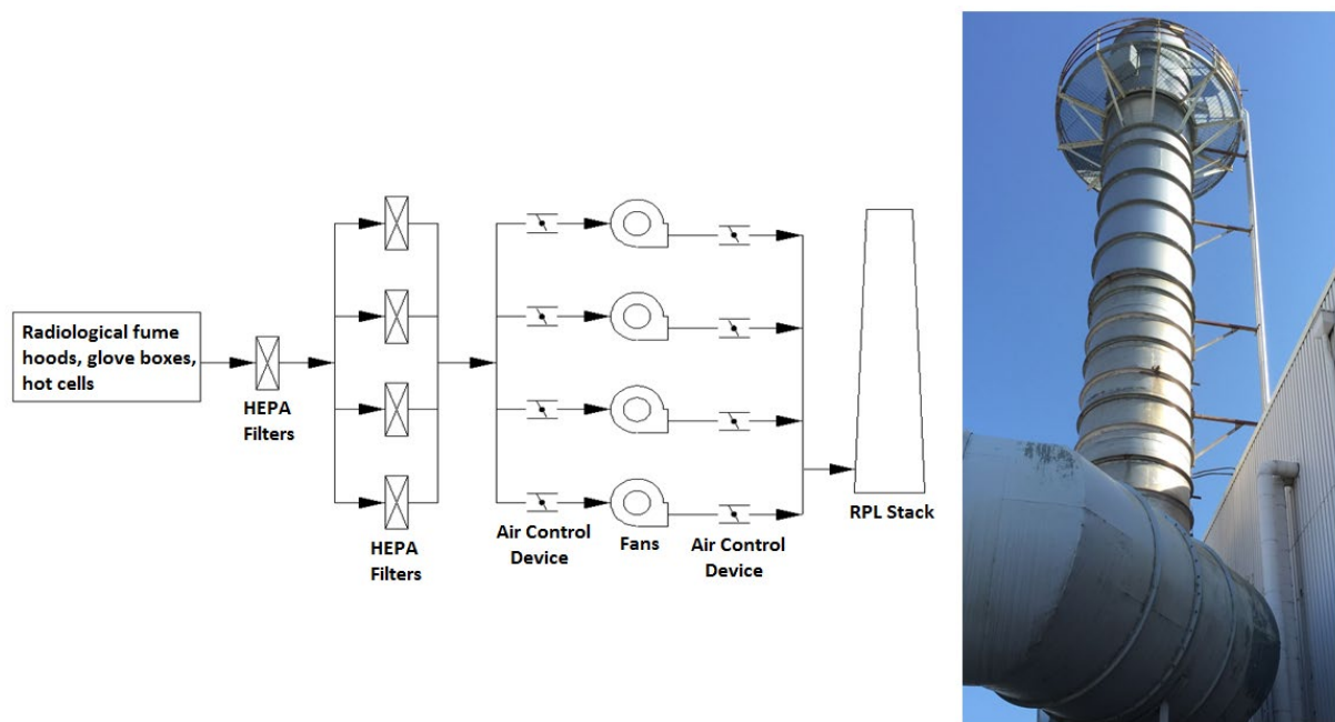
Figure D.1. 325-01-S Building Effluent Pathway
